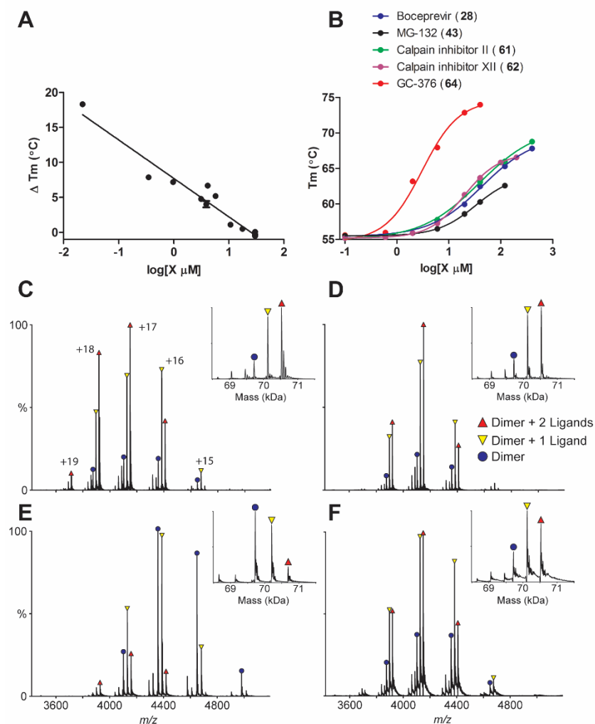
Figure 3: Binding of inhibitors to SARS-CoV-2 M pro using thermal shift binding assay and native mass spectrometry. (A) Correlation of inhibition efficacy (IC 50 ) with \Delta T_m from thermal shift binding assay. Data in Table 2 were used for the plot. The r^2 of fitting is 0.94. (B) Dose-dependent melting temperature ( T_m ) shift. Native MS reveals binding of SARS-CoV-2 M pro to (C) GC-376 (64), (D) Calpain inhibitor II (61), (E) calpain inhibitor XII (62), and (F) Boceprevir (28). All ligand concentrations are 12.5 \mu M except E, which is 25 \mu M . Peak are annotated for dimer (blue circle), dimer with one bound ligand, (yellow down triangle), and dimer with two bound ligands (red up triangle). Other minor signals are truncated dimers, which bind ligands at
