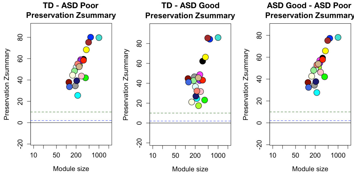
Fig. S3: Module preservation when WGCNA analysis is run separately on each group. This figure shows the module preservation Zsummary statistic for WGCNA analyses run separately on each group in order to show that networks are highly preserved ( Zsummary > 10 ) across groups.
