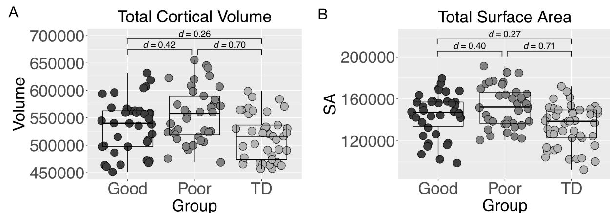
Fig. 1: Subtype differences in total cortical volume (A) and total surface area (B). Standardized effect sizes ( Cohen's d ) are shown for each pairwise group comparison.
