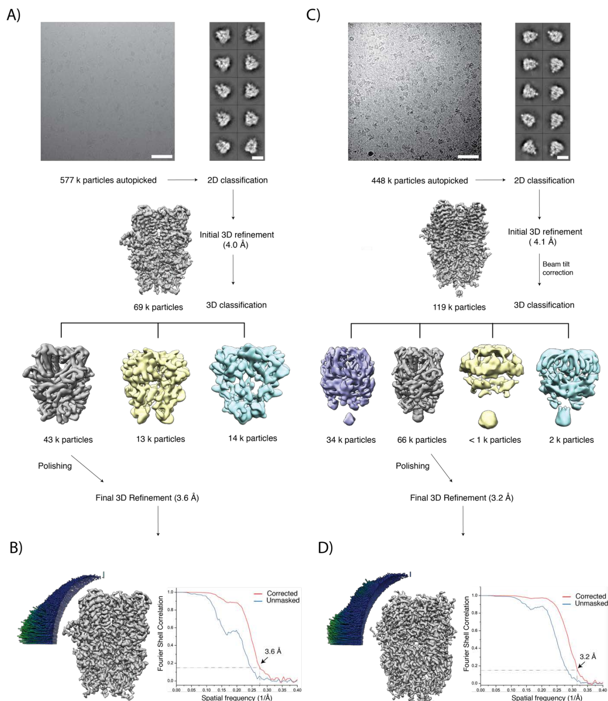
Figure S2. Cryo-EM image processing workflow for TRPC4 in complex with the inhibitor or activator.
