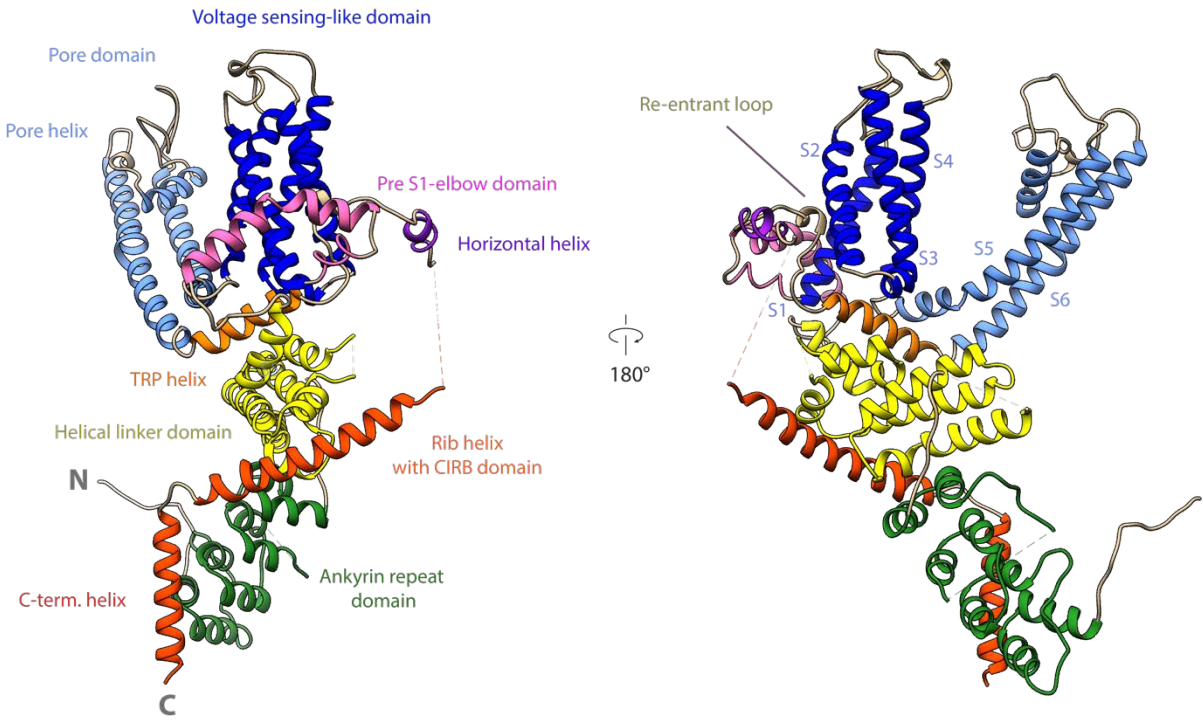
Figure S5. Domain architecture of zebrafish TRPC4 channel.
