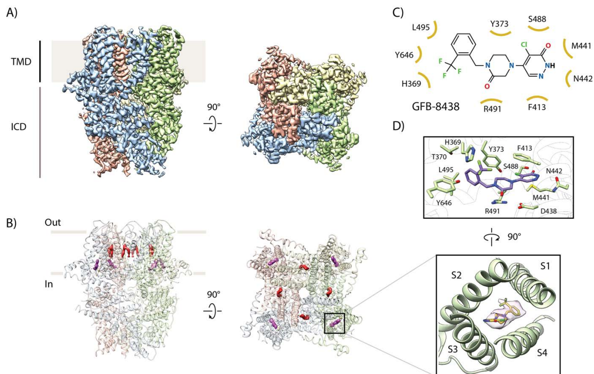
Figure 1. Cryo-EM structure of inhibitor-bound TRPC4 channel.
