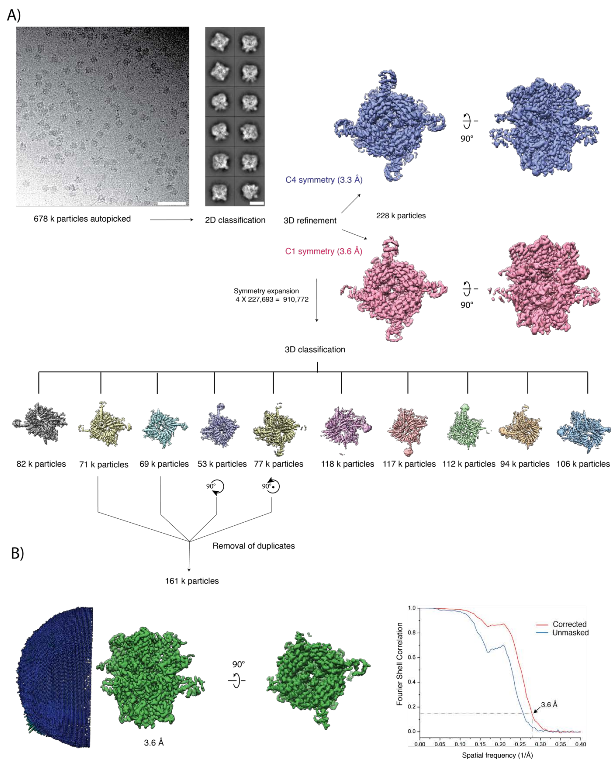
Figure S10. Cryo-EM image processing of the TRPC4- CaM complex.
