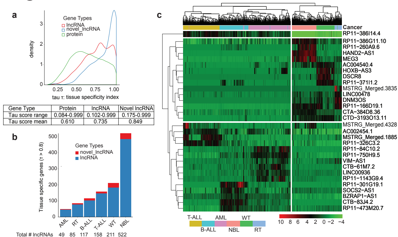
Fig 2: lncRNAs exhibit tissue specific expression that can distinguish cancers.
