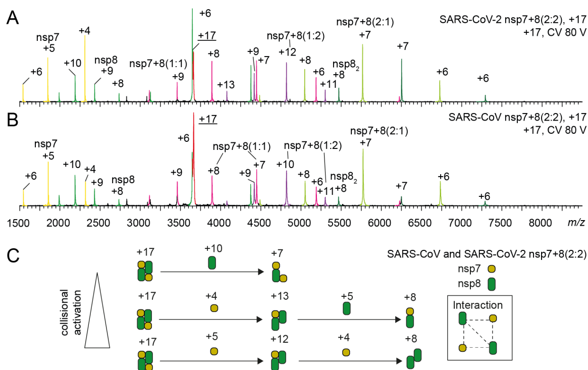
Figure S 10: Topological reconstruction from CID-MS/MS of SARS-CoV and SARS-CoV-2 nsp7+8 heterotetramers. Product ion spectra of (A) SARS-CoV-2 and (B) SARS-CoV 17+ nsp7+8 (2:2) heterotetramers are shown. High charge state precursor allows for efficient dissociation already at relatively low activation (CV 80 V). Product ion species can be clearly assigned from the overview spectra. (C) Schematic pathway of dissociation allows topological reconstruction of the SARS-CoV-2 and SARS-CoV heterotetramers.
