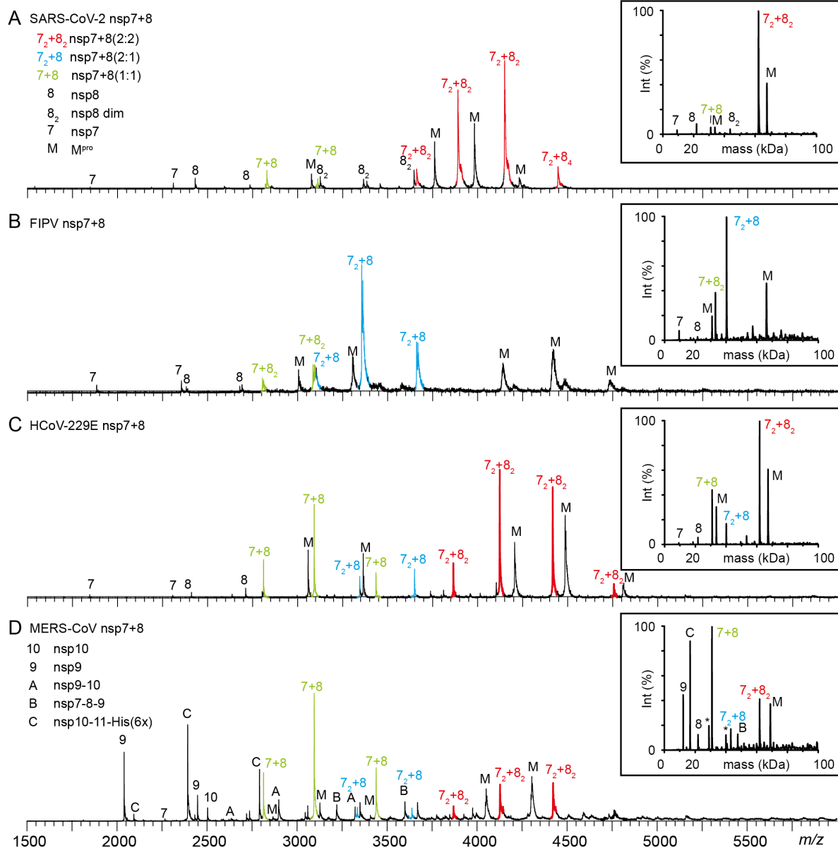
Figure 1: Three complexation groups formed by CoV nsp7+8. Representative mass spectra showing distinct nsp7+8 complexation patterns that were classified into the three groups A, B and AB. Complex formation triggered by M pro (M) mediated cleavage of 15 μM CoV nsp7-8-His 6 or MERS-CoV nsp7-11-His 6 precursors in 300 mM ammonium acetate (AmAc), 1 mM DTT, pH 8.0. (A) SARS-CoV-2 representing group A forms heterotetramers (nsp7+8 (2:2), red), (B) FIPV from group B forms heterotrimers (nsp7+8 (2:1), blue) and (C) HCoV-229E from group AB forms both complex stoichiometries (2:2 and 2:1). (D) In case of MERS-CoV, also group AB, cleavage of the longer nsp7-11-His 6 precursor resulted in additional processing intermediates (labeled A, B, C). In all three complexation groups, nsp7+8 (1:1) heterodimeric intermediates are observed (green). For spectra of all seven CoV nsp7+8 complexes see Figure S 2.
