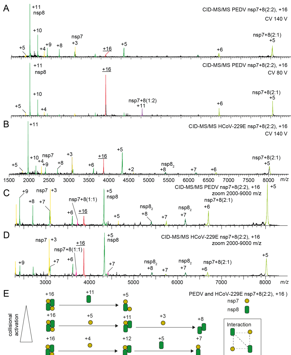
Figure S 8: Topological reconstruction from CID-MS/MS of PEDV and HCoV-229E nsp7+8 heterotetramers. (A) Product ion spectra of PEDV 16+ nsp7+8 (2:2) heterotetramers are shown at two different CV. At 80 V CV, the dissociation of one nsp7 or alternatively one nsp8 occurs, as indicated by the high and low charge products. Notably, the high charge state of the dissociated nsp8 suggests an extended shape of the ion. At 140 V CV, nsp8 dissociates at lower charge states suggesting alternative dissociation pathways. (B) Product ion spectra of HCoV-229E 16+ nsp7+8 (2:2) heterotetramers at 140 V are similar to the PEDV heterotetramers. (C and D) The zoom (2000-9000 m/z ), excluding the nsp8 high charge states, reveals additional product species (e.g. the nsp8 2 homodimer). (E) Schematic pathway of dissociation allows for a topological reconstruction of the PEDV and HCoV-229E heterotetramer.
