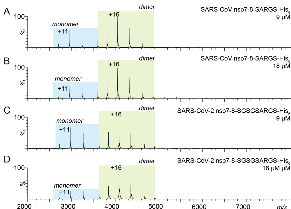
Figure S 5: Monomer-dimer equilibrium in SARS-CoV and SARS-CoV nsp7-8 precursors. Native mass spectra of nsp7-8 precursors of SARS-CoV (A) 18 \mu M and (B) 9 \mu M and SARS-CoV-2 (C) 18 \mu M and (D) 9 \mu M. Proteins at 18 \mu M were diluted to 9 \mu M, incubated for 10 min and then sprayed from 300 mM AmAc, pH 8.0 and 1 mM DTT. Charge states are labelled.
