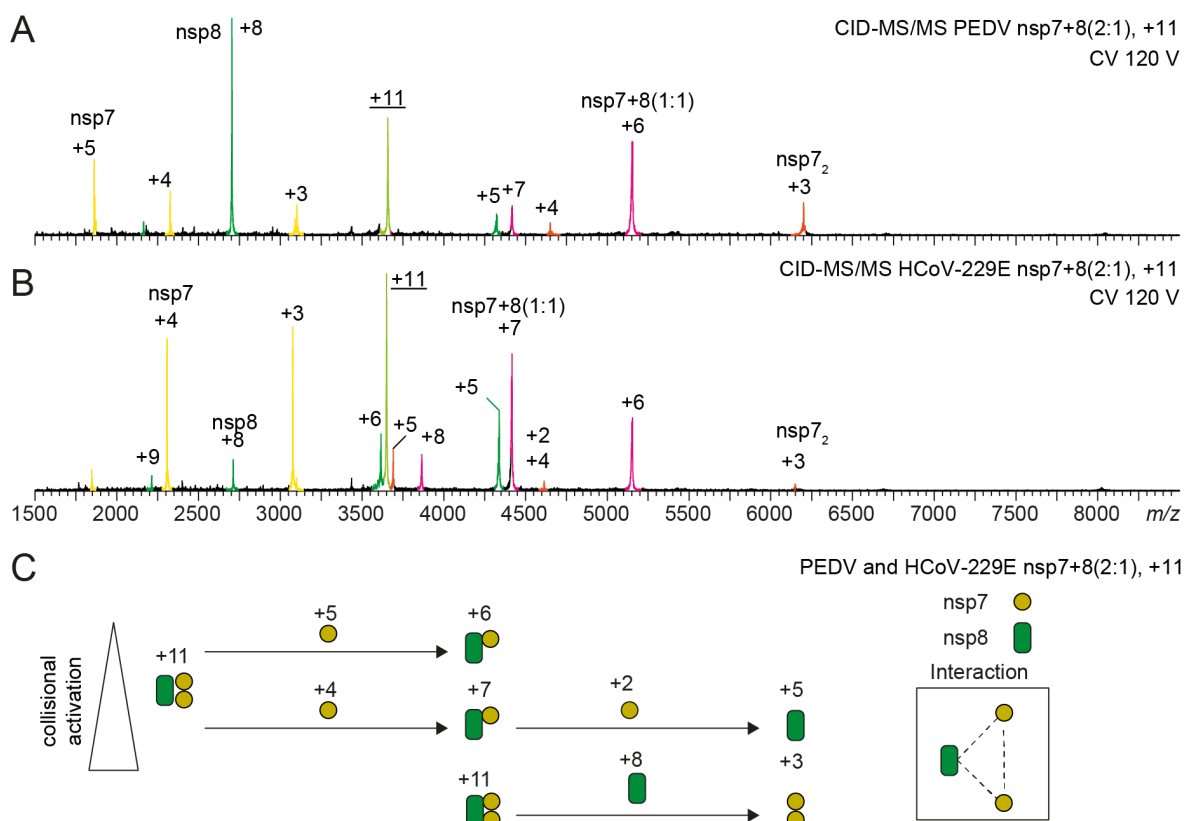
Figure S 7: Topological reconstruction from CID-MS/MS of PEDV and HCoV-229E nsp7+8 heterotrimers. (A) Product ion spectra of PEDV 11+ nsp7+8 (2:1) heterotrimers shows nsp7 homodimeric species, revealing the core interaction of this protein complex. (B) Product ion spectra of HCoV-229E 11+ nsp7+8 (2:1) heterotrimers are shown. Compared to the dissociation pattern of PEDV homologue, the HCoV-229E nsp7 and nsp8 high charge products have distinct intensities and charge state distributions but the detected product species are similar. (C) Schematic pathway of dissociation allows for a topological reconstruction of the PEDV and HCoV-229E heterotrimer.
