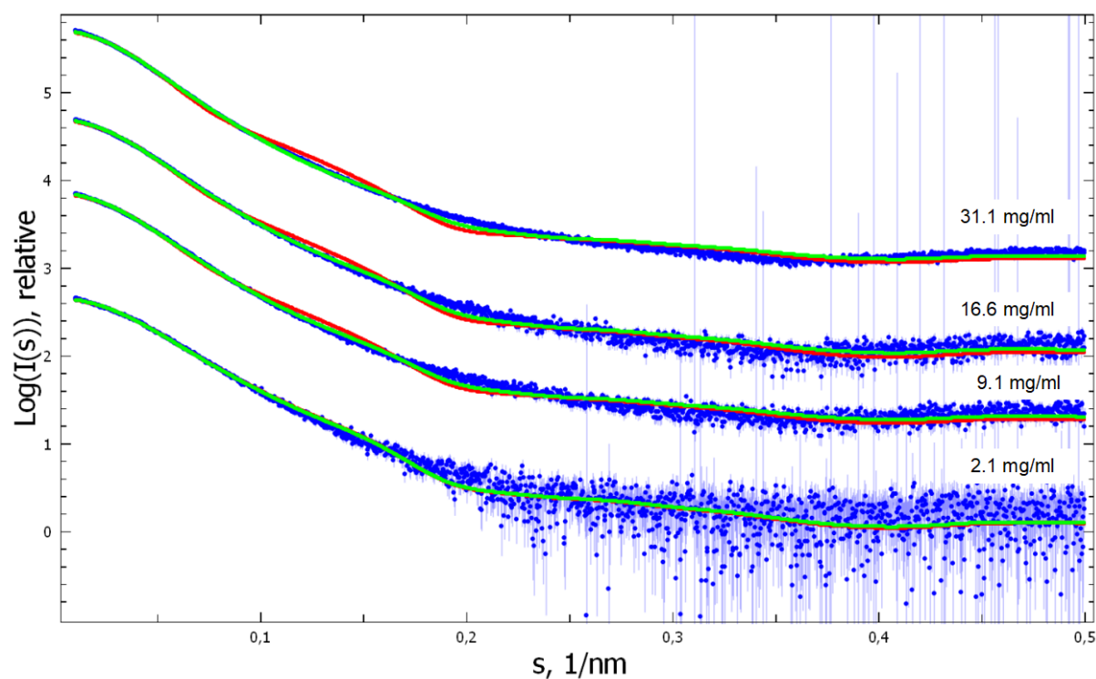
Figure S 14: Fits to all SAXS data. Experimental data (blue with experimental errors) for SARS-CoV-2 nsp7+8 complexes fitted with a mixture of T1 and hexadecamer (red), or T1 and dimer of T1 (green).
