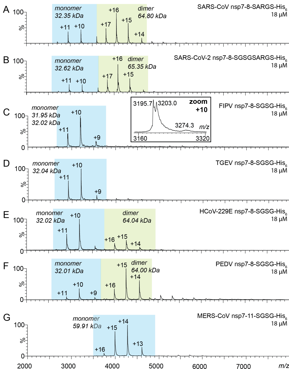
Figure S 4: Mass and oligomeric state of nsp7-8 precursors. Native MS of nsp7-8 precursors (A-G) sprayed at 18 \mu M from 300 mM AmAc, pH 8.0 and 1 mM DTT. Dominant charge envelope is highlighted (blue box). Labelled are charge states and molecular mass. (C) Inset shows mass heterogeneity in FIPV nsp7-8. The experimental molecular weight M_{exp} of the precursors agrees with the sequence-derived theoretical M_{theo} (Table S1). Only FIPV nsp7-8 contained two mass species separated by ~110 Da. This heterogeneity was attributed to the precursor's central nsp8 domain following M Pro processing. Assignment to an amino acid
