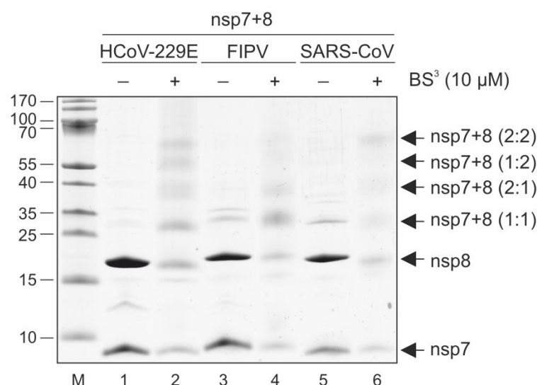
Figure S 12: SDS-PAGE analysis of chemically cross-linked HCoV-229E, FIPV, and SARS-CoV nsp7+8 complexes. The 5 µg protein of nsp7+8 complexes were crosslinked with 10 µM BS 3 (ThermoFisher) in reaction buffer (20 mM HEPES-KOH, pH 8.0, 30 mM KCl, and 2 mM β-mercaptoethanol). Crosslinking was carried out at 37 °C for 30 min and quenched with 50 mM AmAc for another 30 min at 37 °C. After terminating the crosslinking reaction, the samples were mixed with an excess of Laemmli sample buffer (50 mM Tris-HCl, pH 6.8, 2.5 % (w/v) SDS, 10 % (v/v) glycerol, and 0.01 % (w/v) bromophenol blue) and analyzed on 12 % SDS-PAGE. Lanes 1, 3, 5 – nsp7+8 complexes not treated with BS 3 (-) and lanes 2, 4, 6 – nsp7+8 complexes treated with BS 3 . Lane M, marker proteins; molecular masses in kD are indicated to the left. Black arrows on the right indicate the different oligomeric states of the nsp7+8 complexes obtained by crosslinking.
