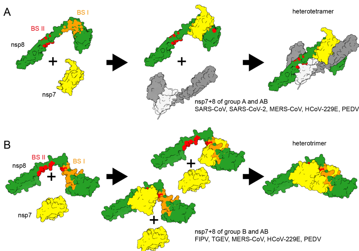
Figure 5: Proposed model for nsp7+8 complex formation. (A) For complexes of group A, heterodimers form via nsp8 BS I, which quickly dimerize via BS II into a heterotetramer. A theoretic route via a preformed nsp8 scaffold is unlikely to play a role in heterotetramer formation since no nsp7+8 (1:2) intermediates are observed for complexes of SARS-CoV or SARS-CoV-2. Moreover, nsp7 and nsp8 occupy neighboring positions in the replicase polyproteins, thus favoring their interaction ( in cis ) at early stages in the infection cycle (when intracellular viral polyprotein concentrations are low) over intermolecular interactions between different replicase polyprotein molecules as is also evident from the low dimerization ability of the precursors. (B) For group B complexes, we propose the formation of a heterodimer intermediate via nsp8 BS I or BS II and subsequent recruitment of a second nsp7, resulting an nsp7+8 (2:1) heterotrimer. This is also supported by the relatively high peak fractions of heterodimers detected. Group AB complexes can use both complexation pathways. In line with this, the proteins also produce a relatively high heterodimer signal but, ultimately, prefer to form heterotetramers rather than heterotrimers.
