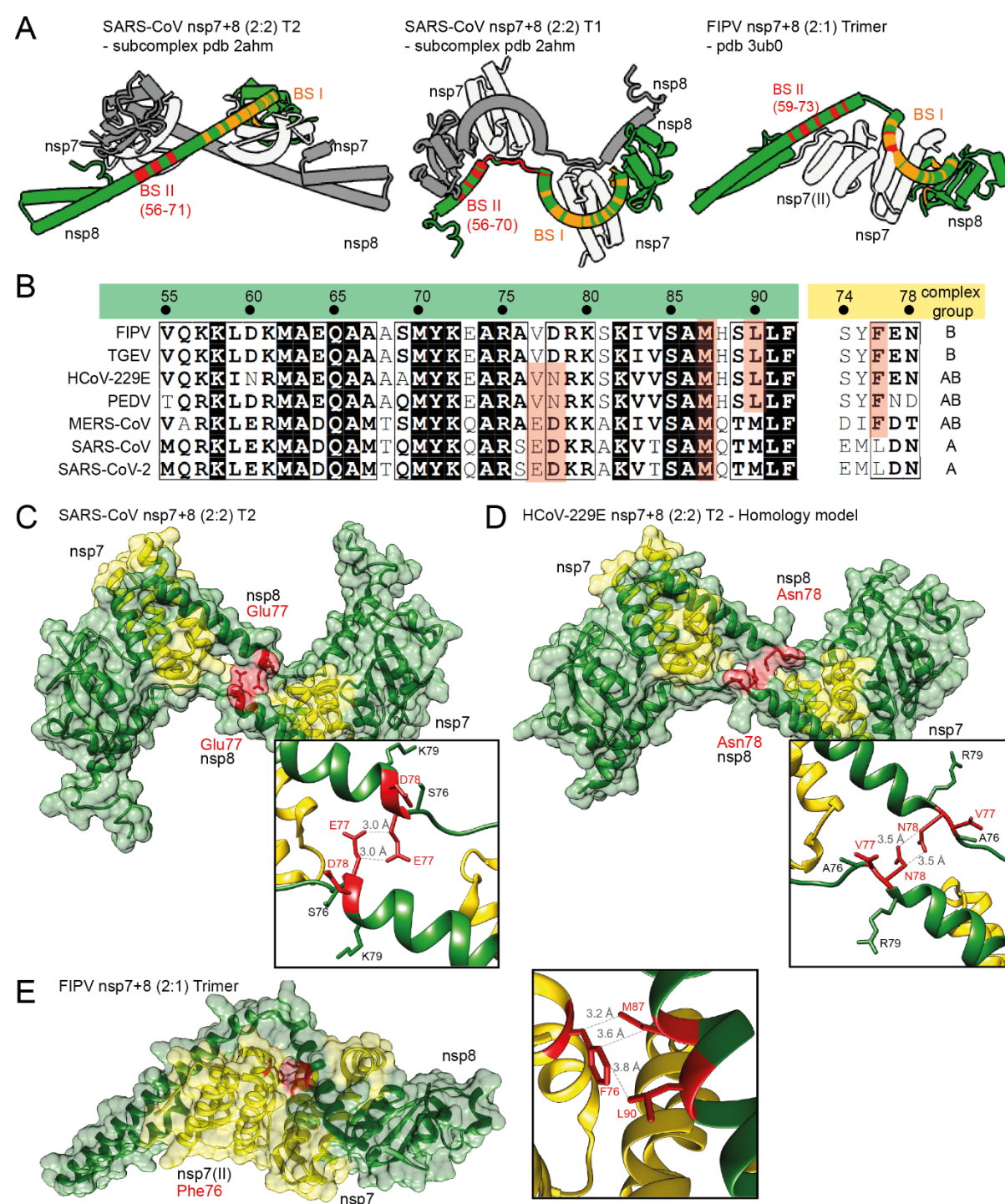
Figure 4: Candidate structures and sequence conservation of nsp7+8 heterotrimers and -tetramers. Candidate structures for nsp7+8 heterotetramer and -trimer are chosen based on experimental stoichiometry and topology
