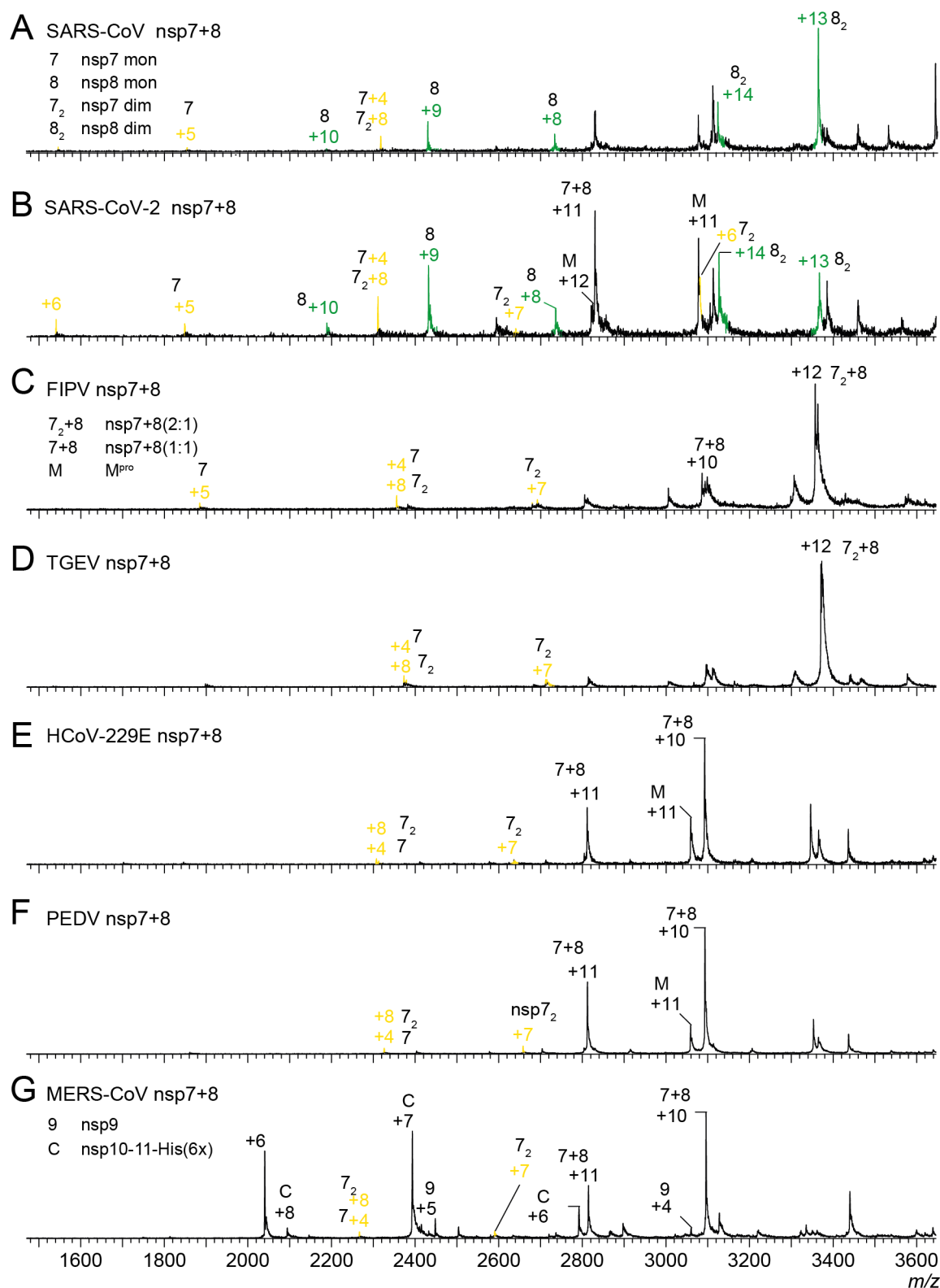
Figure S 3: Zoom in on nsp7 and nsp8 monomers and homodimers from spectra in Figure S 2. Representative native mass spectra showing region 1500-3600 m/z (for full spectra see Figure S 2) of cleaved nsp7-8 or nsp7-11 precursors showing that homodimers of nsp8 (green, nsp8 2 ) were detected for SARS-CoV (A) and SARS-CoV-2 (B), but not for (C) FIPV, (D) TGEV, (E) HCoV-229E, (F) PEDV and (G) MERS-CoV. Homodimers of nsp7 (yellow, nsp7 2 ) were detected for all seven CoVs.
