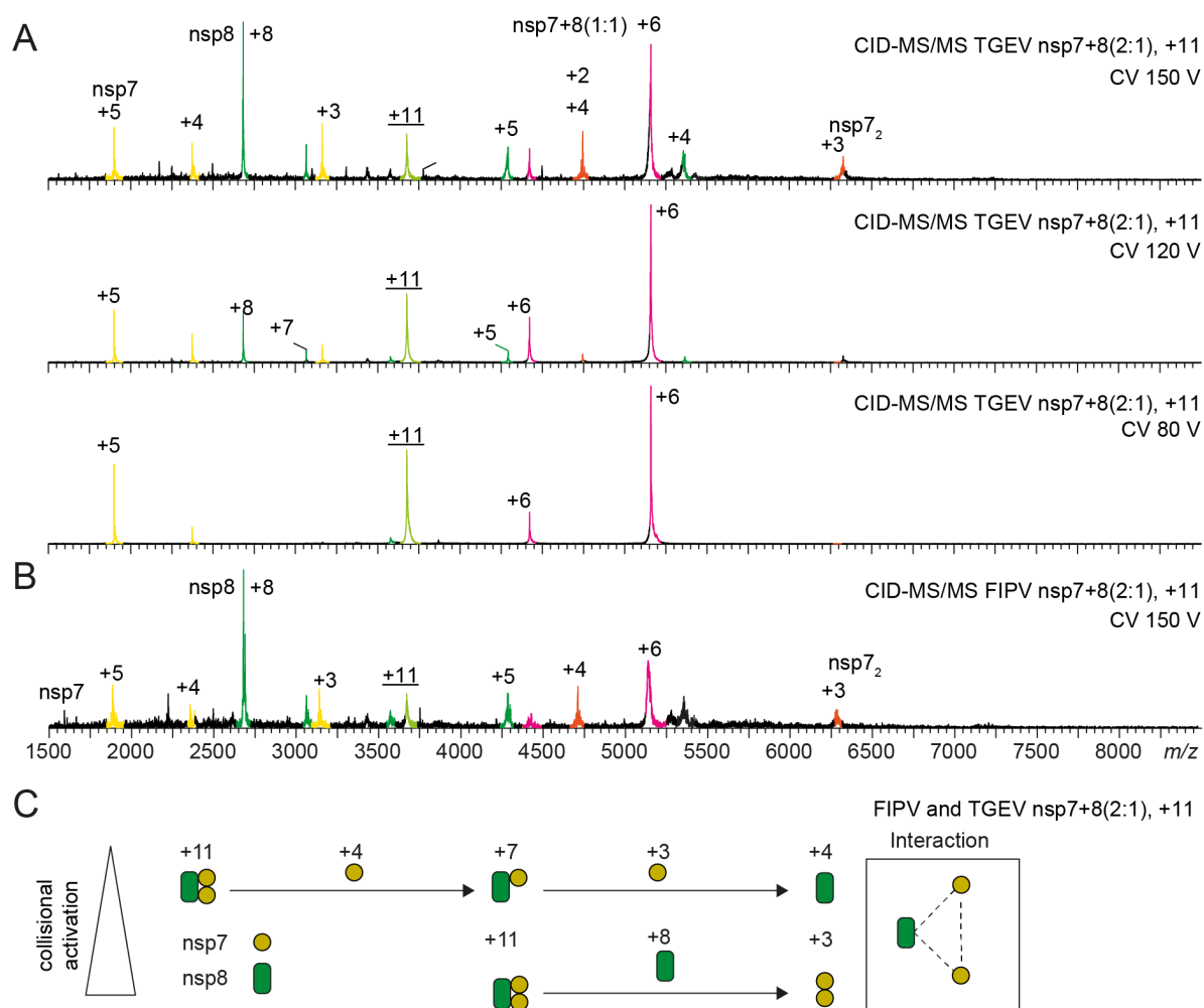
Figure S 6: Topological reconstruction from CID-MS/MS of TGEV and FIPV nsp7+8 heterotrimers. (A) Three product ion spectra of TGEV 11+ nsp7+8 (2:1) heterotrimers are shown at different collisional voltages (CV). Increased collisional activation allows assignment of additional charge states and product species. (B) Product ion spectra of the FIPV 11+ nsp7+8 (2:1) show a similar dissociation pattern as its homologue from TGEV. (C) Schematic pathway of dissociation allows for a topological reconstruction of the TGEV and FIPV heterotrimers.
