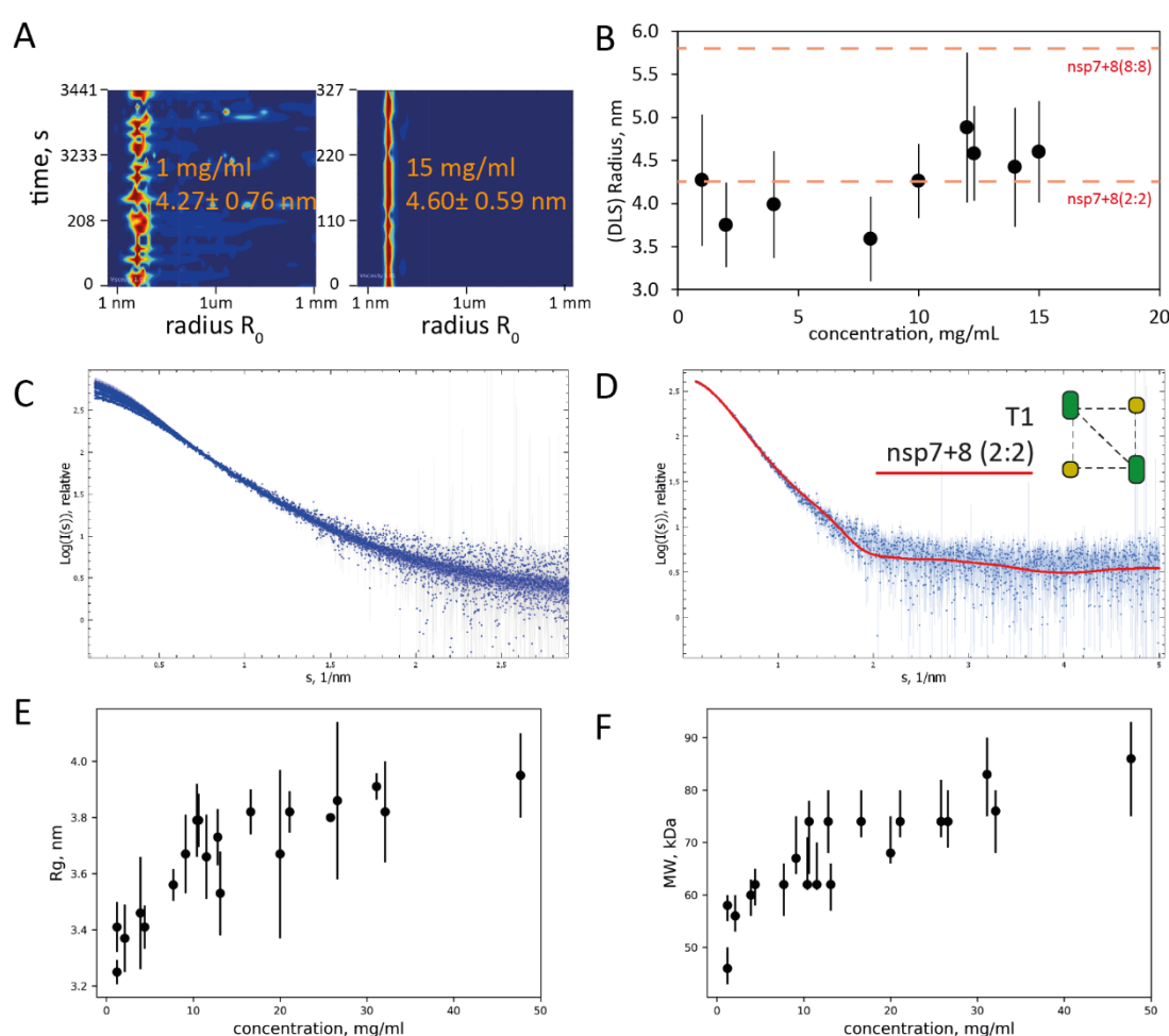
Figure 3: DLS and SAXS reveal oligomeric state of SARS-CoV-2 nsp7+8 at higher protein concentrations. At increasing protein concentrations, the hydrodynamic radius ( R_0 ) remains stable but becomes more homogenous in DLS. (A) shows two exemplary DLS plots (1 mg/ml; 15 mg/ml) and (B) how the radius R_0 develops with increasing protein concentration. Theoretical hydrodynamic radii ( R_{0,theo} ) of heterotetramer and hexadecamer candidate structures are indicated (red dashed lines). (C) displays SAXS curves collected at different solute concentrations and (D) the fit of the curve computed from T1 tetramer (red line) to the SAXS data collected at 1.2 mg/mL (blue dots with error bars). (E) Radius of gyration ( R_g ) and (F) molecular weight estimated from the SAXS data both stabilize with increasing concentration like in DLS on values that are in agreement with the R_{0,theo} of the T1 nsp7+8 (2:2) heterotetramer.
