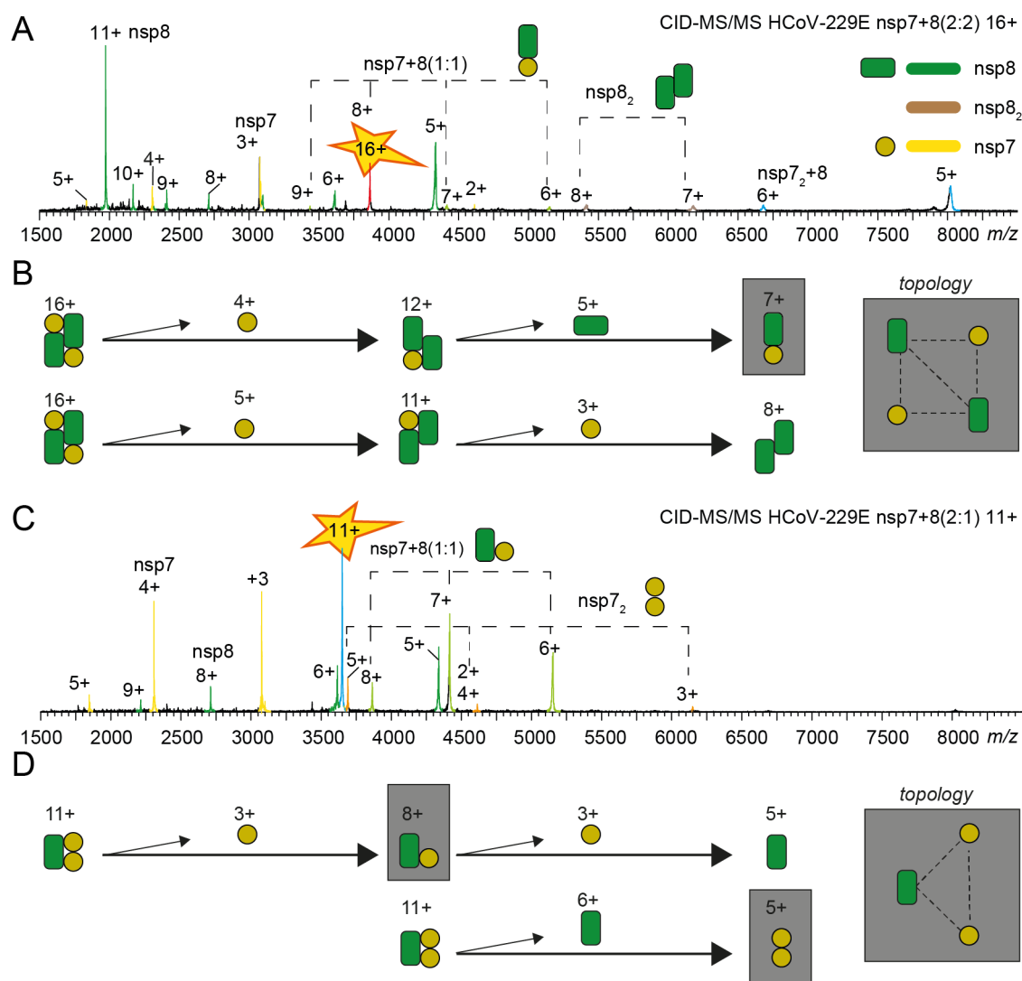
Figure 2: Gas-phase dissociation reveals complex topology. CID-MS/MS product ion spectra (A and C), dissociation pathways and topology maps (B and D) for HCoV-229E nsp7+8 (2:1) heterotrimers and (2:2) heterotetramers are shown. With increasing collisional voltage protein complexes are successively stripped from their subunits revealing alternative dissociation pathways. The remaining dimeric species expose direct subunit interactions in the nsp7+8 complexes (grey boxes). Charge states are labeled. (A and B) The heterotetramers (2:2) undergo two consecutive losses resulting in dimeric product ions of nsp7+8 (1:1) and nsp8 2 . These products indicate that nsp7:nsp8 and nsp8:nsp8 have direct interfaces in heterotetramers. (C and D) HCoV-229E heterotrimers dissociate into the dimeric products nsp7+8 (1:1) and nsp7 2 indicating direct interfaces between nsp7:nsp8 and nsp7:nsp7 in heterotrimers. All CoV heterotrimers follow similar dissociation pathways, also all CoV heterotetramers follow a common dissociation route, which allow a topological reconstruction of two distinct complex architectures (Figure S 6-Figure S 10).
