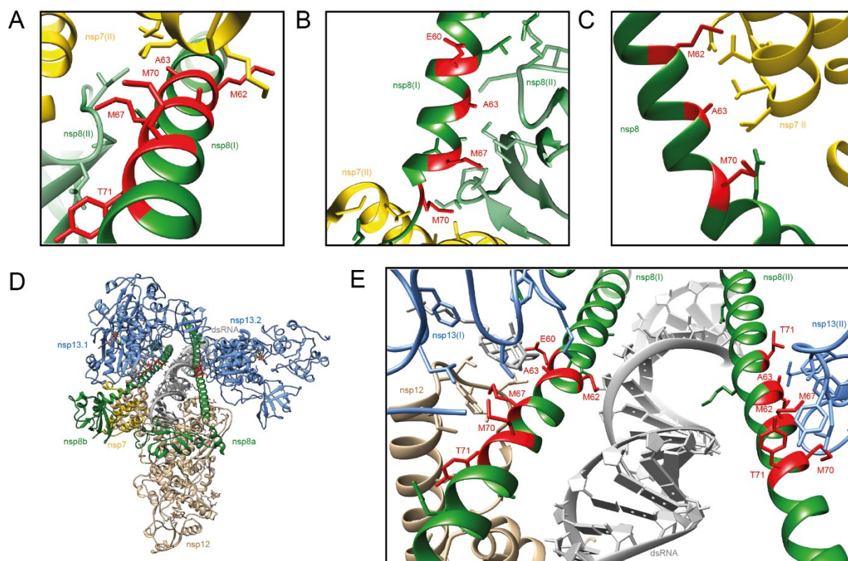
Figure S 16: Conserved stretch of nsp8 has various binding contexts. Candidate complexes involving similar conserved residues (red) in the nsp8 BS II are shown here for (A) the SARS-CoV nsp7+8 (2:2) heterotetramer candidate structures T1 and (B) T2 (subcomplexes of pdb 2ahm) as well as (C) the FIPV nsp7+8 (2:2) heterotrimer (pdb 3ub0). (D) Cryo electron microscopy structure of the nsp7+8+12+13 (1:2:1:1) polymerase complex (pdb 6xez) [29]. The two subunits of nsp8 (green), bind as a monomer nsp8a and as a nsp7+nsp8b heterodimer to the nsp12 RdRp. From there, nsp8a and nsp8b extend and interact as a facet with the RNA duplex and also individually with one subunit of the nsp13 helicase. The molecular contacts between nsp8 and nsp12/13 are mediated by exactly the same amino acids in the nsp8 BS II that are involved in nsp7+8 complex formation. (E) Zoom into the interacting region at nsp8a and nsp8b BS II and its amino acids in contact (VDW radius -0.4 Å) with the nsp12 thumb domain (brown), nsp13.1 and nsp13.2 (blue). All side chains of residues involved in contacts are displayed. Molecular graphics and analyses performed with UCSF ChimeraX, developed by the Resource for Biocomputing, Visualization, and Informatics at the University of California, San Francisco, with support from National Institutes of Health R01-GM129325 and the Office of Cyber Infrastructure and Computational Biology, National Institute of Allergy and Infectious Diseases [45].
