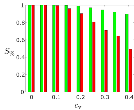
Fig. 6. Percentage of successfully switched Targets ( S\% ) in a balanced consortium ( N_t = N_a = N_d = 17 ) as the coefficient of variation c_v is varied. The bar plot in red (green) represents the percentage at steady state of Targets that, starting from ON (OFF) state, are turned OFF (ON) following the reference input r_{in} being switched to r_{in}^{OFF} ( r_{in}^{ON} ). For each value of c_v , the results of 100 simulations were averaged, each obtained by drawing independently all cells' parameters from normal distributions centered on their nominal values, \bar{\mu} , and with standard deviation \sigma = c_v \cdot \bar{\mu} .
