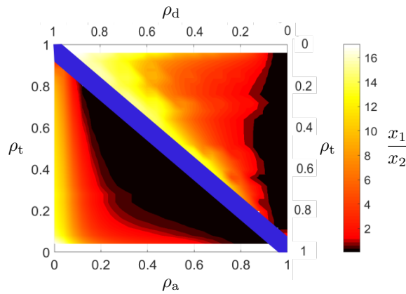
Fig. 5. Steady-state value of x_1/x_2 in response to switch commands, r_{in}^{OFF} (bottom left) and r_{in}^{ON} (top right), as the relative ratios of the three populations are changed. Switch commands are applied with the Targets starting from the opposite state. The total cell population in the consortium is set to N = 50 . For each cell type \rho_j = N_j/N , j = \{t, a, d\} , is its relative ratio within the consortium, and such that \rho_a + \rho_d + \rho_t = 1 .
