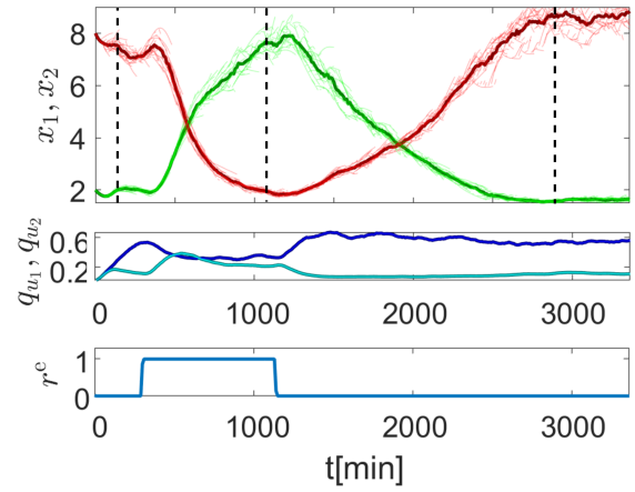
Fig. 3. Evolution of the average (thick lines) and single cell (thin lines) values of the concentrations of repressor proteins x_1 (green) and x_2 (red) in the Target population (top panel) when the reference signal r_{in}(t) is switched from low to high and vice versa. The middle panel shows the average value of the concentrations of quorum sensing molecules q_{u_1}^t (light blue) and q_{u_2}^t (dark blue) inside the Target cells. The bottom panel shows the value of r^e at the center of the chamber.
