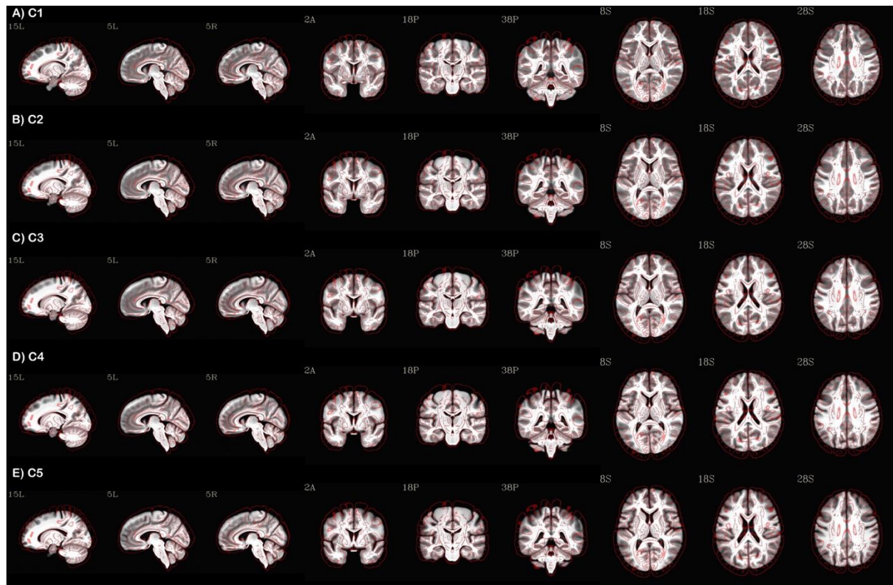
Figure S2: The five IBTs (C1-5) with three sets of sagittal, coronal and axial view displayed as underlay in grayscale and edge-filtered version of the MNI 2009 non-linear template mask as overlay for size comparison. High tissue contrast and detail are evident in each case.
