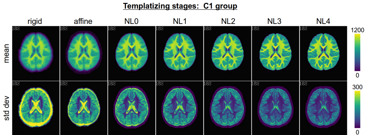
Figure 2 – Axial slices of mean (top row) and standard deviation (bottom row) maps through successive stages of the templating algorithm (first stage at the left) for the C1 age-band. Note that the mean and standard deviation maps have separate scales, to show details more clearly in each.
