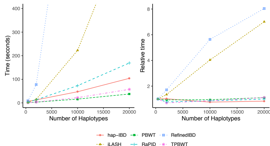
Figure 7: IBD computation runtimes and complexity for different methods. IBD computed for 42,927 SNPs from human chromosome 1. (Left) The x-axis is the number of haplotypes analyzed and the y-axis is the time in seconds taken to infer IBD. All methods were run using 1 CPU core. See Table 2 for parameter settings of the different methods. The four PBWT-based methods were at least an order of magnitude faster than the two non-PBWT-based methods; the original Durbin (2014) PBWT was the fastest. Computation times for TPBWT on larger datasets (millions of samples) using the parallel batching approach described in the main text are reported in Section 2.3 and Table 1. (Right) Runtime needed to compute IBD for each haplotype in samples sizes of 400 to 20000 haplotypes relative to the time needed to compute IBD for each haplotype in a sample size of 400. Slopes close to zero indicate linear time complexity, positive slopes indicate super-linear time complexity.
