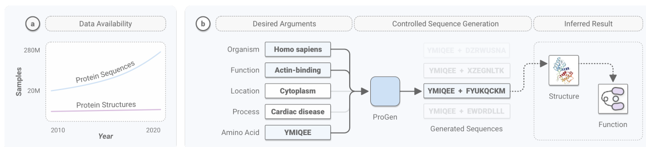
Figure 1. a) Protein sequence data is growing exponentially as compared to structural data. b) We utilize protein sequence data along with taxonomic and keyword tags to develop a conditional language model: ProGen.
