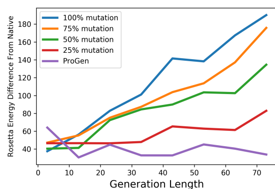
Figure 9. ProGen completion quality for VEGFR2 remains steadily near native conformational energy levels across generation lengths.
