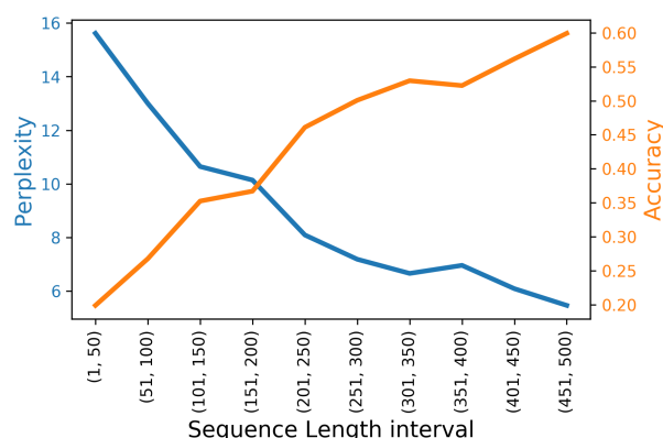
Figure 3. Full test set performance is better for later segments of sequences in keeping with intuition that additional context supports better predictions. We examined intervals up to 500 tokens to ensure a minimum of 30k samples per interval.
