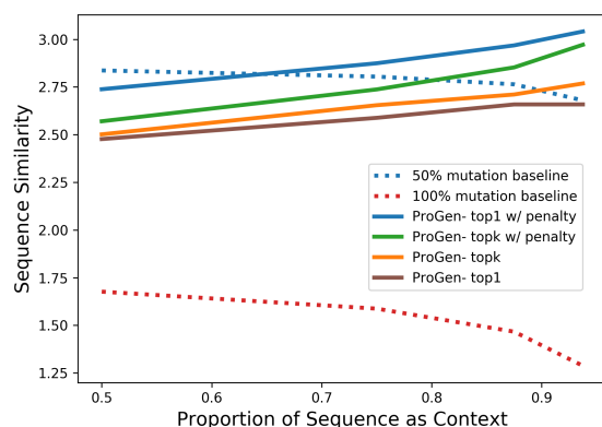
Figure 5. Across all context lengths, greedily sampling with a repetition penalty provides the best results according to sequence similarity.
