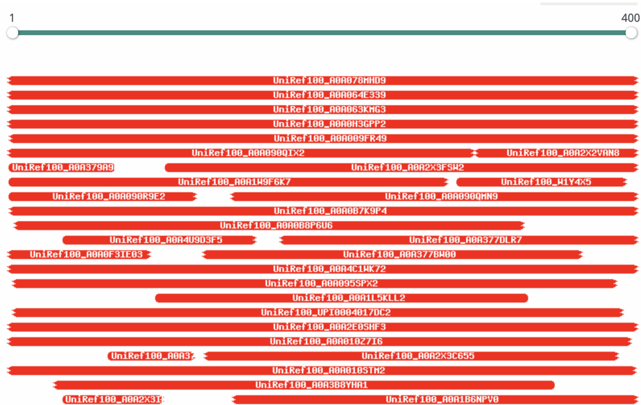
Figure 13. There are multiple sequences that align well with the ProGen generated FMN sequence from only conditioning tags. Many of the matching alignments have properties reflective of FMN proteins (e.g. oxidoreductases). A red color corresponds to a significantly low E-value, implying a matching homolog. The MSA was directly taken using HHblits.
