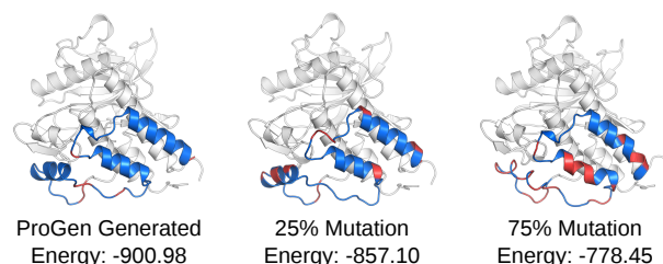
Figure 10. ProGen makes fewer mistakes and prioritizes conservation of secondary structure as compared to baselines. Blue is low energy (stable) and red high (unstable).
