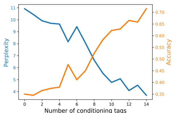
Figure 4. Full test set performance also improves as the number of conditioning tags associated with proteins increases. We examined proteins with up to 14 conditioning tags to ensure a minimum of 3k samples per category.
