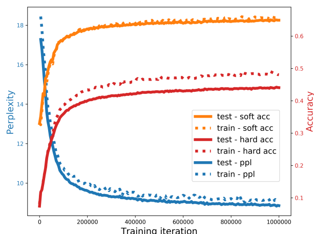
Figure 2. Large model capacity is warranted as ProGen has yet to overfit. BLOSUM62-informed soft accuracy shows no gap between train and test performance, suggesting hard accuracy hides the possibility that ProGen errors often correspond to amino acid substitutions found in nature. For metrics details see Section 3.4.
