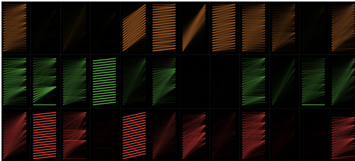
Figure 17. Attention patterns of ProGen for a given sequence. Layers 1-3 (rows) and attention heads 1-12 (columns) are displayed. The attention mechanism exhibits well-differentiated local and global patterns which may indicate specialization of each head on different tasks. Two corresponding attention heads from this visualization are shown in Figure 18.
