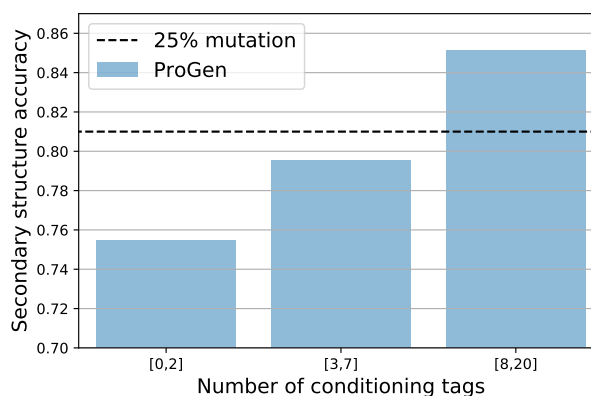
Figure 7. ProGen generates sequences that conserve secondary structure of the protein. Increasing the number of conditioning tags yields better secondary structure accuracy than the 25% mutation baseline.
