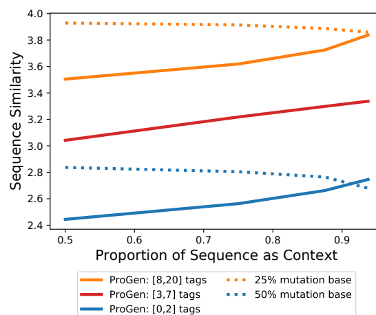
Figure 6. A greater number of conditioning tags enables higher quality generation. With at least 8 conditioning tags, generation quality approaches the 25% mutation baseline.
