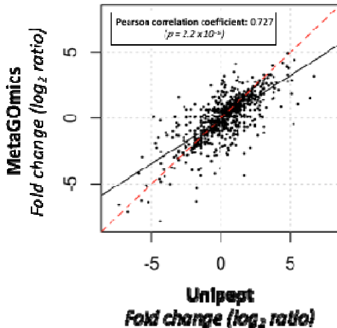
Figure 2 B) Comparison of quantitative expression for molecular function GO terms from Unipept and MetaGOmics. Log2ratio of spectral counts 'with sugar sample' (WS) against 'no sugar sample' (NS) was calculated for MetaGOmics- and Unipept-generated molecular function GO terms. Unipept identified 1,109 molecular function GO terms, while MetaGOmics identified 1,753 molecular function GO terms. The data points in figure represent quantitative values for 953 molecular function GO terms that overlapped between Unipept and MetaGOmics.
