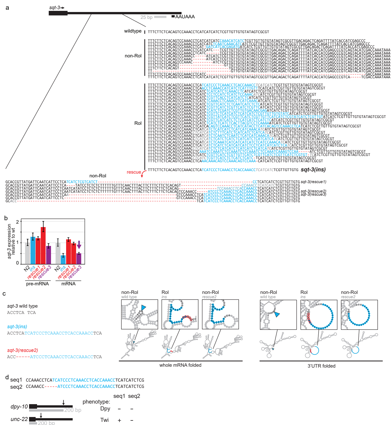
Supplementary Figure 10. Deletions affecting the repressive RNA element in the sqt-3(ins) 3' UTR can rescue the Rol phenotype. a , Nucleotide sequences of relevant 3' UTR regions in Rol, non-Rol and rescued mutants showing the inserted and deleted nucleotides. b , mRNA or pre-mRNA levels of sqt-3 in mutant and revertants at 26 hrs into synchronized development. Levels were quantified by qRT-PCR with primers specific for spliced or un-spliced transcript. c , Predicted RNA secondary structures of wild type, insertion mutant and rescued allele. Predictions were made for the whole mRNA or only the 3' UTR. d , Transplantation of mutant sequences into independent 3' UTRs. Sequence 1 (from insertion mutant) or sequence 2 (from rescued insertion mutant) were knocked-in at the dpy-10 or unc-22 3' UTR. Seq1 led to the characteristic reduction-of-function phenotype Twitching (Twi) in unc-22 .
