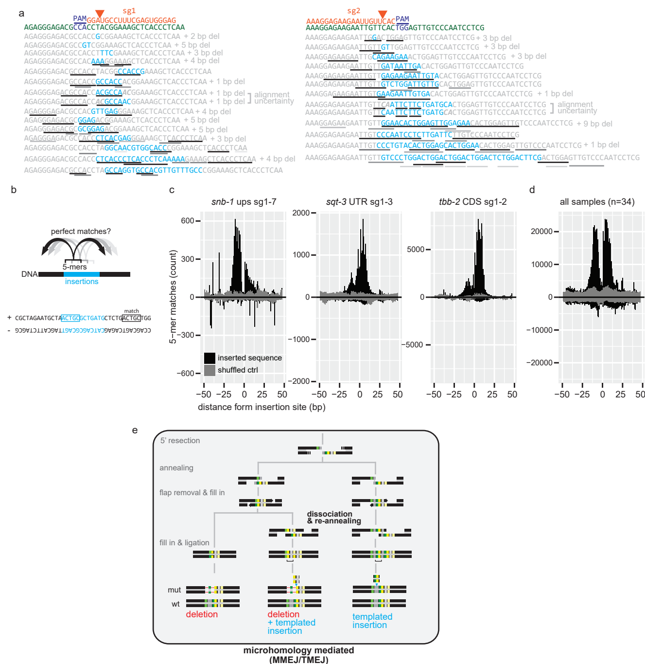
Supplementary Figure 4. Insertions are templated from surrounding sequences. a , Examples of microhomology observed between insertions and surrounding regions in genotypes of GFP-negative his-72::GFP animals. b , Scheme showing the analysis approach which matches all possible 5-mers from an insertion to the surrounding sequence. c , Matches of 5-mers from insertions to surrounding sequence (+/- 50bp), shown for three samples. d , For data from 34 samples, matches of 5-mers from insertions to surrounding sequence (+/- 50bp). e , Diagram showing mechanistic steps of dsDNA repair via microhomology-mediated end joining. Highlighted is the dissociation & re-annealing step which could lead to the templated insertions observed in our data.
