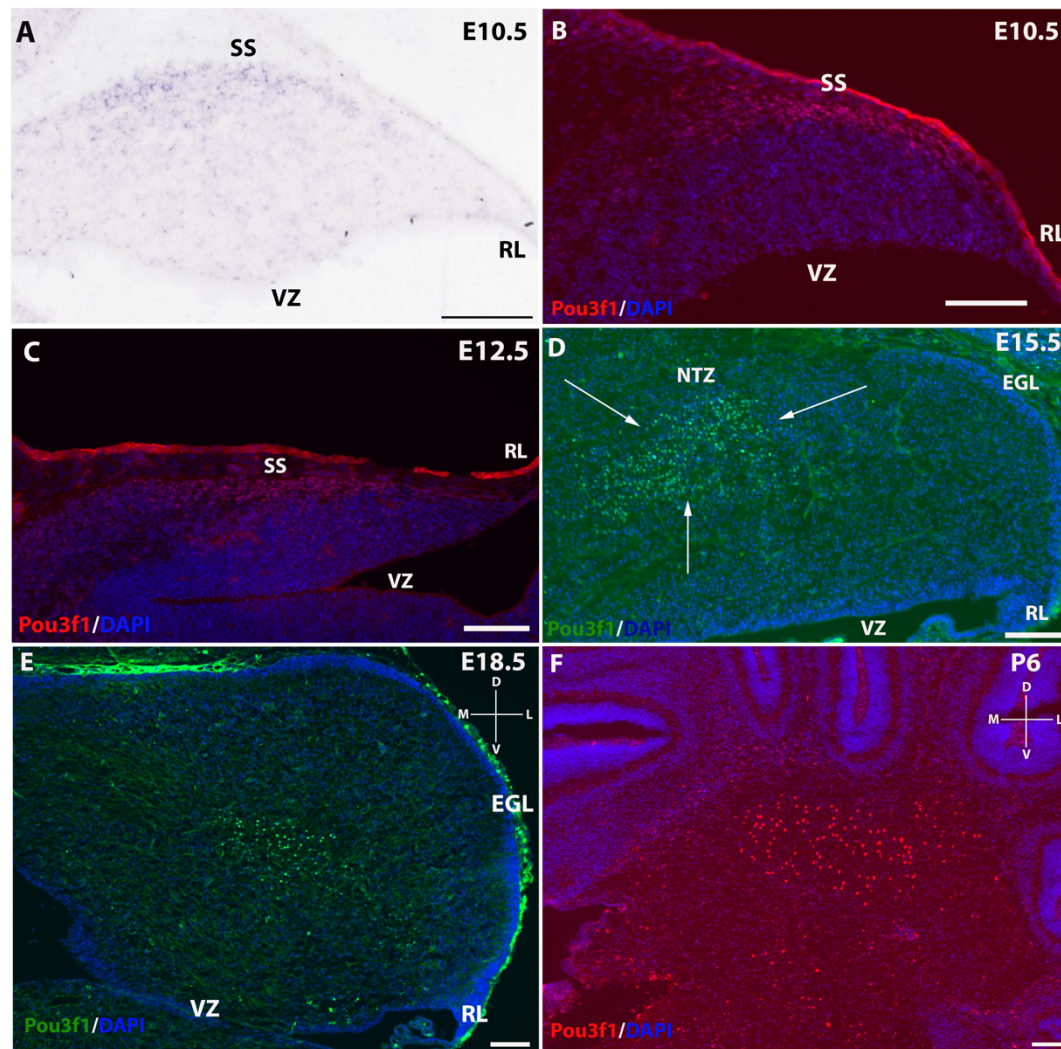
Figure 2. The expression pattern of Pou3f1 across space and time. A, B, C, In the E10.5 and E12.5 cerebella, in situ hybridization (ISH) (A) and immunofluorescent (IF) stainings (B, C) reveal that Pou3f1 is expressed in cells along the subpial stream (SS). D, In the E15.5 cerebellum, Pou3f1 is expressed primarily in the nuclear transitory zone (NTZ, white arrows). E, F, By E18.5, Pou3f1-expressing cells have reached the cerebellar white matter, with no noticeable change in spatial position at P6. A to D show sagittal sections of the cerebellum, while sections shown in E and F are in the coronal plane. D, dorsal. EGL, external germinal layer. L, lateral. M, medial. NTZ, nuclear transitory zone. RL, rhombic lip. SS, subpial stream. V, ventral. VZ, ventricular zone. Scale bars, 100 \mu m.
