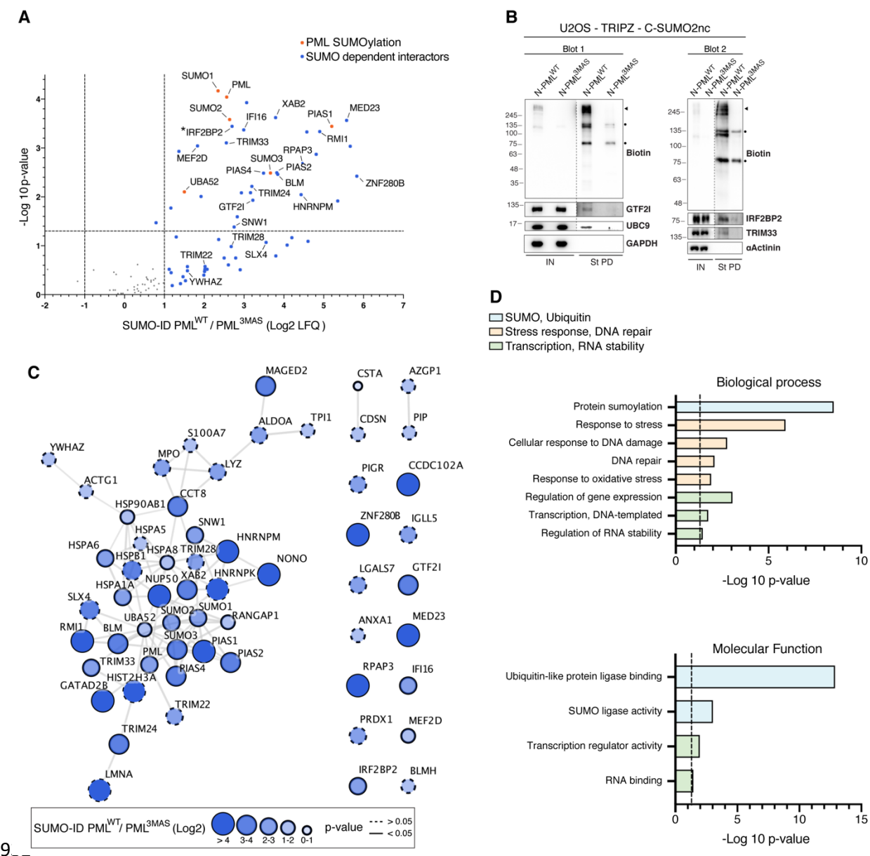
Figure 4: SUMO-ID identifies SUMO-dependent interactors of PML. (A) Volcano plot of LC-MS analysis comparing streptavidin pull-downs of U2OS double stable cell lines for TRIPZ-MYC-CTurboID 195 -SUMO2nc together with FLAG-NTurboID 194 -PMLIVa WT or FLAG-NTurboID 194 -PMLIVa 3MAS . Cells were treated with 1 µg/mL of doxycycline for 24 hours and 50 µM of biotin for 2 hours. 59 high-confidence SUMO-dependent PML interactors were defined. Asterisk (*) indicates that IRF2BP2 was detected with one peptide but further validated by Western blot and immunofluorescence. (B) Western blot validations of PML SUMO-dependent interactors identified by SUMO-
