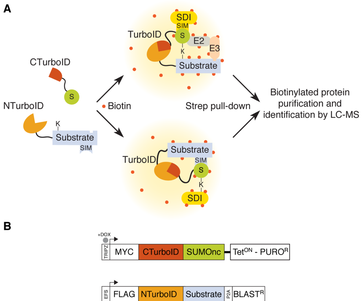
Figure 1: Identification of SUMO-dependent interactions: the SUMO-ID strategy.
