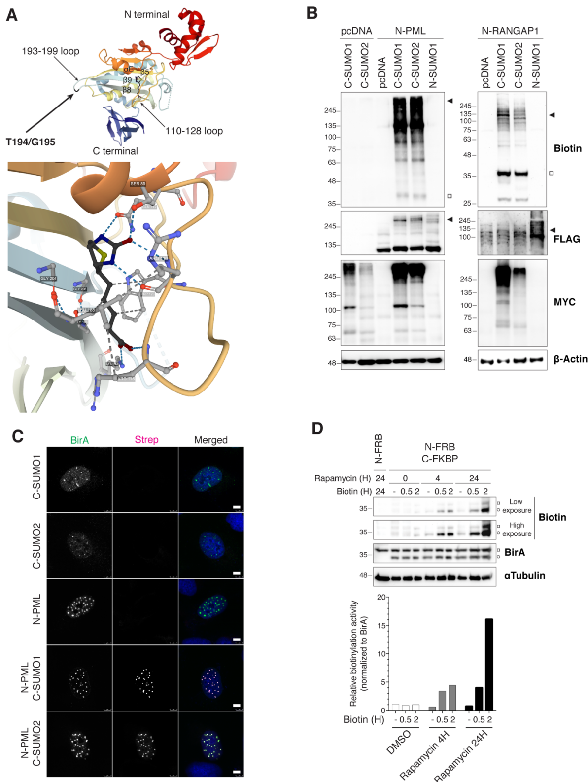
Figure 2: T194/G195 Split-TurboID is suitable for SUMO-ID studies. (A) Structure of the E. coli BirA with bound biotin (PDB ID: 1HXD 74,75 ), depicting the T194/G195 split point and the BirA-Biotin interaction. T194/G195 split point breaks the 193-199 loop
