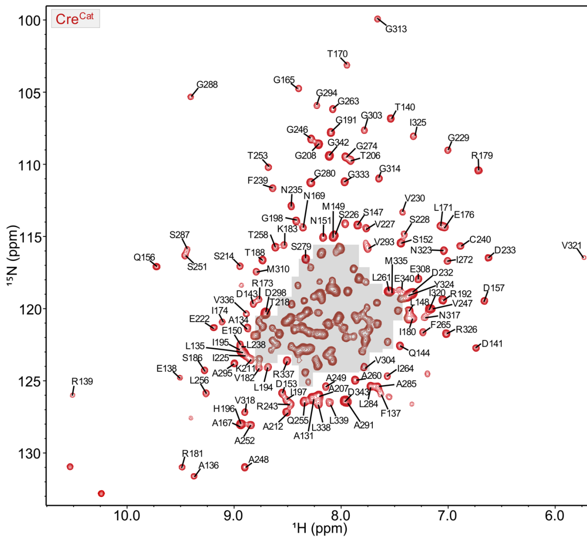
Figure S2. ^1\text{H} - ^{15}\text{N} TROSY-HSQC spectrum of \text{Cre}^{\text{Cat}} . Amide chemical shift assignments are indicated; those for the crowded region highlighted in gray are shown in Fig. S3.
