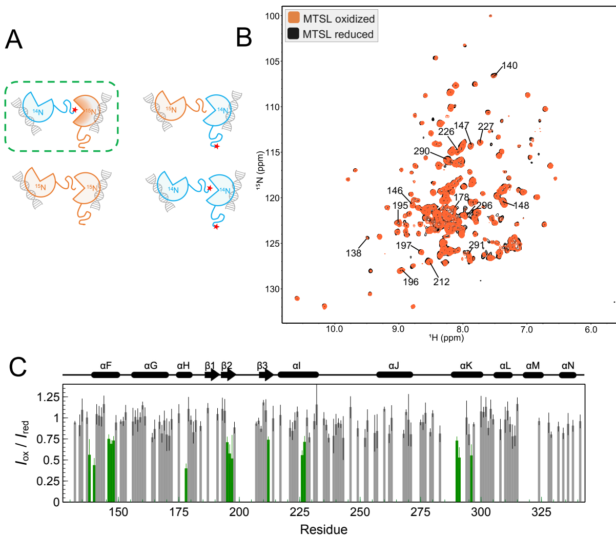
Figure S9. Strong Intermolecular PRE-NMR of \text{Cre}^{\text{Cat}} -DNA half-site complex is consistent with trans interactions via Cre C-terminus between half-site complexes.
