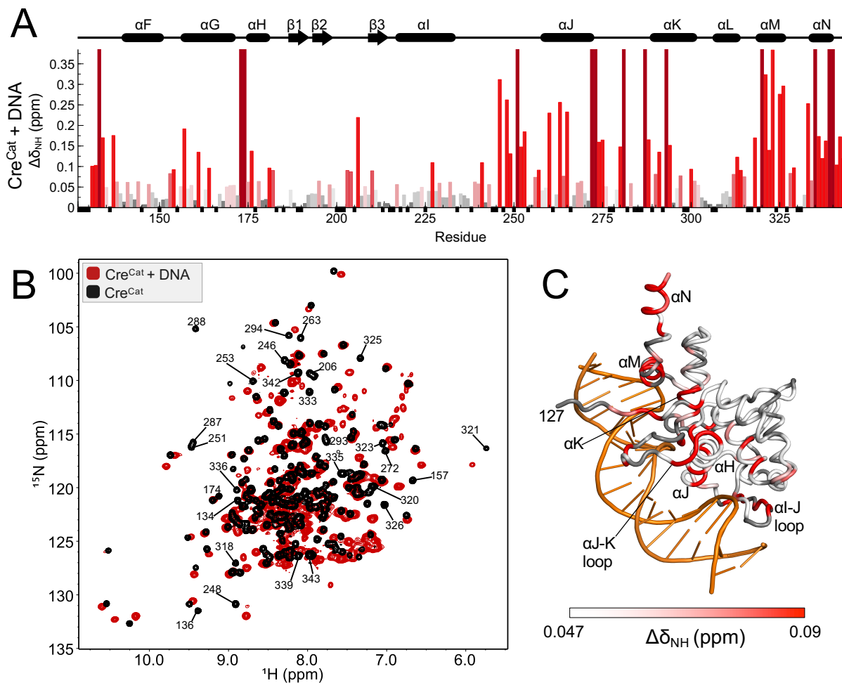
Figure 6. C-terminal helix \alpha N region of Cre Cat is perturbed upon binding to loxP DNA (A) Per-residue amide CSPs [ \Delta\delta_{NH} = (\Delta\delta_H^2 + \Delta\delta_N^2/25)^{1/2} ] of Cre Cat upon binding to loxP half-site hairpin DNA with a linear color ramp from gray (= 0 ppm) to red ( \geq twice the \Delta\delta SD (0.047 ppm)). Largest CSPs, or those that resulted in peak-broadening beyond detectability (assigned in free Cre Cat but unassigned in the Cre Cat -DNA complex) are shown in maroon. Unassigned residues are indicated by small negative black bars. Secondary structure elements of Cre synaptic complex crystal structure (PDB ID 2HOI, chain B) are shown above the plot. (B) Overlay of ^1H - ^{15}N TROSY-HSQC spectra of free Cre Cat (black) and bound to a DNA half-site (red) with select residue assignments indicated ( > 3 SD ppm). (C) CSPs mapped onto the crystal structure (PDB ID 2HOI, chain B) as a linear gradient from white ( \leq 1 SD ppm) to red ( \geq 2 SD ppm). Unassigned residues are shown in gray.
