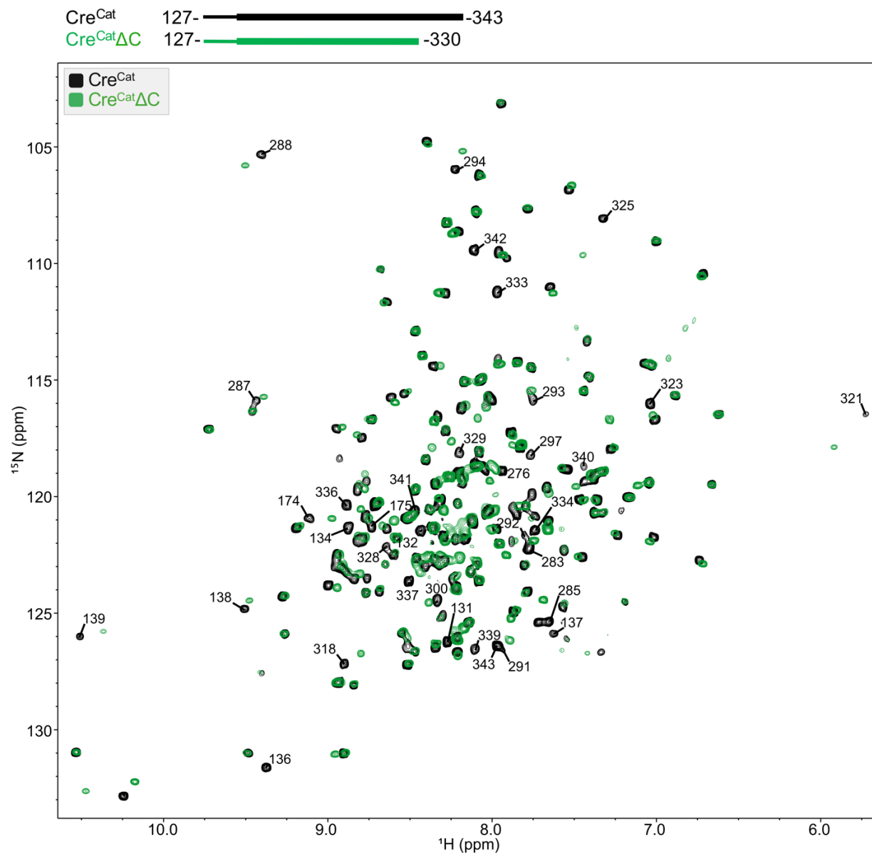
Figure S4. Truncation of C-terminal region causes CSPs in resonances from \text{Cre}^{\text{Cat}} core. Overlay of ^1\text{H} - ^{15}\text{N} TROSY-HSQC spectra of \text{Cre}^{\text{Cat}} (residues 127-343; black) and \text{Cre}^{\text{Cat}}\Delta\text{C} (residues 127-330; green). Assignments of residues with CSPs greater than 1 SD ( = 0.065 ppm) are indicated.
