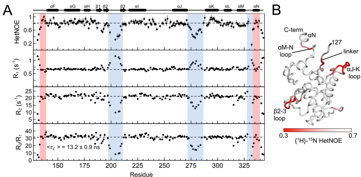
Figure 2. \text{Cre}^{\text{Cat}} loops \beta\text{2-3} , \alpha\text{J-K} and \alpha\text{M-N} , but not helix \alpha\text{N} , exhibit fast timescale dynamics. (A) \{^1\text{H}\} - ^{15}\text{N} Heteronuclear NOE, ^{15}\text{N} longitudinal R_1 relaxation rate constant (s ^{-1} ), ^{15}\text{N} transverse R_2 relaxation rate constant (s ^{-1} ) and corresponding R_2/R_1 ratios for \text{Cre}^{\text{Cat}} ; 800 MHz; 298 K. Dashed lines in panels represent average values calculated excluding regions of fast timescale dynamics. The secondary structure elements of \text{Cre}^{\text{Cat}} synaptic complex crystal structure (PDB ID 2HOI, chain B) are shown above the plot for comparison. (B) \{^1\text{H}\} - ^{15}\text{N} HetNOE values for \text{Cre}^{\text{Cat}} mapped onto the crystal structure (PDB ID 2HOI, chain B) as a linear gradient from red (= 0.3) to white ( \geq 0.7 ). Residues with no data are shown in gray.
