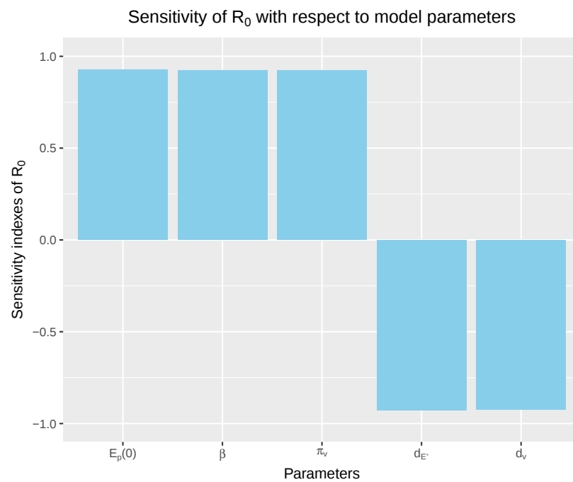
Figure 3: Sensitivity of R_0 with respect to E_p(0) , \beta , \pi_v , d_{E^*} , and d_v . The samples of parameters are taken from the uniform distribution U(0.8p, 1.2p) , where p is used to illustrate the mean value of parameters of COVID-19 that shown in Table.1.
