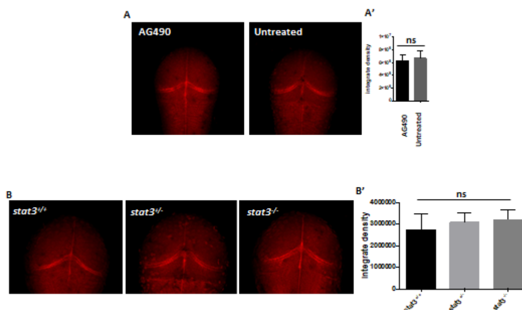
Fig. S6 mt_nd2 mRNA expression is not affected by AG-490 nor in 48-hpf stat3 mutant larvae. A: FISH with mt_nd2 probe in the TeO of 48-hpf larvae treated for 24 hours with AG490. A': fluorescence quantification of mt_nd2 mRNA levels in the TeO (n=10). B: FISH with mt_nd2 probe in the TeO of 48-hpf stat3 +/+ , stat3 +/- , and stat3 -/- larvae. B': fluorescence quantification of mt_nd2 mRNA levels in the TeO.
