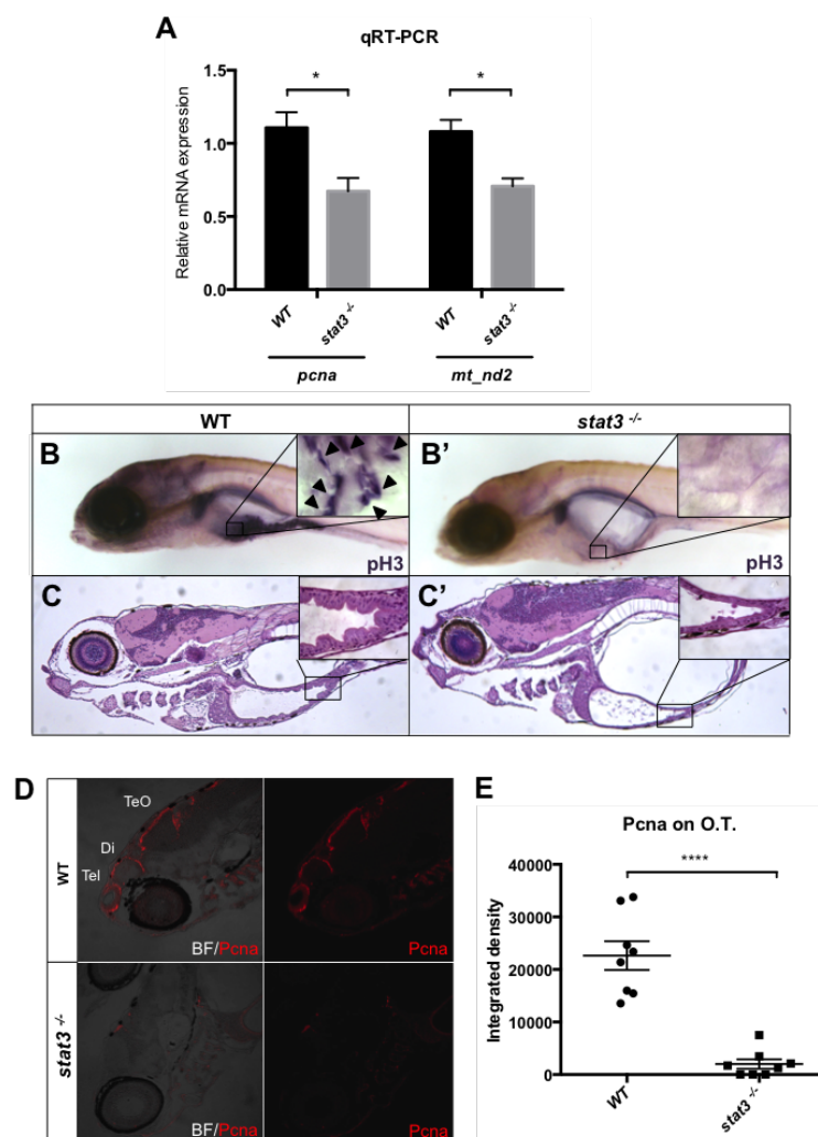
Fig. 9 stat3 KO impairs normal mitochondrial transcription and cell proliferation in the intestine and brain of 6-dpf zebrafish larvae. A: Relative mRNA expression of mt_nd2 and pcna transcripts assayed by qRT-PCR in homogenized stat3 -/- and WT siblings at 6 dpf; zgapdh was used as internal control (p-values= 0,0358; 0,0182). B-B': phospho-Histone-H3 (pH3) immunostaining of stat3 -/- and WT siblings at 6 dpf; zoom on the intestine. (pH3 positive cells=arrowheads). C-C': EE staining on WT and stat3 -/- mutant sections at 6 dpf shows the complete loss of folding in the mutant intestinal epithelium. D: IF with anti-PCNA Ab on 6-dpf stat3 -/- mutants showing decrease of fluorescence in the CNS (Tel= telencephalon; Di: diencephalon; TeO: tectum opticum). E: Fluorescence quantification of PCNA protein on lateral sections of 6-dpf stat3 -/- mutants and WT siblings; zoom on the head (n=8) (p-value<0,0001). Statistical analysis was performed by unpaired t-test on 3 independent biological samples (where n not specified). *p<0,05; ****p<0,0001; error bars=SEM.
