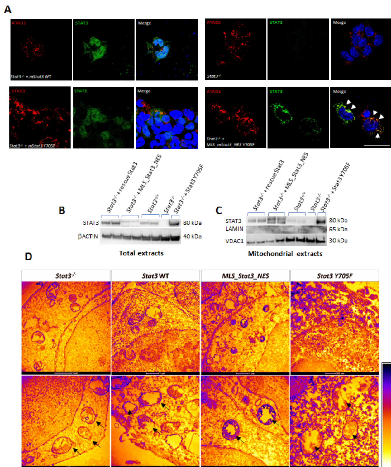
Fig. 5 Y705 phosphorylation is necessary for the correct localization of STAT3 in the mitochondrion. A: immunofluorescence with anti-STAT3 and anti-ATAD3 Ab on ESCs transiently transfected with the constructs used on zebrafish experiments. Arrows indicate the colocalization of ATAD and STAT3. Scale bar: 200 \mu m. B: western blot of total STAT3 in ESCs extracts, \beta -actin was used as a loading control. C: western blot of mitochondrial STAT3 from ESCs mitochondrial extracts, VDAC1 was used as a mitochondrial loading control, Lamin was used as a nuclear loading control. D: representative pictures of DAB immunohistochemistry on ESCs acquired with TEM and pseudo-colored to enhance
