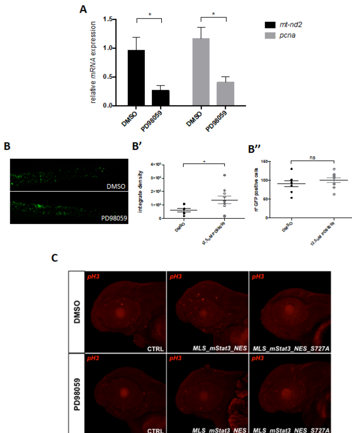
Fig. S5 MEK-ERK pathway regulates mitoStat3-driven cell proliferation by phosphorylating STAT3 on S727 residue. A: qRT-PCR analysis of mt-nd2 and pcna in 48-hpf larvae treated with 12.5 \mu M PD98059 from 24-48 hpf. B: representative pictures of Tg(7xStat3:EGFP) transgenic larvae treated with 12.5 \mu M PD98059 from 24 dpf to 96 dpf. B': fluorescence quantification of Tg(7xStat3:EGFP) transgenic larvae treated with 12.5 \mu M PD98059 from 24 dpf to 96 dpf. B'': number of EGFP positive cells in intestines of Tg(7xStat3:EGFP) transgenic larvae treated with 12.5 \mu M PD98059 from 24 dpf to 96 dpf. Statistical analysis was performed by unpaired t-test on 3 independent biological samples.
