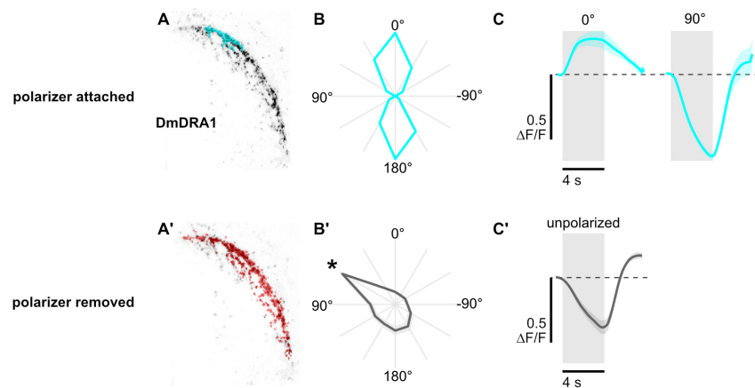
Figure S2: Polarization-opponent flash responses in DmDRA1
