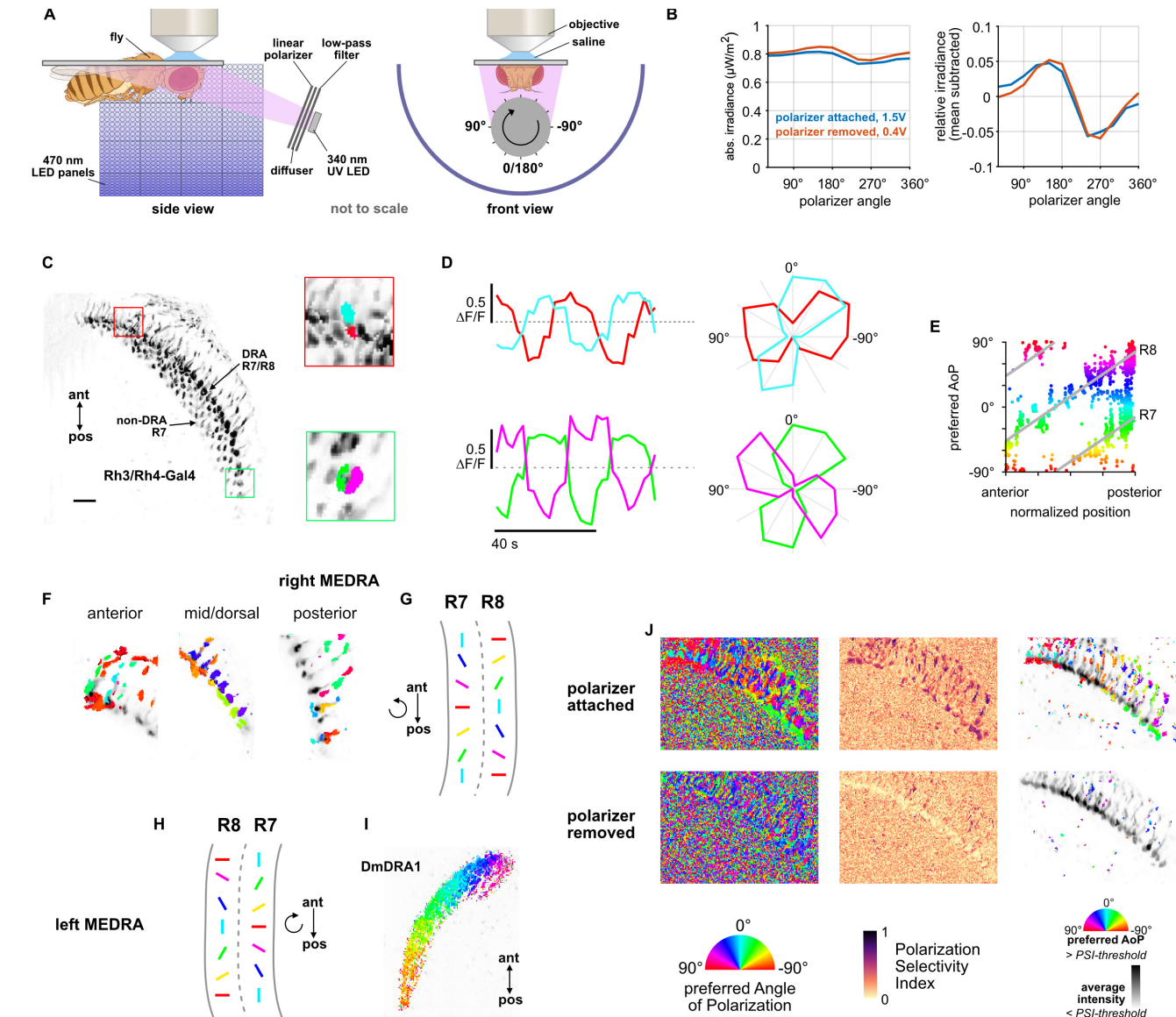
Figure S1: Polarizer characterization and R7/R8 photoreceptor stimulation
