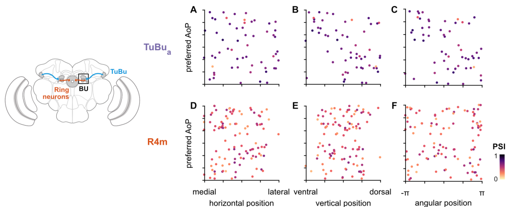
Figure S5: Unstructured organization of preferred angles of polarized light in the anterior bulb
