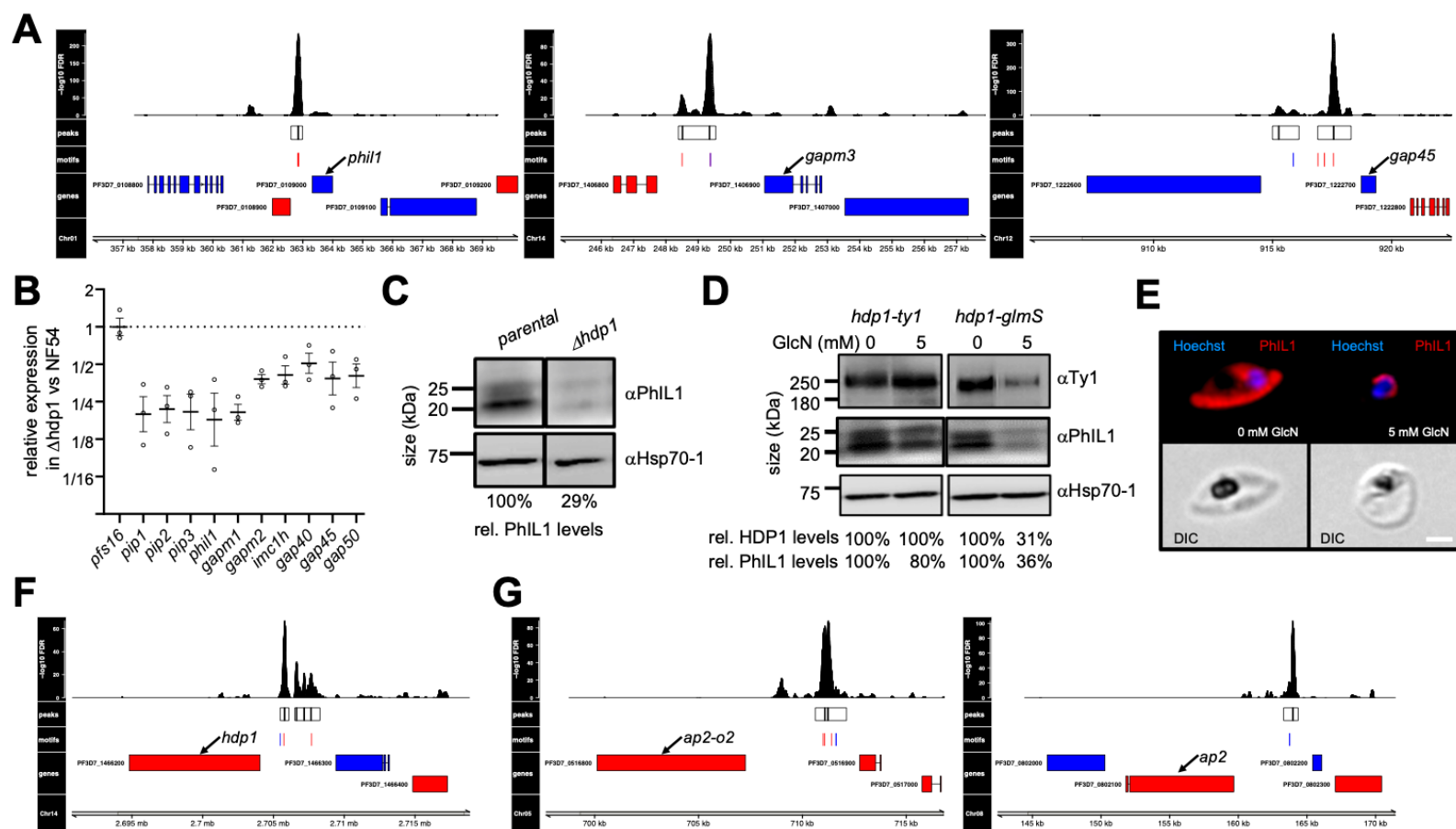
Fig. 5: HDP1 is essential for expansion of the inner membrane complex in early gametocytes. (A) Example HDP1 binding sites upstream of genes encoding inner membrane complex proteins. Histogram track shows the significance of enrichment by position. Regions of significant enrichment are shown as boxes with black vertical lines indicating peak summits within each peak. Instances of Motif A Motif B, or overlapping motifs within peaks are shown in red, blue and purple, respectively. Genes encoded in forward or reverse orientation are shown in blue or red, respectively. Combined estimate of n=2 . (B) Validation of down-regulation of genes encoding inner membrane complex genes in HDP1 knockout parasites by qRT-PCR. n=3 (C) PhIL1 expression in parental and \Delta hdp1 gametocytes. Hsp70-1 abundance shown as the loading control. Representative result of n=2 . (D) Day 5 morphology of hdp1-tyl and hdp1-glmS gametocytes under 0 and 5 mM glucosamine. HDP1 and PhIL1 protein levels in hdp1-tyl and \Delta hdp1 day 5 gametocytes. Hsp70-1 abundance shown as the loading control. Representative result of n=3 . (E) Immunofluorescence microscopy of PhIL1 distribution in day 5 gametocytes of hdp1-glmS under 0 and 5 mM glucosamine. Scale Bar: 3 \mu m (F-G) HDP1 binding sites upstream of genes encoding HDP1 itself and two ApiAP2 proteins. Tracks are the same as in (A).
