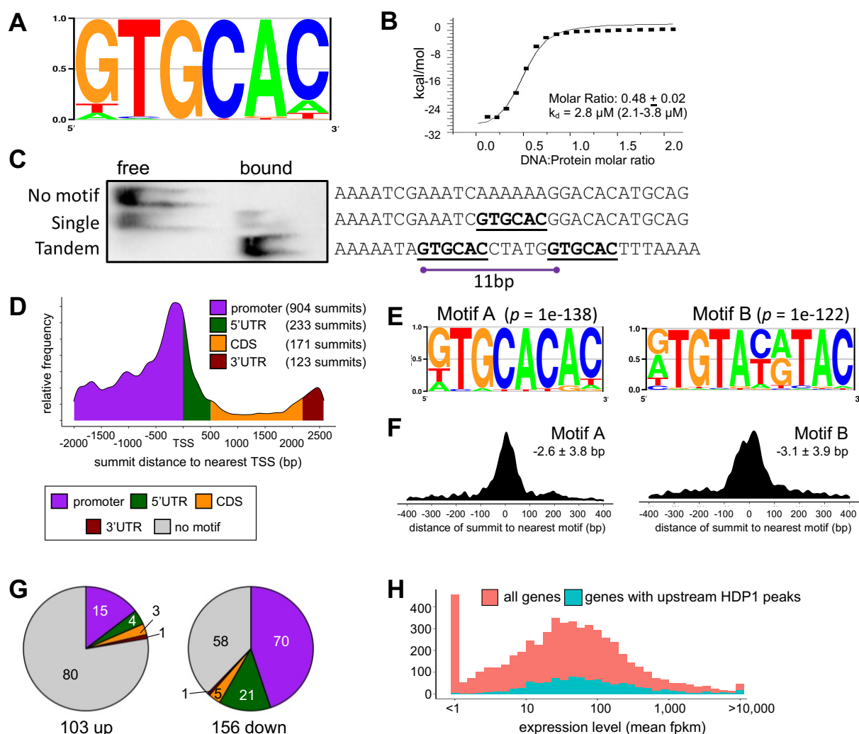
Fig. 4: HDP1 binds near the TSS of genes expressed in early gametocytes. (A) Maximum enrichment DNA motif for the GST-HDP1 DBD as determined by from protein binding microarray. y-axis shows the fraction of each base at that position. (B) Isothermal calorimetry indicates the HDP1-DBD domain recognizes DNA as a dimer. n=2 . (C) Optimal gel-shift was observed for probes containing a tandem motif with a 5bp spacer compared to probes with either a single or no motif. Representative of n=3 . (D) Distribution of gene-associated HDP1 ChIP-seq binding sites ( n=2 ). Relative distance to the transcription start site (TSS) is shown on the x-axis. Length of gene features shown is the median length of features with HDP1 binding summits. Summits found within regions mapping to two adjacent genes (242/1188 summits) were counted for both. (E) Highly enriched sequence motifs within 100 bp centered on HDP1-GFP ChIP-seq summits. y-axis shows the fraction of each base at that position. (F) Density graph of the distance between instances of Motif A (left) or Motif B (right) within HDP1-bound regions to the nearest ChIP-seq summit. The mean distance \pm s.e.m. is also shown. (G) Number of differentially regulated genes based on location of HDP1-bound regions. (H) Histogram of mean expression levels in early gametocytes of NF54 for all genes (red) and genes with upstream (promoter or 5'UTR) HDP1 motifs (teal). Note the lack of genes with HDP1 upstream peaks that have very low expression.
