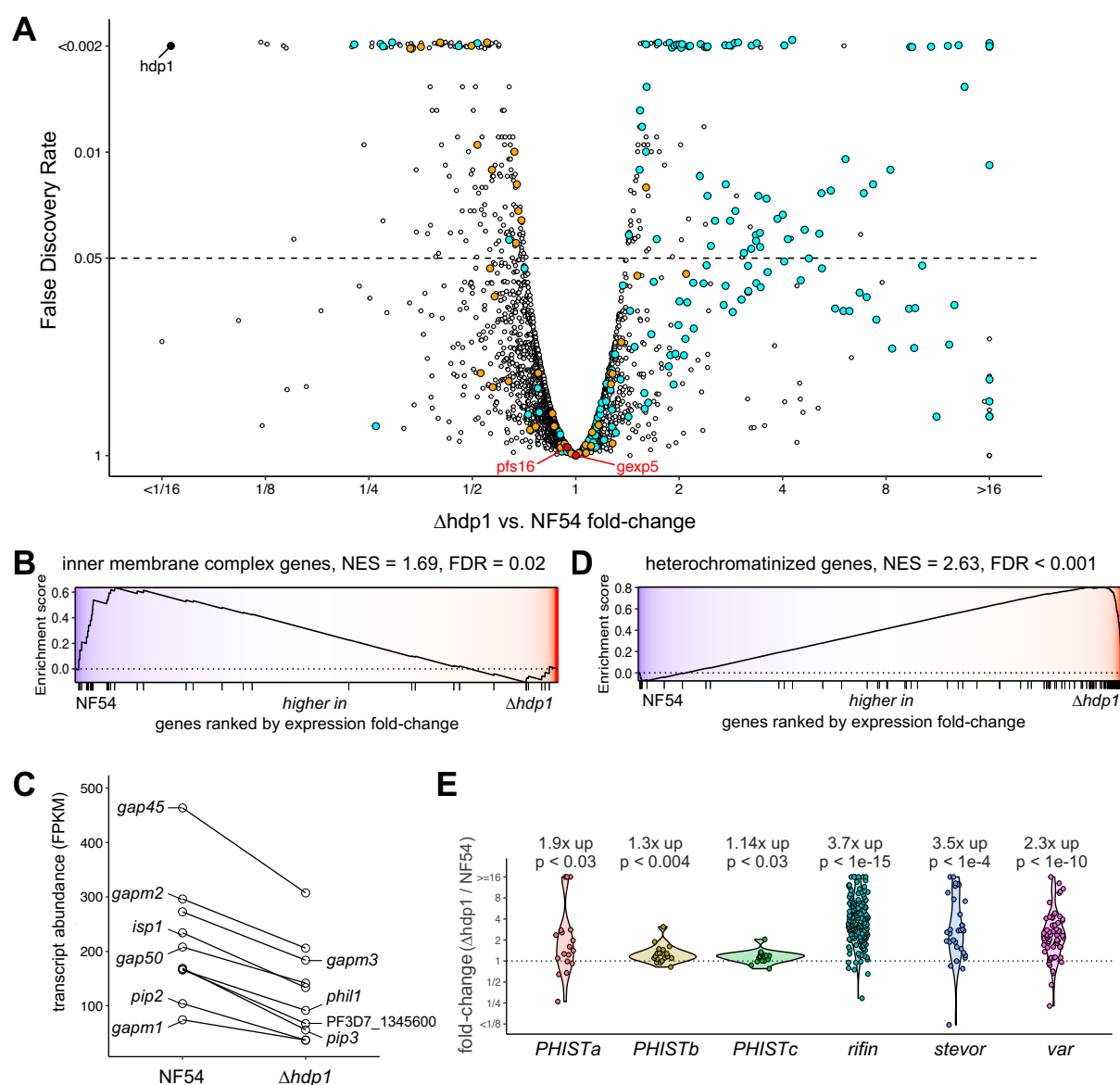
Fig. 3: Disruption of HDP1 results in leaky expression of heterochromatin-associated genes and reduced expression of inner membrane complex genes in early gametocytes. (A) Genome-wide comparison of differential gene expression in \Delta hdp1 and parental NF54 gametocytes on day 2 of gametocytogenesis (stage I, n=2). hdp1 (solid black), heterochromatin-associated genes (cyan), IMC genes (orange) and the two canonical early gametocyte markers, pfs16 and gexp5 (red) are highlighted. Gene set enrichment analysis (GSEA) indicated significant downregulation of IMC genes (B-C) and global upregulation of heterochromatin associated genes (D-E). For the gene enrichment plots (B & D) genes with detectable expression are ranked along the x-axis by expression fold-change, from highest in NF54 to highest in \Delta hdp1 , with tick marks indicating the ranks of inner membrane complex or heterochromatinized genes, respectively. The y-position of the line indicates the enrichment score as a sliding-window for genes that are highest in NF54 to those highest in \Delta hdp1 . The overall normalized enrichment score (NES) and false discovery rate (FDR) for each gene set are shown above each plot. Geometric mean fold-changes and p-values (two-sided, one sample t-test) are indicated in (E).
