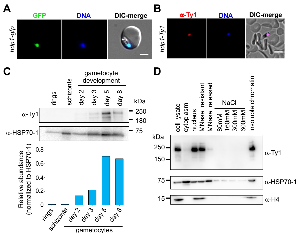
Fig. 2: HDP1 is a chromatin-associated protein nuclear protein expressed in gametocytes. (A) Live-cell fluorescence microscopy of hdp1-gfp gametocytes on day 5 of maturation stained with the DNA dye Hoechst33342 (blue). Scale Bar: 3 \mu m. Representative of n=2. (B) Immunofluorescence microscopy of hdp1-Ty1 gametocytes on day 5 of maturation co-stained with anti-Ty1 antibodies (red) and Hoechst33342 (blue). Scale Bar: 5 \mu m. Representative of n=2. (C) Western blotting of parasite lysates in asexual stages and during gametocyte maturation shows HDP1 is expressed during the stages of gametocytogenesis. Representative of n=3. (D) Western blot of cytoplasmic and nuclear extracts of hdp1-Ty1 gametocytes on day 5 of maturation stained with antibodies against the Ty1 epitope tag, the histone H4, and HSP70-1. Representative of n=3
