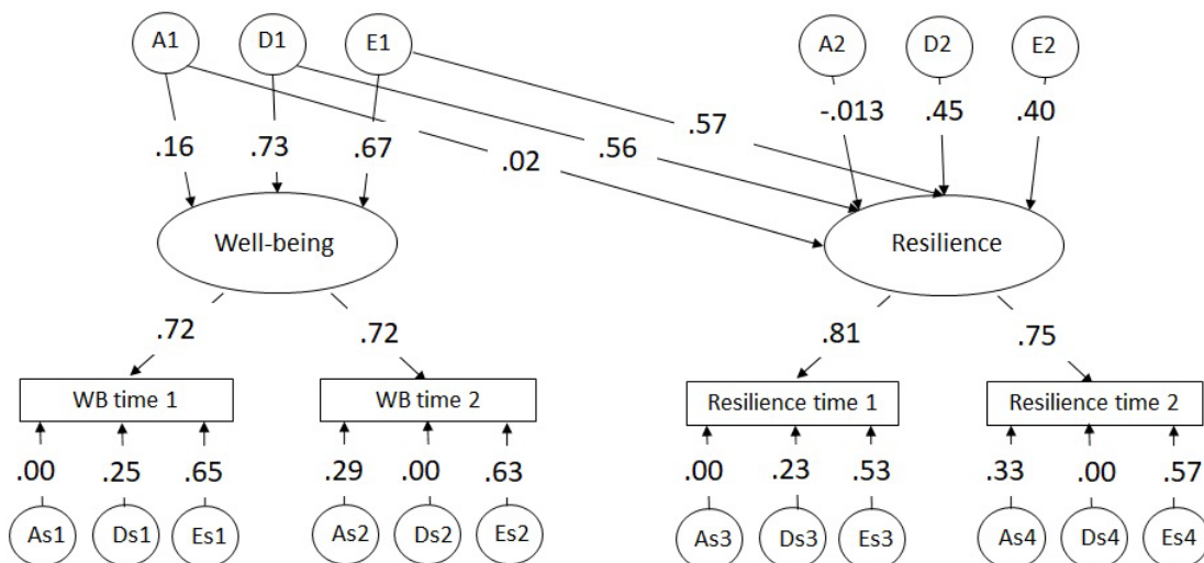
Figure S4. Path estimates of the full common pathway model of resilience and well-being for females and males. WB= well-being, A= common additive genetic effect, E= common unique environmental effects, As= time-specific additive genetic effect, Es= time-specific environmental effect.
