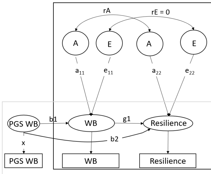
Figure 1. The MR-DoC model. The black box indicates the Direction of Causation model part. The grey box indicates the Mendelian Randomization part. Path g_1 indicates the causal effect, path b_1 indicates the PGS effect on well-being and path b_2 reflects the pleiotropy between well-being and resilience. WB= well-being, A= common additive genetic effect, E= common unique environmental effects, r_A = additive genetic correlation, r_E = environmental correlation.
