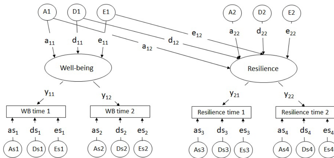
Figure S1. Longitudinal measurement model. WB= well-being, A= common additive genetic effect, E= common unique environmental effects, As= time-specific additive genetic effect, Es= time-specific environmental effect.
