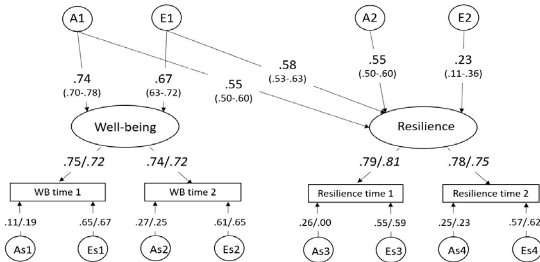
Figure 4. Unstandardized path estimates of the final common pathway model of resilience and well-being. The factor loadings from the common factors to the time-specific factors and the time-specific variance decomposition could not be constrained to be equal for females and males, indicated by estimates for females/males. WB= well-being, A= common additive genetic effect, E= common unique environmental effects, As= time-specific additive genetic effect, Es= time-specific environmental effect.
