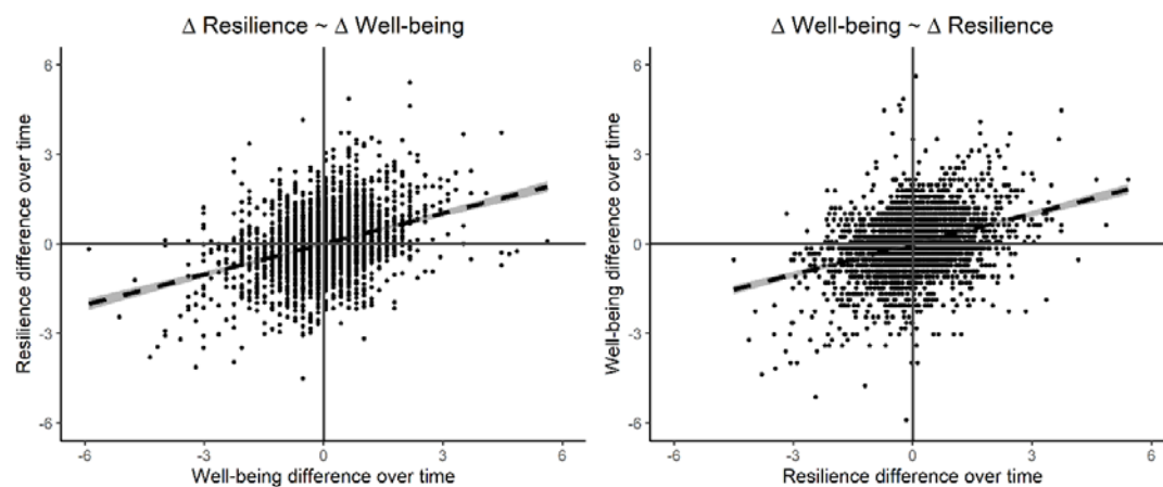
Figure 3. The relation between the within-subject differences over time in resilience and well-being.
