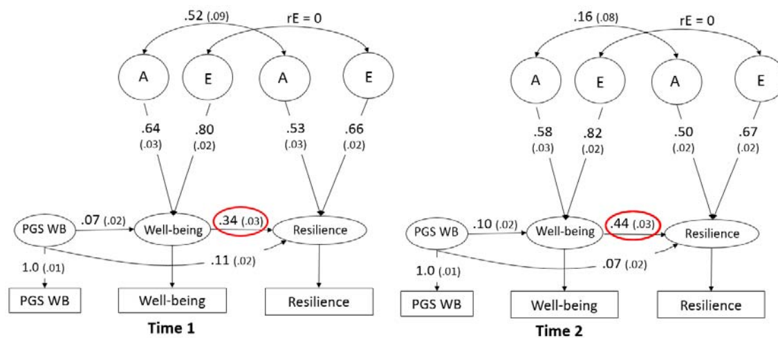
Figure 6. The results of the MR-DoC model. The models show the model with the well-being polygenic score and resilience as the outcome in cross-sectional data from time point 1 and 2 respectively. The causal effects can be seen in the red circle. WB= well-being, , PGS= polygenic score, A= additive genetic effect, E= unique environmental effect, rE= environmental correlation.
