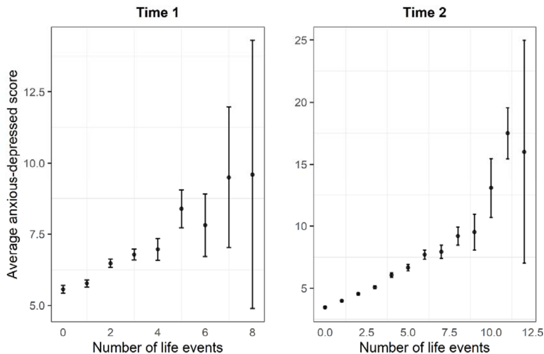
Figure S2. Association between the number of life events and the anxious depressed score.
