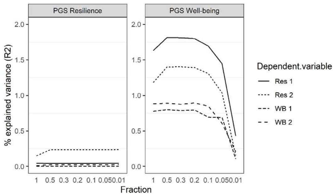
Figure S3. Explained variance by the resilience and well-being PGS for the different fractions of SNPs included.
