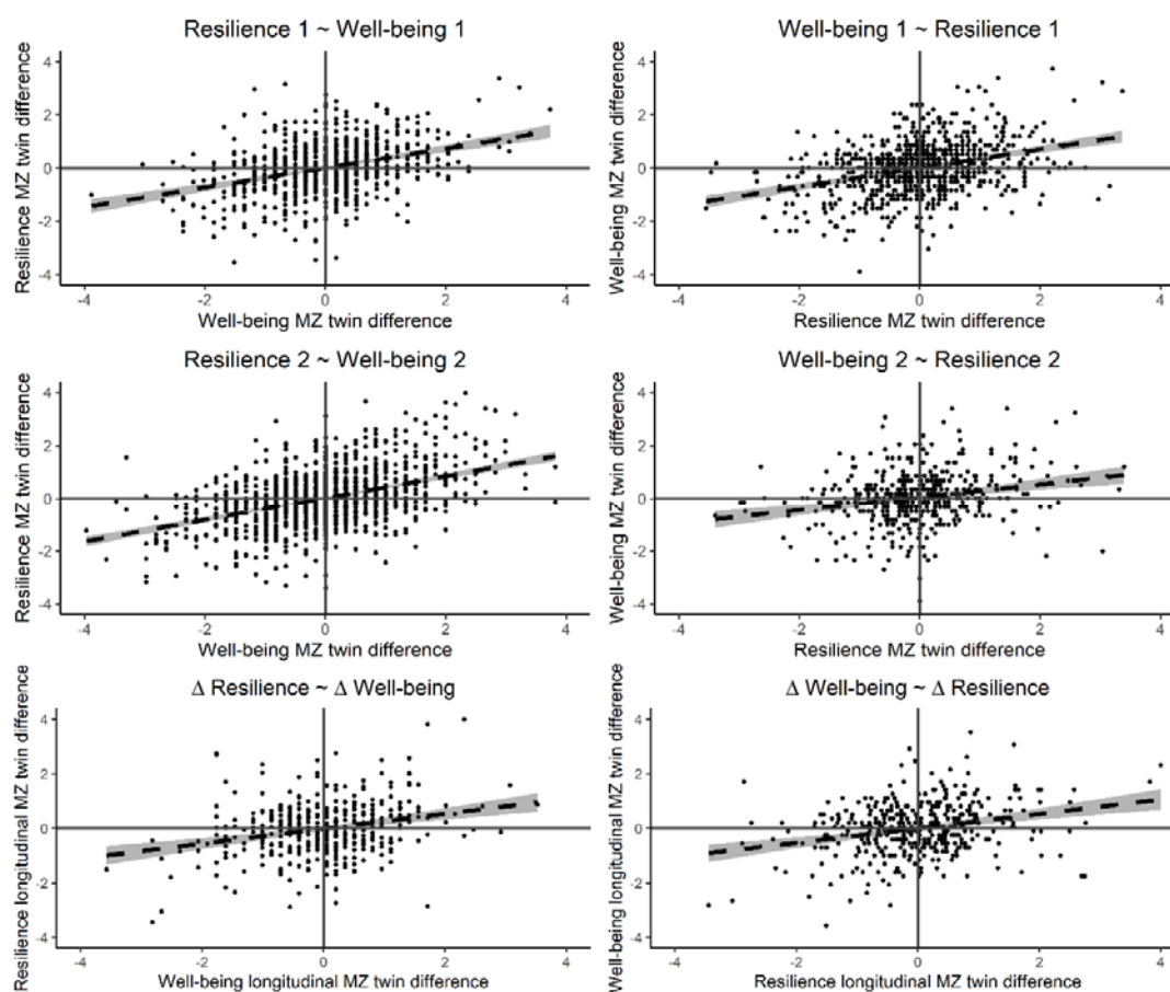
Figure 5. The monozygotic twin differences models. In the left upper panels, the MZ twin difference score of resilience is predicted by MZ twin differences in well-being (cross-sectional, at T1 and T2). In the right upper panels, the MZ twin difference score of well-being is predicted by MZ twin differences in resilience (cross-sectional, at T1 and T2). The lower panel shows the longitudinal association between MZ within-twin pair differences in resilience and well-being.
