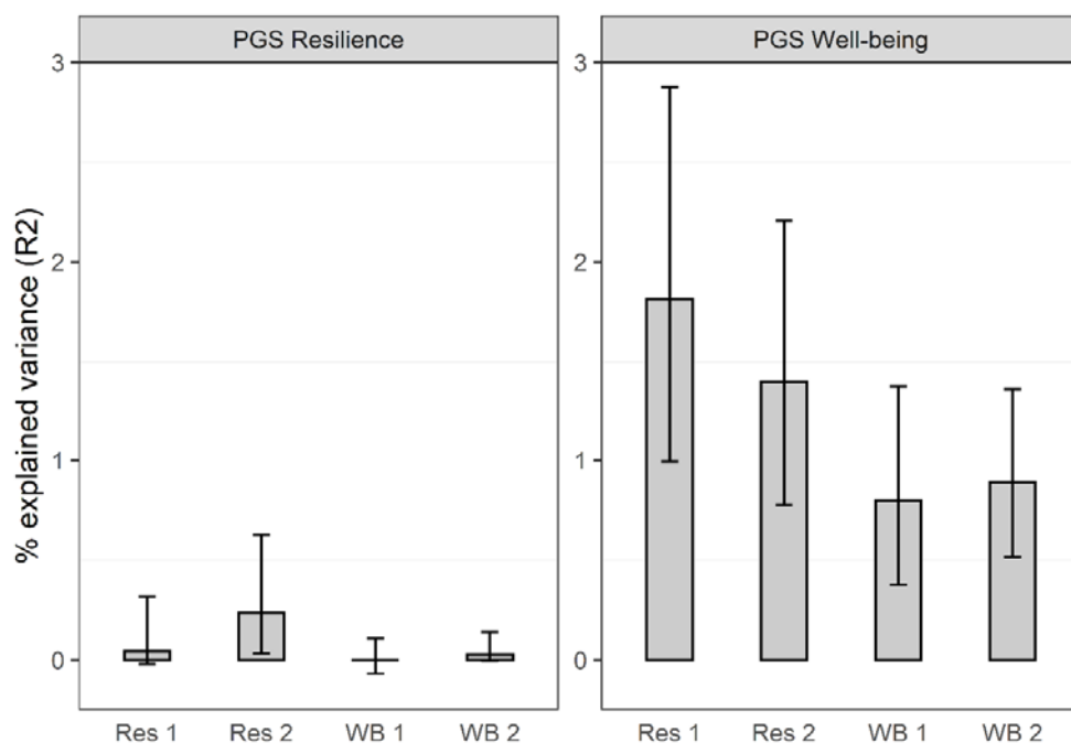
Figure 2. Explained variance in the phenotypic resilience and well-being scores by the polygenic scores (PGS) of resilience (left panel) and well-being (right panel). Res 1= resilience time point 1, Res 2= resilience time point 2, WB 1= well-being time point 1, WB 2= well-being time point 2.
