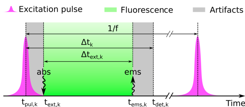
Figure 10: Cartoon of the factors that contribute to the recorded photon arrival times. Here, t_{pul,k} is the time of the pulse's peak. Since pulses last for some time, they may excite the molecules at slightly different times. As such, we denote with t_{ext,k} the absorption time of the molecule triggering the k^{th} detection. Moreover, we denote with t_{ems,k} the emission time of the photon triggering the k^{th} detection. At last, on account of electronics limitations, the detection time, which we denote with t_{det,k} , might be different from t_{ems,k} . Here, the artifacts shown in gray originate from two sources: the left gray-shaded region is due to the width of the pulse which leads to variation in the time of the molecular excitation, and the right gray-shaded region arises from the camera-dependent detection uncertainty. The time during which the fluorophore is excited (fluorescence lifetime) is shown in green.
