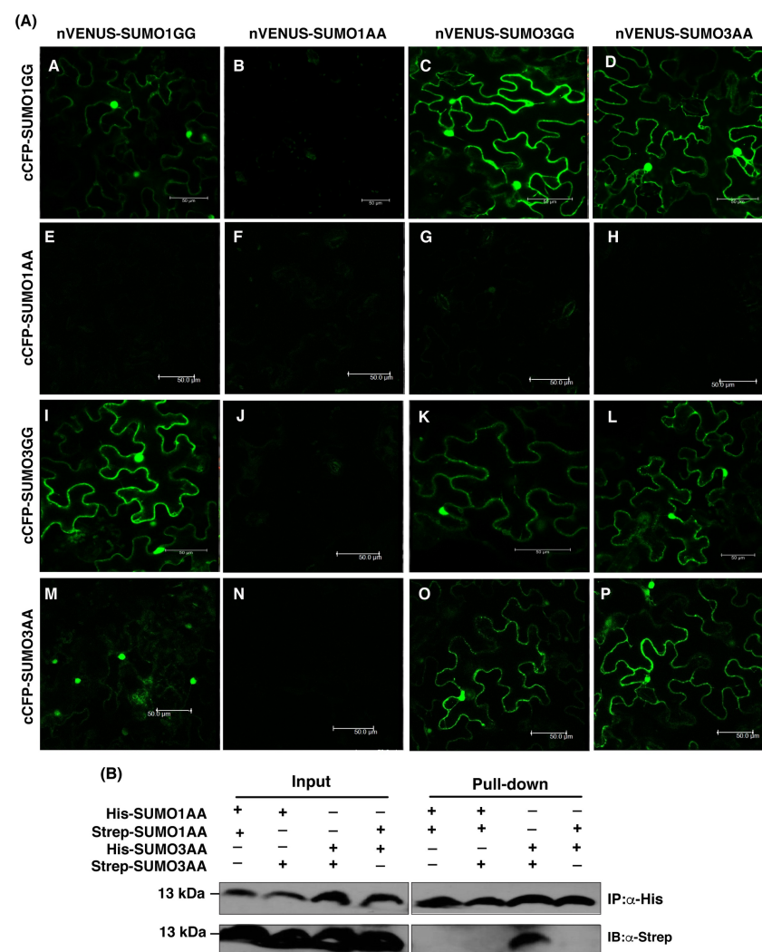
Fig 7: SUMO3, but not SUMO1, can form oligomers. (A) Green fluorescence indicative of YFP reconstitution between BiFC (Bi-molecular Fluorescence complementation) combinations of SUMOylation proficient (GG) or deficient (AA) forms of SUMO1 and SUMO3 isoforms are shown. Agrobacterium GV3101 strains expressing the indicated BiFC constructs were co-infiltrated in expanded N. benthamiana leaves. Infiltrated leaf sections were visualized under a confocal microscope at 2-days post-infiltration (dpi). (Scale bar = 50 \mu m). Images are representative of pattern observed in two independent experiments. (B) In vitro binding assays between SUMO1 and SUMO3 isoforms. His-or Strep-II-tagged SUMO1 or SUMO3 isoform as indicated were expressed in E. coli . Bacterial lysates from indicated combinations were mixed and enriched through the \text{Ni}^{2+} -NTA matrix. Enrichment of the mentioned His-SUMO and the co-eluting isoform was investigated via immunoblotting with anti-His or anti-Strep antibodies, respectively (pull-down panel). The input panel shows the protein levels in the extracts used for the enrichments. Position of protein molecular weight standards (in kDa) are indicated.
