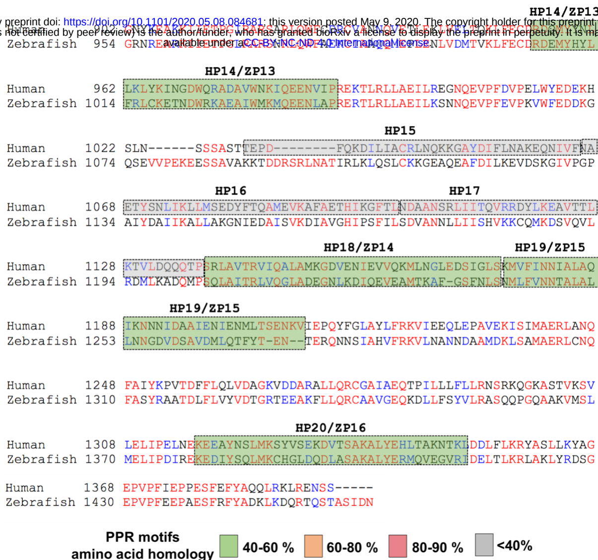
Supplementary Figure 3: Amino acid alignment of LRRPRC human protein with zebrafish Lrrpprc protein. Multiple protein sequence alignment was performed by T-COFFEE multiple sequence alignment webserver. Zebrafish PPR domains were predicted by performing blastp using human PPR domains as the query. The colors of the boxes represent the percentage of homology between the two protein sequences. 16 zebrafish domains were predicted by the homology analysis. Predicted zebrafish mitochondrial targeting sequence is highlighted in blue box (1-77 amino acids). (HP(n): Human PPR domain; ZP(n): Zebrafish PPR domain)
