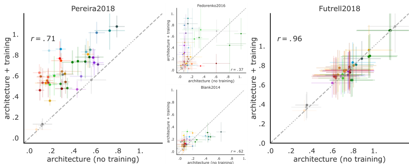
Figure S7: Model architecture alone already yields predictive representations and untrained performance predicts trained performance. In Fig. 5, we showed that untrained models already achieve robust brain predictivity (averaged across the three neural and one behavioral datasets). Here, we show that this relationship also holds for each dataset individually: Pereira2018: p < 0.00001 , Fedorenko2016: p < 0.05 , Blank2014: p < 0.00001 , Futrell2018: p < 0.00001 .
