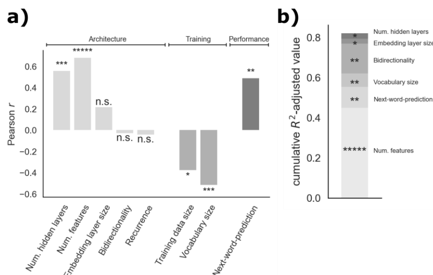
Figure S9: Effects of model architecture vs. training on neural and behavioral scores. a) We compared the effects on neural and behavioral scores (the averaged model score across all four datasets) of three kinds of features: (i) architectural properties, (ii) training-dependent variables, and, for comparison, (iii) performance on the next-word-prediction task examined in the main text (Fig. 3, 4c). b) Alternative combination of predictors with stepwise forward regression model. New predictors are added based on the highest R^2 -adjusted value of the new model, as long as variance increases by adding a new factor (thus excluding training dataset size and recurrence). Significance markers indicate the p-value for significance of adding model terms. For each regression step, we plot the added explained variance (in R^2 -adjusted) of the variable chosen by the model. The overall cumulative R^2 -adjusted value of the selected model is 0.822. As in a), the preferred explanatory variable is the number of features. Stepwise forward regression based on significance leads to the same model-choice. Note that, as above, t5-11b is excluded for regression based on next-word-prediction, and multilingual models are excluded for regression on training size.
