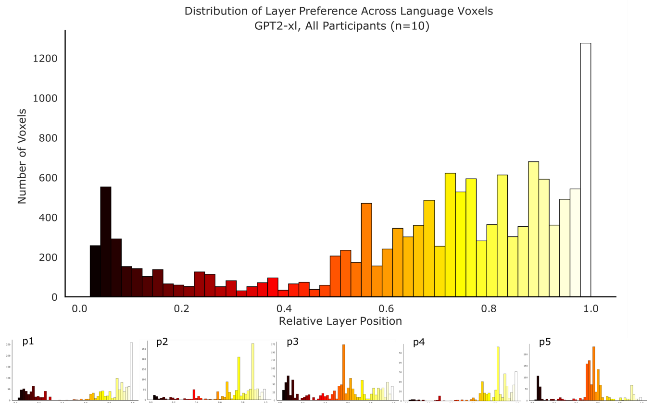
Figure S11: Distribution of layer preference (best performing layer) per voxel for GPT2-xl for Pereira2018. A per-voxel per-participant raw predictivity value was obtained in the language network by computing the mean over cross-validation splits and experiments. For each voxel, the layer with the highest predictivity value was estimated as the “preferred” layer (argmax over layer scores). As in the main analyses, the voxels in the language network were included. Zero on the x-axis corresponds to the embedding layer of the model. The upper plot is averaged across all participants in Pereira2018 (n=10). The lower panel shows the participant-wise layer preference for five representative participants. Across participants, most voxels show the highest predictivity value for later layers of GPT2-xl. Within participants, the layer preference across voxels varies but is often clustered around particular layers. Investigations of how predictivity fluctuates across model layers, and/or between the language network and other parts of the brain, is left for future work.
