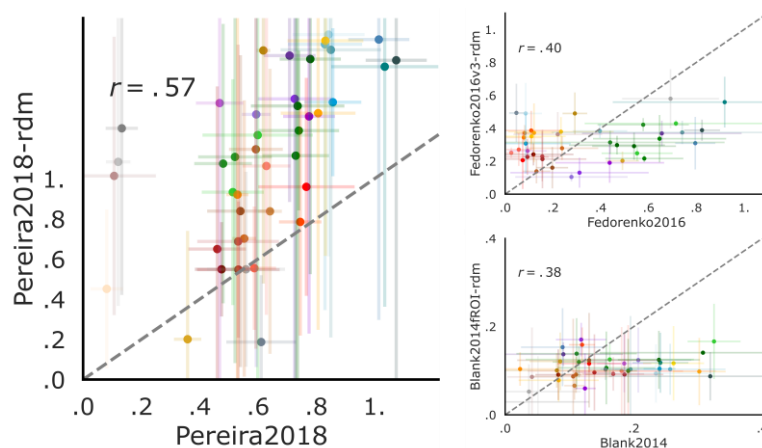
Figure S2: Scores generalize across metrics. Model scores on each dataset generalize across different choices of a similarity metric; here we plot the predictivity metric used in the manuscript on the x-axis against a model-to-brain similarity metric based on representational dissimilarity matrices (RDMs) between models and neural representations on the y-axis. Like in the predictivity metric, stimuli along with corresponding model activations and brain recordings were split 5-fold but we then only compared the respective test splits given that the RDM metric does not employ fitting. Specifically, we followed (Kriegeskorte, 2008) and computed the RDM for each model's activations, and a separate RDM for each brain recording dataset, based on 1 minus the Pearson correlation coefficient between pairs of stimuli; then, we measured model-brain similarity via Spearman correlation across the two RDMs' upper triangles. The RDM score for one model on one human dataset is then the mean over splits. We ran each model and compared resulting scores with the primarily used scores from the predictivity metric. Correlations for models' scores between the predictivity and the RDM metrics are: Pereira2018 r = .57 , p < 0.0001 ; Fedorenko2016 r = .40 , p < .01 ; Blank2014 r = .38 , p < .05 .
