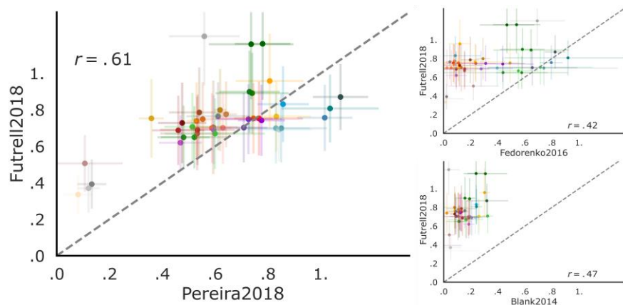
Figure S6: Models' neural predictivity for each dataset is correlated with behavioral predictivity. In Fig. 4b, we showed that the models' neural predictivity (averaged across the three neural datasets: Pereira2018, Fedorenko2016, Blank2014) correlates with behavioral predictivity. Here, we show that this relationship also holds for each neural dataset individually: Pereira2018: p < 0.0001 , Fedorenko2016: p < 0.01 , Blank2014: p < 0.01 .
