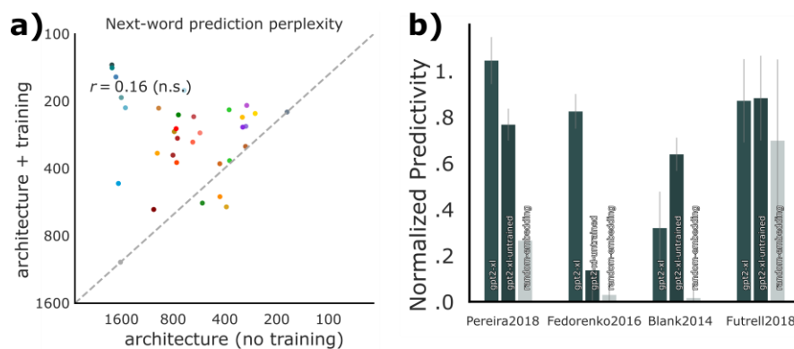
Figure S8: Performance of models with random weights depends on architecture. a) The relationship between model performance with vs. without training on the wikitext-2 next-word-prediction task. Consistent with model performance with vs. without training on neural and behavioral datasets (Fig. 5), untrained models perform reasonably well. Training improves scores by 80% on average, and most prominently for GPT models, in teal (where the quality of the training data is optimized; see Computational models in Methods ). b) Neural and behavioral scores of GPT2-xl, the best-performing model, with vs. without training, and of a random embedding of the same size. Embedding size alone is not sufficient: a random embedding matched in size to GPT2-xl scores worse than untrained GPT2-xl in all four datasets (3 neural, and 1 behavioral). These results suggest that model architecture critically contributes to model-to-brain and model-to-behavior fits.
