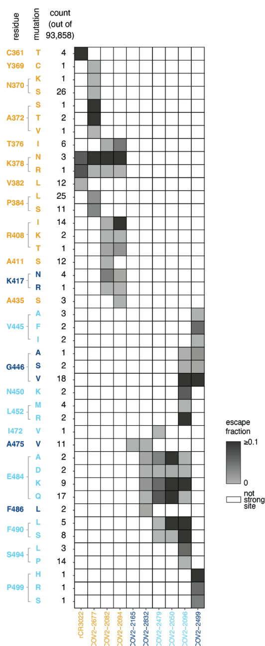
Figure S4. Variation at sites of antibody escape among currently circulating SARS-CoV-2 viruses. Table shows all RBD mutations sampled among sequences in GISAID as of 6 September 2020 at sites of escape from at least one antibody. Cells are colored by escape fraction of the individual circulating mutant for each antibody: white cells indicate sites that are not sites of escape from an antibody; for sites of escape, per-mutation escape fraction is colored from light to dark gray, with any mutation conferring >0.1 escape fraction colored equally dark. Sites are in orange for the core RBD, light blue for the RBM, and dark blue for ACE2 contact residues. Antibodies are colored according to where the majority of their sites of escape fall. These per-mutation counts are collapsed into the site-wise table presented in Figure 5A.
