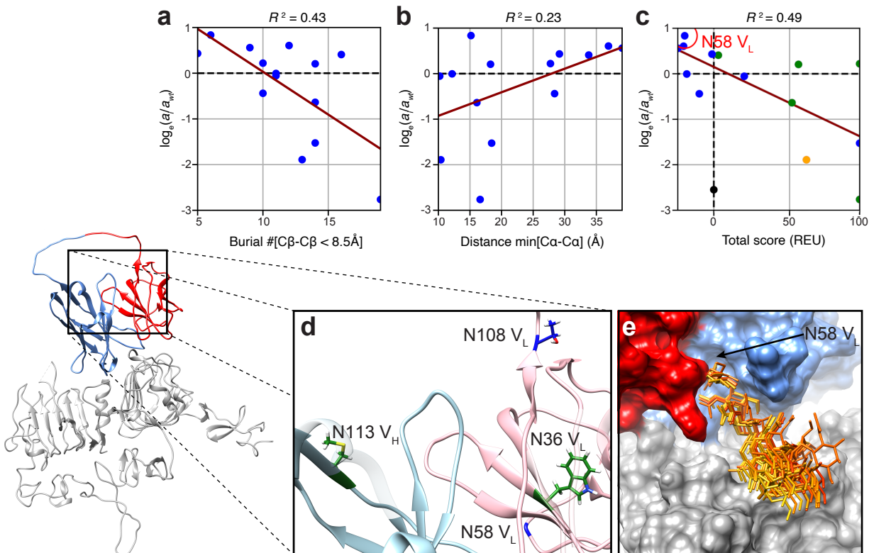
Figure 6: Quantitative analysis of scFv-HER2 variants. The structure of scFv-HER2 V_L (red) and V_H (blue) domains in complex with HER2 protein (gray) is shown at bottom left. Regression analyses of log activity ratio (glycosylated / wild-type) versus (a) burial of sequon substitution site, (b) distance of closest HER2 residue from the sequon substitution site, and (c) total Rosetta score. In all three panels, the dark red lines are the respective regression lines. Colors of dots in (c) show the respective secondary structure of the sequon substitution site. Orange, green, and blue correspond to \alpha -helix, \beta -strand, and loop regions, respectively. N58 V_L (red circle) has the highest glycosylated binding activity increase and is discussed in the text. (d) Wild-type representation of sites used for analysis of sequon substitution (36 V_L , 108 V_L , and 113 V_H ) and glycosylation (58 V_L ). Side-chain colors reflect their respective secondary structures. (e) Glycan arrangement (orange sticks) from eight low energy conformations of glycosylated N58 V_L variant of scFv-HER2, revealing possible glycan-HER2 interaction responsible for binding activity improvement.
