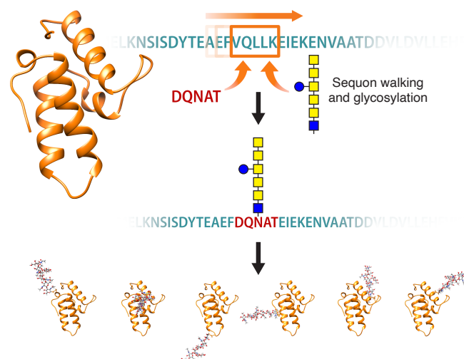
Figure 1. Fine-mapping the effects of glycan installation. Schematic of shotgun scanning glycomutagenesis (SSGM), a glycoprotein engineering method based on combinatorial protein libraries in which glycosylation “sequon walking” is used to introduce an acceptor site at every possible position along the protein backbone. Note that the multi-residue nature of a sequon (e.g., N-X-S/T or D/E-X 1 -N-X 2 -S/T where X, X 1 , X 2 ≠ P) necessitates insertion or replacement of up to four additional amino acid substitutions at each position. The resulting library is expressed in glycoengineered bacteria, providing an opportunity for each library member to be expressed and glycosylated in a manner that is compatible with high-throughput screening via glycoSNAP to interrogate the glycosylation phenotype of individual variants. By integrating bacterial SSGM libraries with multiplexable assays, the biochemical and biophysical properties of each glycovariant can be individually interrogated.
