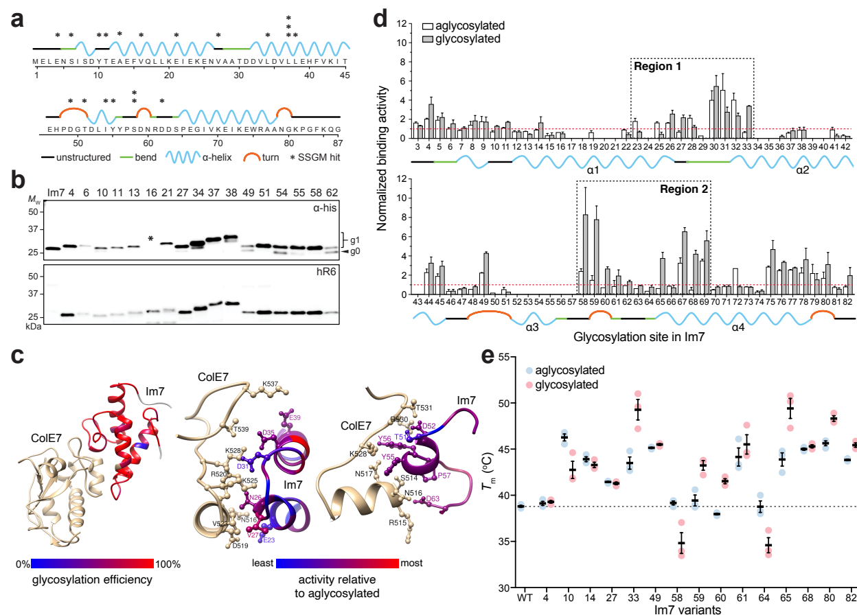
Figure 3. Exhaustive N-glycosylation of bacterial Im7 and its consequences. (a) Primary sequence and predicted secondary structure for E. coli Im7 immunity protein. Asterisks denote location and frequency of glycosite hits isolated using SSGM. Predicted structures adapted from PDB ID 1AYI. (b) Immunoblot analysis of supernatant fractions from CLM24 cells carrying plasmids encoding YebF-Im7 fusions with sequon mutations at indicated position and requisite N-glycosylation machinery. Blots were probed with anti-polyhistidine antibody (α-His) to detect acceptor protein (top panel) and hR6 serum against the glycan (bottom panel). Markers for aglycosylated (g0) and singly glycosylated (g1) forms of acceptor proteins are indicated at right. Molecular weight ( M_w ) markers are indicated at left. Asterisk indicates construct with mutation that introduced stop codon just before 6xHis tag, preventing α-His detection. Results are representative of at least three biological replicates. (c) Mapping of in vivo glycosylation efficiency onto three-dimensional structure of Im7 in complex with ColE7 (left). Heatmap analysis of the glycosylation efficiency was determined based on densitometric quantification of the percent glycosylated (defined as g1/[g0+g1] ratio) for each acceptor protein in the anti-His immunoblot. Detailed interactions between ColE7 and Im7, highlighting sidechains of Im7 in the regions of α1-loop12-α2 (residues 19-39; middle) and loop23-α3-loop34 (residues 46-63; right). Heatmap analysis of change in binding activity was determined by normalizing activity measured for glycosylated sequon variant by aglycosylated counterpart. (d) Binding activity of glycosylated (gray bars) and aglycosylated (white bars) YebF-Im7 variants recovered from supernatants was measured by ELISA with ColE7 as immobilized antigen. All data were normalized to binding activity measured for aglycosylated YebF-Im7 lacking a sequon (wt), such that values greater than 1 (denoted by dashed red line) indicate enhanced binding activity relative to wt Im7. Dashed boxes correspond to two regions (Region 1: residues 23-33; Region 2: residues 58-69) that have many variants with increased activity. Data are average of three biological replicates and error bars represent standard deviation of the mean. (e) DSF analysis of 15 most active YebF-Im7 variants with and without glycosylation. T_m calculated as midpoint of thermal transition between native and unfolded states. Dashed line indicates T_m for wt YebF-Im7 ( 38.6 \pm 1.0 °C). Black bars are average of three independent replicates with error bars reported as standard error of the mean.
