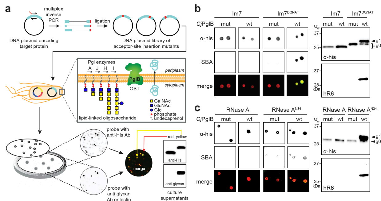
Figure 2. Construction and interrogation of SSGM libraries. (a) Schematic of SSGM library construction using multiplex inverse PCR approach. The resulting plasmid library, encoding acceptor protein variants with glycosite substitutions at every possible position, was used to co-transform E. coli strain CLM24 along with two additional plasmids encoding the requisite N -glycosylation machinery from C. jejuni . The resulting bacterial library was plated on solid agar, after which colonies and their secreted glycoproteins were replica plated on nitrocellulose membranes as described in the text. (b) Immunoblot analysis of acceptor proteins in colony secretions (left) and extracellular supernatant fractions (right) derived from E. coli CLM24 carrying a plasmid encoding either YebF-Im7 or YebF-Im7 DQNAT along with plasmids encoding N -glycosylation machinery with either wild-type CjPglB (wt) or an inactive mutant (mut). (c) Same as in (b) but with YebF-RNase A and YebF-RNase A N34 in colony secretions (left) and periplasmic fractions (right). Blots were probed with anti-polyhistidine antibody (α-His) to detect acceptor protein and SBA or hR6 serum to detect the glycan. Bottom color panels in (b) and (c) depict overlay of α-His and SBA blots (merge). Arrows denote aglycosylated (g0) and singly glycosylated (g1) forms of YebF-Im7 DQNAT or YebF-RNase A N34 . Molecular weight ( M w ) markers are indicated at left. Results are representative of at least three biological replicates.
