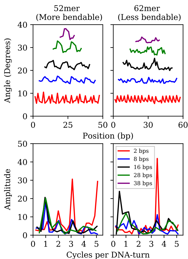
Figure 6: Top: length-evolution of bending angle profiles along the sequence for the most (left) and less (right) curved oligomers (52mer and 62mer, respectively). Bottom: frequencies (in cycles per DNA-turn) obtained after applying fast Fourier transforms to bending positional data
