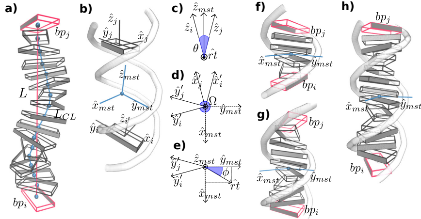
Figure 1: Schematic diagrams of the algorithm implemented in SerraNA for calculating the geometric parameters at different fragment lengths. (a) Vertical displacement is characterized by end-to-end distance (in red) and contour length (in blue). (b) Twist and bend angles between bp i and j are obtained via the mid-base triad ( T_{mst} ) positioned at the mid-point. (c) Bending angle \theta and bending axis \hat{r}_t are defined by directional vectors \hat{z}_i and \hat{z}_j . Co-planar vectors \hat{y}'_i , \hat{y}'_j , \hat{x}_{mst} and \hat{y}_{mst} define twist angle \Omega (d) and roll and tilt bending angles (e). (f)-(h) T_{mst} between bp (in red) separated by 4, 8 and 12 bp, respectively. Roll and tilt consist on bending towards grooves and backbone, respectively, at the fragment midpoint for the different sub-fragment lengths. Angles and T_{mst} are highlighted in blue.
