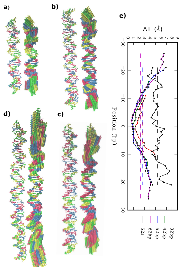
Figure 5: (a)-(d) 32mer, 42mer, 52mer and 62mer averaged structures together with the corresponding end-effect essential modes. (e) Molecular position dependence of end-to-end distance local increments ( \Delta L ) caused by end-vibrational modes from relaxed simulations and by the 52 bp pulling simulation with a maximum extension of 5% (52s), using in all cases sub-fragments of 5 bp length.
