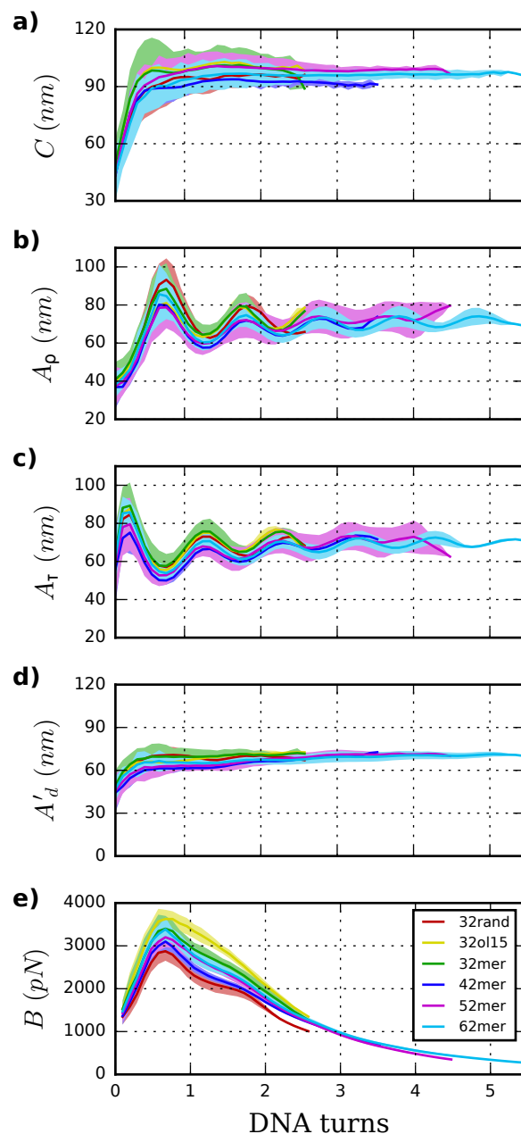
Figure 3: Elastic constants associated with twist ( C ), roll ( A_\rho ), tilt ( A_\tau ) and stretch ( B ) obtained through the inverse-covariance matrix method at different lengths, together with the dynamic persistence length ( A'_d ) obtained via A_\rho and A_\tau combination (see text for more details). Values reported here are averages over all possible sub-fragments with a particular length, discarding the ten longest stretches, and the corresponding standard deviations are given as shade areas.
