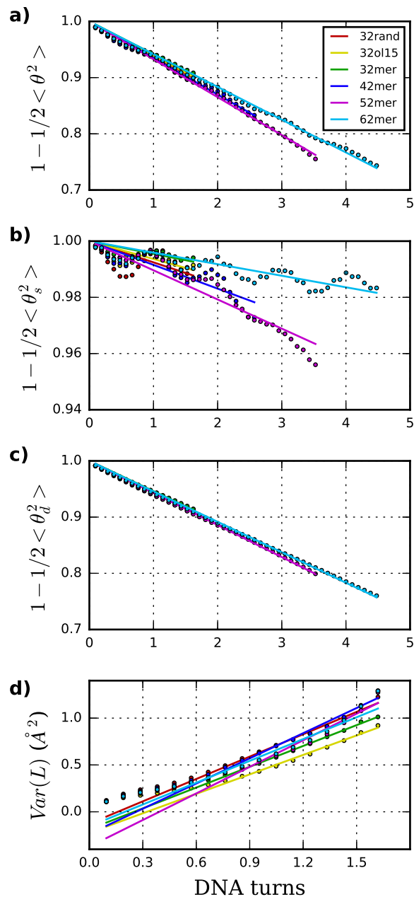
Figure 4: (a)-(c) Persistence length ( A ) together with its static ( A_s ) and dynamic ( A_d ) contributions are obtained through the linear fit of directional decays associated to \langle \theta^2 \rangle , \langle \theta_s^2 \rangle and \langle \theta_d^2 \rangle , respectively. Values reported here are averages over all possible sub-fragments at a particular length, discarding ten longest lengths. (d) Stretch modulus ( B ) is obtained through linear fit of end-to-end partial variance using central 18mer.
