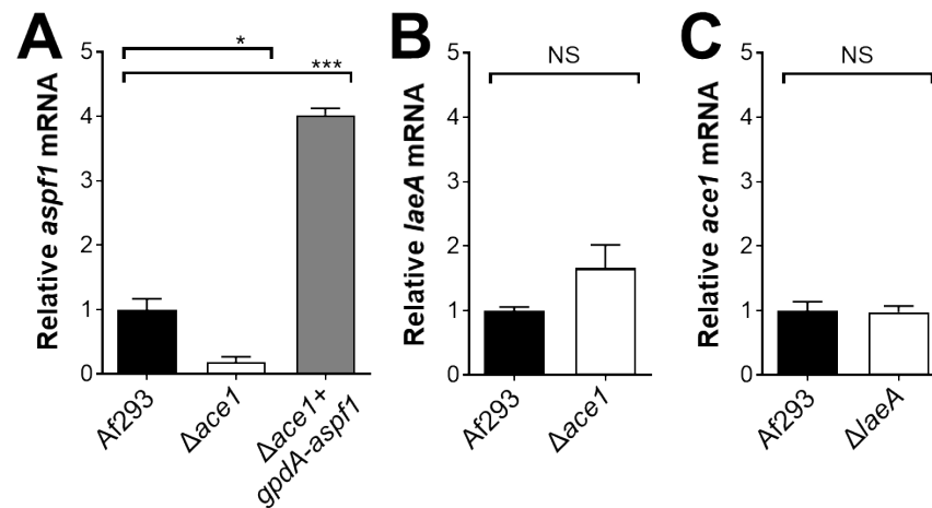
Fig 7. qPCR verification of transcriptional profiling results. Real-time PCR analysis of the relative transcript levels of aspf1 (A), laeA (B), and ace1 (C) in the indicates strains. The organisms were grown in AMM with low nitrogen and low zinc. Results are the mean \pm SD of 3 biological replicates. *, P < 0.05 ; ***, P < 0.001 ; NS, not significant.
