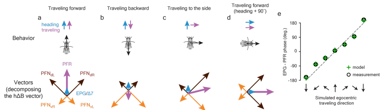
Extended Data Figure 6 | A five-vector model for building the PFR traveling-direction signal. PFRs receive h \Delta B input and thus they can be modeled to receive PFN_v and PFN_d vector input, disynaptically, through the h \Delta B route. PFRs also receive direct PFN_d monosynaptic input in the fan-shaped body and direct EPG/ \Delta 7 monosynaptic input in the bridge. As such, one can model PFR cells as receiving five vector inputs: two PFN_v vectors whose magnitude is regulated by the PFN_v \rightarrow h\Delta B \rightarrow PFR pathway exclusively, two PFN_d vectors whose magnitude is regulated by the PFN_d \rightarrow h\Delta B \rightarrow PFR pathway augmented by additional, direct, monosynaptic inputs from PFN_d s to PFRs, and one EPG/ \Delta 7 vector input that arrives to the PFRs in the bridge. The weight of the EPG/ \Delta 7 in our models always turns out to be small and thus that vector is depicted with a short blue arrow of unchanging length in the diagrams. a , When a fly travels forward, both PFN_d vectors are long and both PFN_v vectors are short, leading the sum of the five vectors, i.e., the PFR (purple) vector, to point forward (i.e., in the fly's heading direction). b , When a fly travels backward, both PFN_d vectors are short and both PFN_v vectors are long, leading the sum, i.e., the PFR (purple) vector, to point backward. c , When a fly travels rightward, the right-bridge PFN_d vector and the left-bridge PFN_v vector are longer than their counterparts on the opposite side of the bridge, leading the sum, i.e., the PFR (purple) vector, to point rightward. Because PFRs receive—in addition to their h \Delta B inputs—direct, EPG/ \Delta 7 input in the bridge and PFN_d input in the fan-shaped body, these additional inputs (if functionally relevant) will tend to bias the PFR traveling direction signal to the front. Indeed, in fitting the PFR data, our model gave these inputs (particularly the additional PFN_d input) functional weight because, empirically, we observed that the PFR bolus is indeed commonly skewed to the frontal direction (Figure 1i; PFR bolus position is consistently biased toward the horizontal zero line in cases where presented optic flow that simulated flies to be traveling sideways, \pm 60^\circ and \pm 120^\circ ). While we do not yet functionally understand why PFRs incorporate a frontal skew to their traveling-direction signal, this skew is why the purple, PFR, summed vector points slightly upward here. d , Same as panel a, but after the fly has turned clockwise by 90^\circ , which shifts the whole reference frame by 90^\circ because both the PFN_d and PFN_v activities are linked to the EPG bolus, which rotates when the fly turns. e , There is a good correspondence between the measured deviation of the PFR phase from the EPG phase (as a function of the optic-flow direction presented) in Figure 1i (circles) and the deviation predicted by our formal model (plus signs). See Methods for details.
