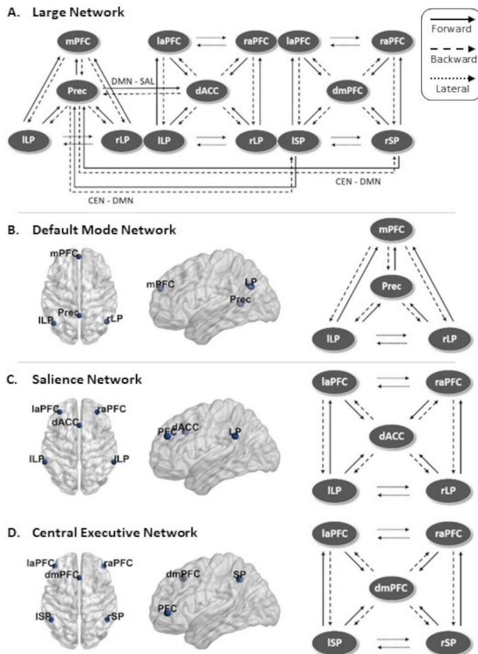
Figure 1. Full model schematics and node locations. A. Schematic view of the large DCM model consisting of the 14 nodes and connections combining three RSNs. Inter-RSN connections were specified between PCC/precuneus and bi-lateral superior parietal nodes, and between PCC/precuneus and anterior cingulate cortex. B-D. Location of the nodes and the schematic representation of the full model for DMN, SAL, and CEN, respectively.
