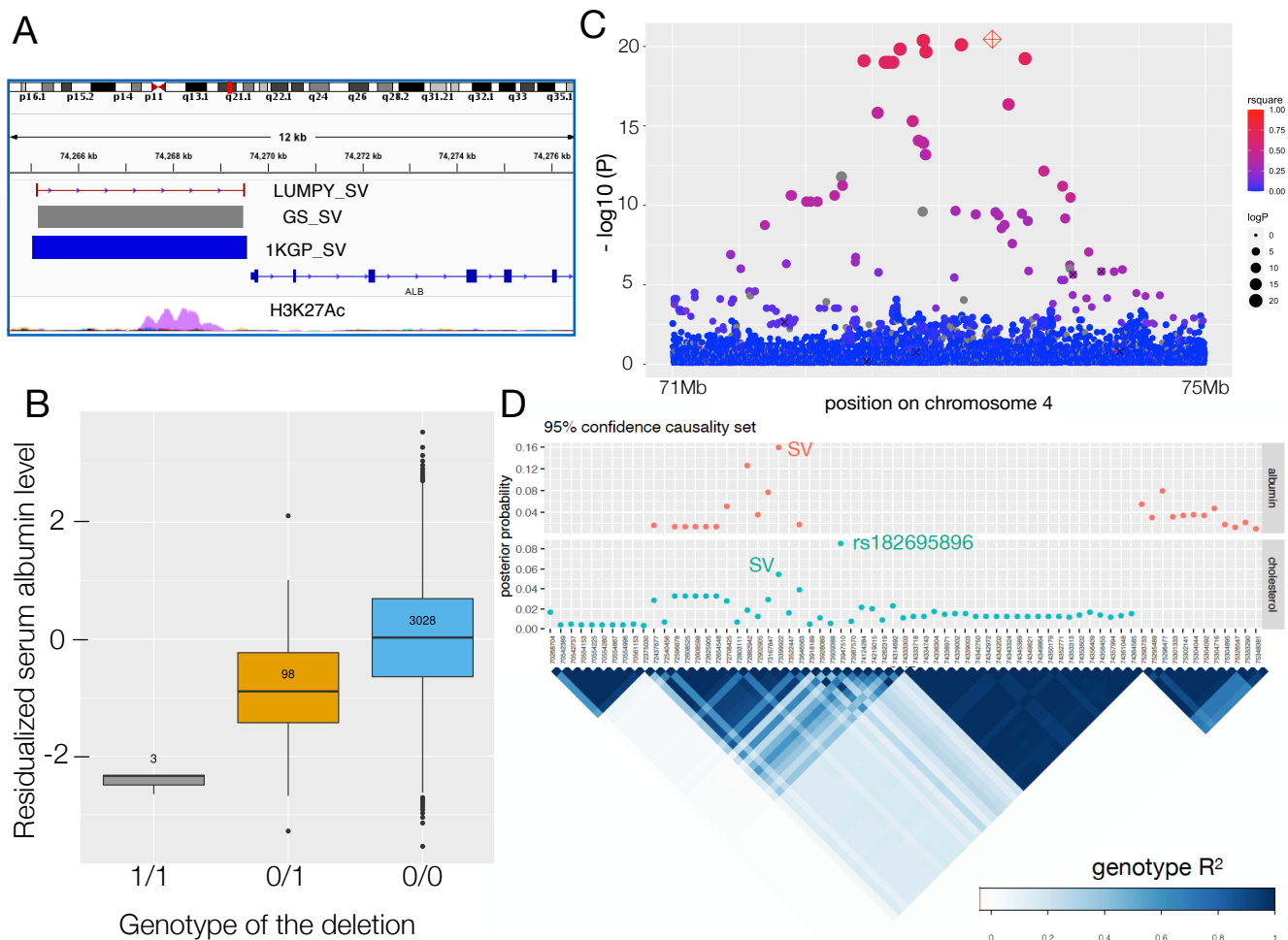
Figure 3. The ALB promotor deletion associated with serum albumin level and cholesterol traits
