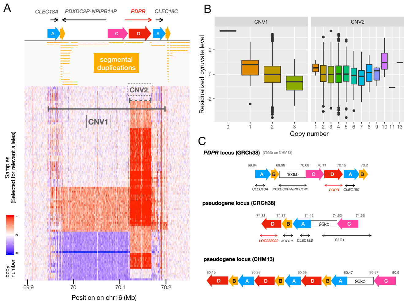
Figure 4. The multi-allelic CNV at the PDPR locus affecting pyruvate and alanine.
