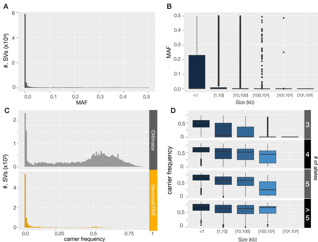
Figure 2. Frequency distribution of the high-confidence SVs
