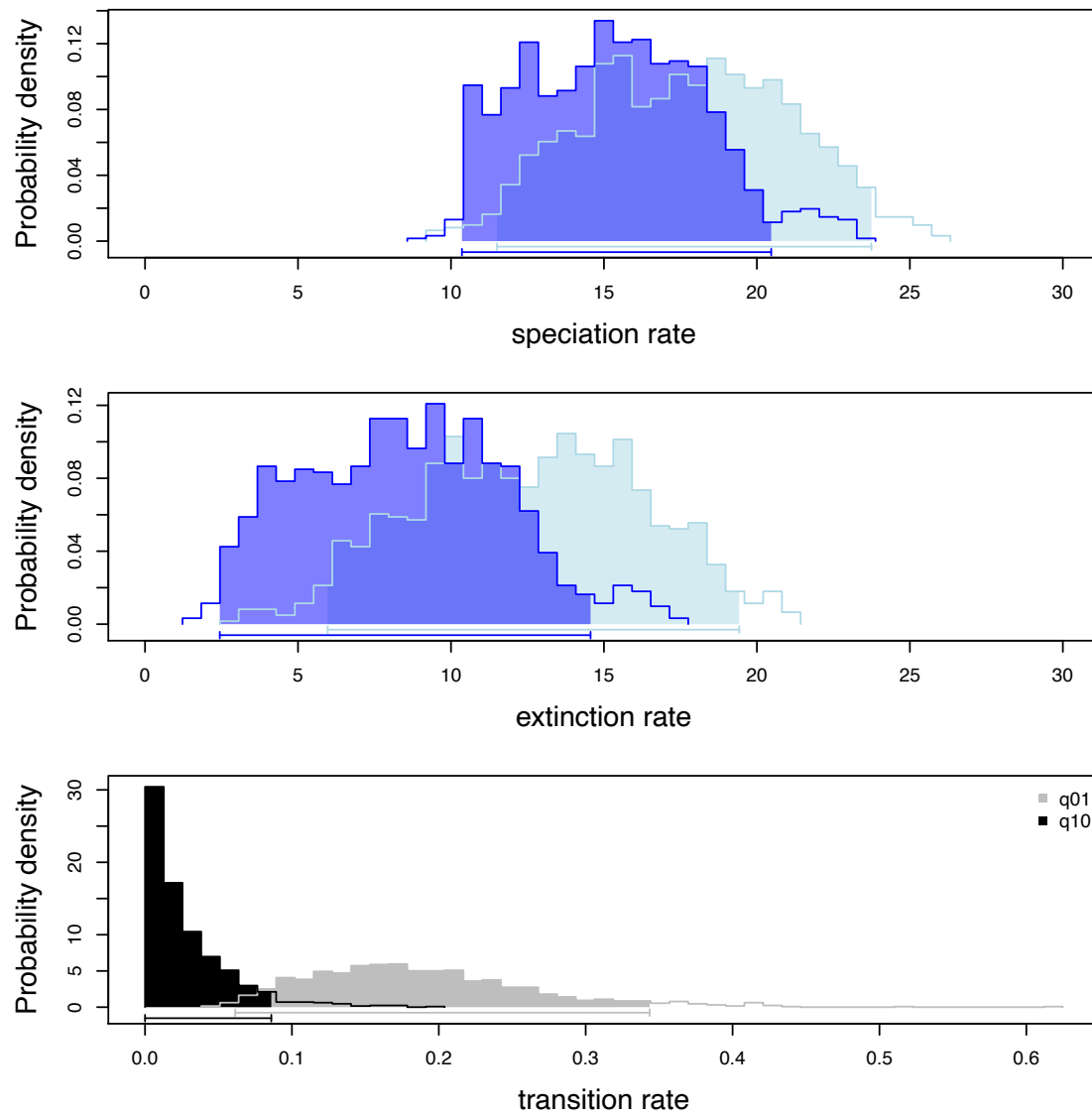
Fig. 4 Parameter estimates from BiSSE analyses. Panels show the density of the posterior probabilities of speciation and extinction rates for anascan (light blue) versus ascophoran (blue), estimated from the global ML tree (see Supplementary Fig. S6 for Bayesian interpretation). Transition rates are also shown, where the transition from ascophoran to anascan is skewed towards zero, supporting the ancestral state reconstruction analyses.
