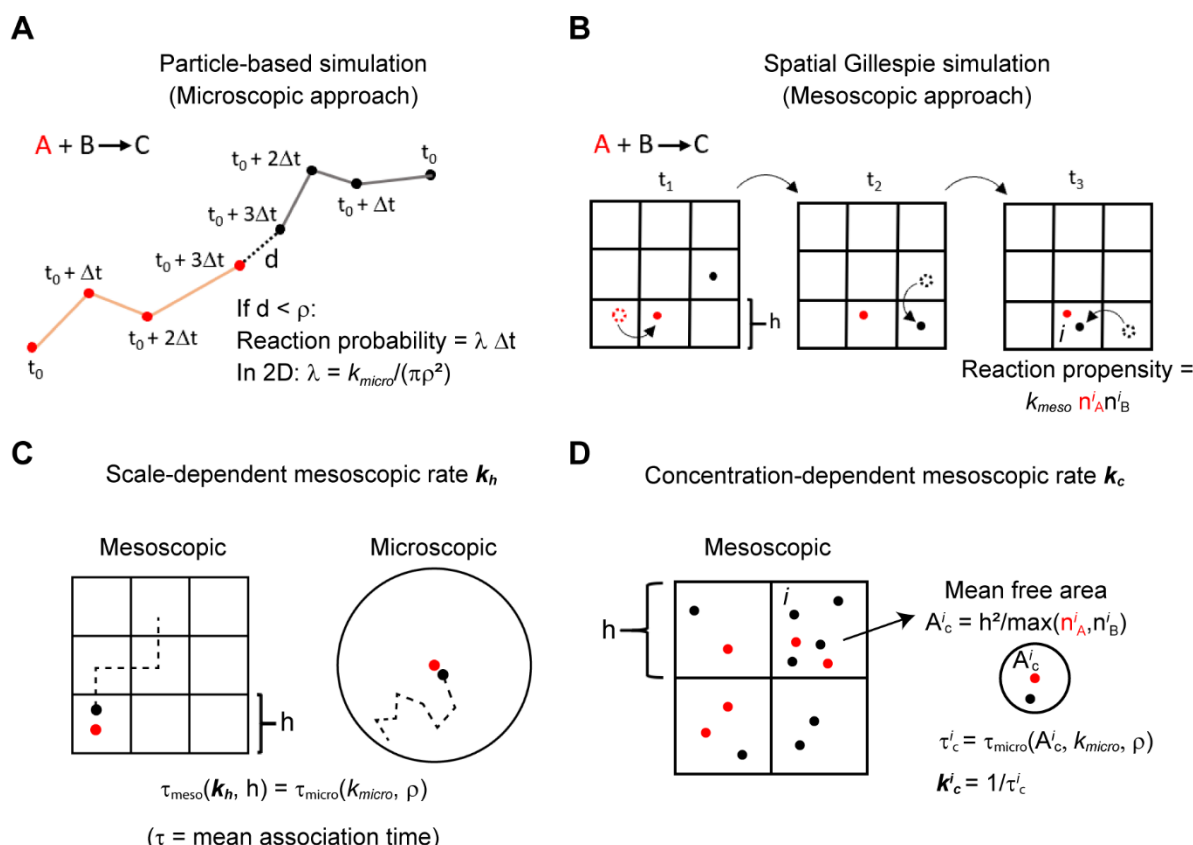
Figure 1. Schematic of the simulation of a generic bimolecular reaction A + B \rightarrow C using a particle-based method and the spatial Gillespie approach. In the particle-based simulations (A) molecules undergo a random walk in continuous space and discrete time intervals \Delta t . If a pair of reacting molecules are within a distance \rho characteristic of their size, they react with probability \lambda \Delta t during an interval \Delta t . In the spatial Gillespie approach (B), the domain is discretized using a grid, here with square elements of size h . Molecule jumps to adjacent grid elements and reactions take place sequentially at random times as a realization of the reaction-diffusion master equation. The propensity of a reaction within a grid element i is proportional to the number of molecules ( n_A^i, n_B^i ) and a mesoscopic rate constant k_{meso} . (C) By setting k_{meso} equal to the scale-dependent mesoscopic rate k_h , the mean association time of two molecules matches between the reaction-diffusion master equation and an analogous microscopic representation. (D) A concentration-dependent mesoscopic rate k_c^i for the grid element i is estimated as 1/\tau_c^i where \tau_c^i is the mean association time in a microscopic representation of two molecules diffusing in a domain with area A_c^i . A_c^i is the mean free area between the most abundant reactant in the grid element i (further details in the main text and Methods section).
