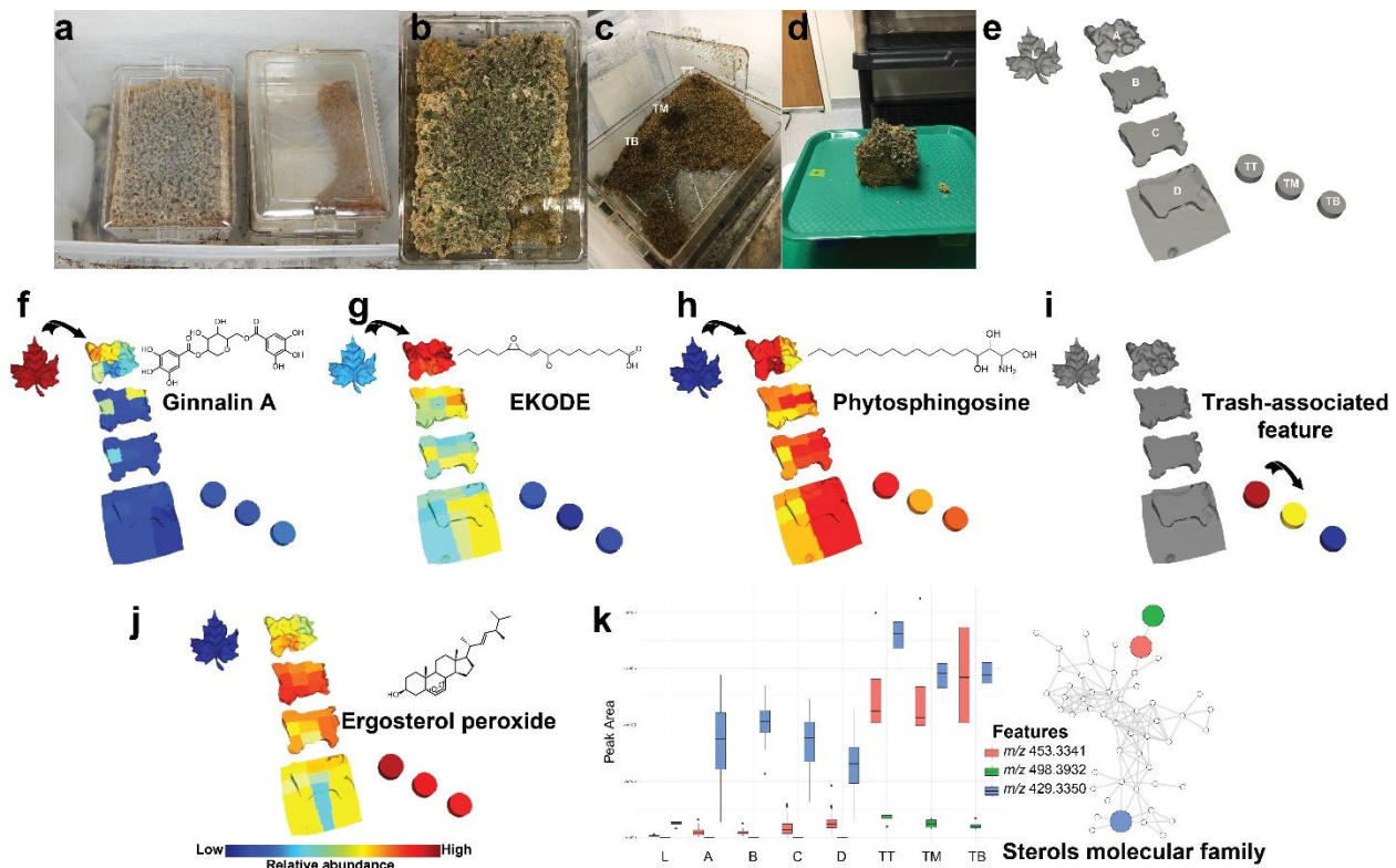
Fig. 1 | Spatial distribution of molecular signatures from A. texana fungus garden. a-d. Deconstruction of the Atta texana JKH000189 fungus garden: a. Plastic containers with an Atta texana fungus garden (left) and waste material removed by ants (right). Ants have free access to both chambers; b. This picture shows the location of a removed 10x10x10cm portion of the fungus garden (lower right corner). The green fragments at the top of the fungus garden are freshly incorporated maple leaves; c. Chamber containing the trash material removed from the fungus garden by the ants. Three sampling locations from the trash are highlighted as "TB", "TM", and "TT"; d. Removed 10x10x10cm fungus garden portion for consequent sample preparation for LC-MS/MS; e. 3D representation of deconstructed fungus garden portion, as shown in (d). On the left side, a representation of the maple leaves (L) placed in the outer colony box that ants cut and incorporate into the top of the fungus garden; layers of the fungus garden from top to bottom (A, B, C, and D) and at the right side of the figure, the representation of the three sample locations from the trash chamber, from top to bottom (TT, TM and TB); f-i. Spatial distribution of ginnalin A, detected as m/z 469.0971 (f), (E)-9-oxo-11-(3-pentyloxiran-2-yl)undec-10-enoic acid (trans-EKODE-(E)-Ib) detected as m/z 311.221 (g), phytosphingosine detected as m/z 318.2995 (h), unknown feature associated to the trash material detected as m/z 474.3783 (i); j-k. The abundance of features belonging to the molecular family of sterols were also detected at high intensity in the trash material, suggesting that these compounds accumulate in the trash material: j. Ergosterol peroxide detected as m/z 429.3350; k. Abundance of features associated with trash material belonging to the sterols molecular family (ergosterol peroxide, feature m/z 498.3932 and feature m/z 453.3341). The boxes represent the 25%, 50%, and 75% quantile and the whiskers extend \pm 1.5 times the interquartile range. The annotation of ergosterol peroxide from GNPS libraries (cosine score = 0.71) was confirmed using a reference standard (Supplementary Table S1), a level 1 match according to the 2007 metabolomics initiative, 32 while the m/z 498.3932 is consistent with a molecular formula of C_{32}H_{52}NO_3 (error 1.9 ppm) and belongs to the same molecular family - a level 3 match. 32 A detailed description of the sample preparation can be found in the Online methods. See online
