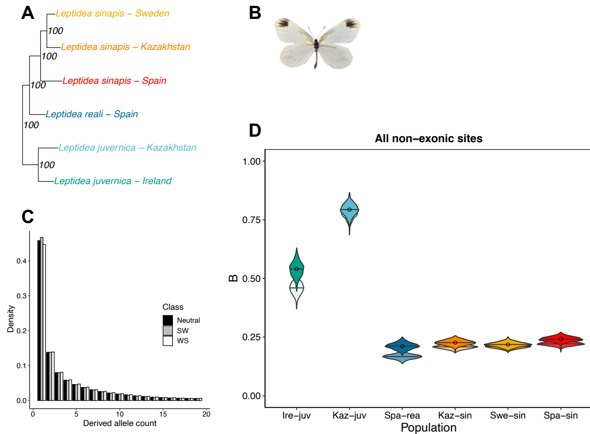
Figure 1. Leptidea butterflies show variation in the genome-wide strength of gBGC. A) Phylogeny of the six Leptidea populations included in this study. Node values represent support from 100 bootstrap replicates on sites. The phylogeny in A) is based on a subtree from a maximum-likelihood phylogeny used as a starting tree in Figure 1 of Talla et al. (2017). B) Mounted specimen of Leptidea sinapis . C) DAF spectra for polarized non-exonic SNPs of the Swedish L. sinapis population split in categories S→W (SW), W→S (WS) and GC-neutral. D) Estimates of the population-scaled coefficient of gBGC ( B = 4N_e b ). Circles represent point estimates from the original DAF spectra using model M1*, bars are mean values of B for the 1,000 bootstrap replicates of sites. Overlain and opaque violins are bootstrapped values for model M1* and underlain, transparent violins are estimates for model M1.
