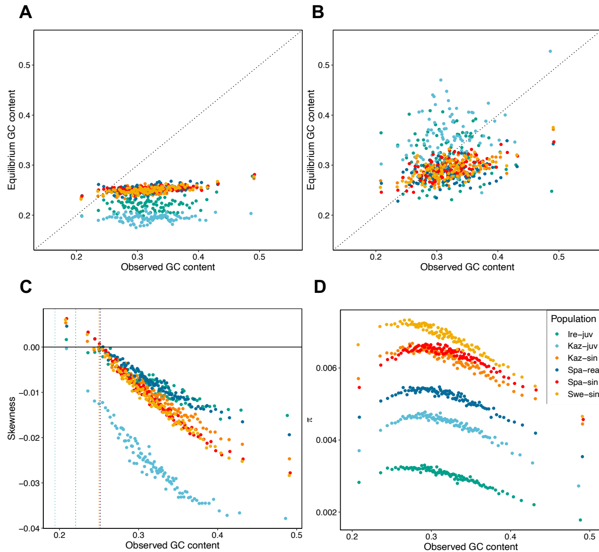
Figure 4. Observed GC content, equilibrium GC content and their association with \lambda , B and genetic diversity ( \pi ). A) Observed GC content compared to equilibrium GC content determined by mutation bias ( \lambda ) alone. B) Observed GC content compared to equilibrium GC content when accounting for gBGC. Dotted lines in (A) and (B) represent x = y . C) The skewness of the folded SFS shows the strong S \rightarrow W bias in the segregating variation which increases with observed GC content in the ancestral genome. Extrapolating from the distribution of skewness values onto the y=0 line serves as a validation of the estimated \lambda . Dotted vertical lines represent the GC equilibrium under mutation bias alone, 1/(1+\lambda) , for each population. D) The association between genetic diversity ( \pi ) and observed GC content. Points in all panels represent GC centiles.
