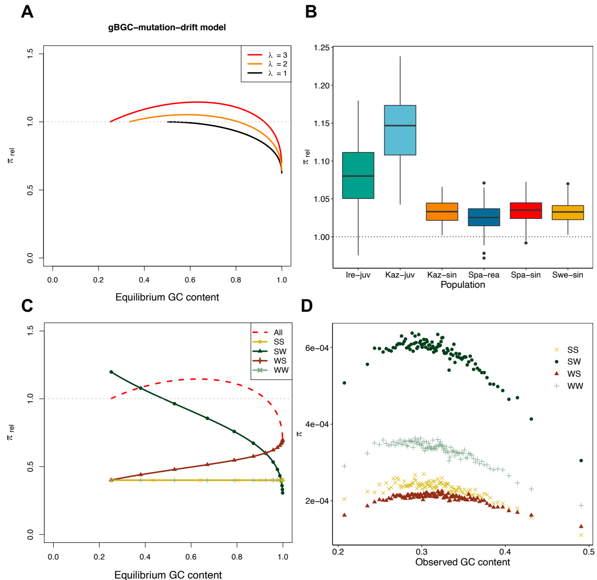
Figure 5: A model for genetic diversity under gBGC-mutation-drift equilibrium, predicted \pi_{rel} per population and \pi per mutation category. A) Genetic diversity relative to neutral ( B = 0 ) across equilibrium GC content determined by B and \lambda . Lines begin at B = 0 and end at B = 8 . The mutation bias is held constant. B) Genetic diversity values predicted from the gBGC-mutation-drift equilibrium model using output from the inference of gBGC. Most of the genome for each population have values of B and \lambda such that their relative strength boosts the long-term genetic diversity compared to B = 0 . The lower and upper limit of the box correspond to the first and third quartiles. Upper and lower whiskers extend from the top- and bottom box limits to the largest/smallest value at maximum 1.5 times the inter-quartile range. C) Components of the gBGC mutation drift model. Only results from \lambda = 3 are shown. The separate mutation categories were standardized by mutational opportunity while “All” was standardized as in A). The genetic diversity is here assumed to be equal for N \rightarrow N and W \rightarrow S mutations ( \theta_N / \theta_{WS} = 1 ). D) Genetic diversity in Swedish L. sinapis measured by average pairwise differences ( \pi ) across genomic GC content for all four mutation categories: S \rightarrow S (SS), S \rightarrow W (SW), W \rightarrow S (WS), W \rightarrow W (WW). The other populations are shown in Figure S3.
