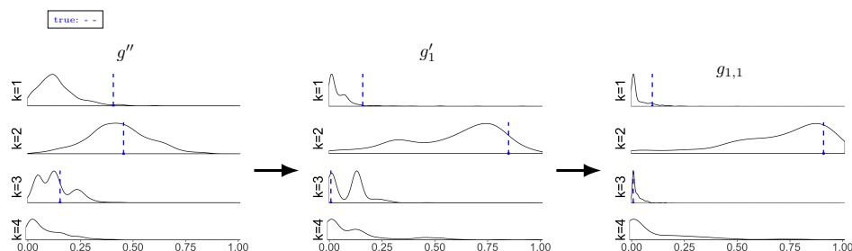
Fig 5: Marginal posterior density estimates for simulation data with N = 6 and N_i = 4 . The population-level subpopulation marginal distribution g'' slightly underestimates the fraction of subpopulation k = 1 and is accurate for the other subpopulations. The accuracy of the individual-level distribution g'_1 and the sample-level distribution g_{1,1} are more accurate in part because they are closer to the data in the model hierarchy.
