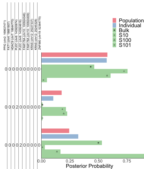
Fig 6: Posterior distribution plots for Patient 6 from Model hDP. Red bars show the population level distribution over subpopulations ( \hat{g}''|\mathcal{H}, \mathbf{x} ), blue bars show the individual level distribution ( \hat{g}'|\mathcal{H}, \mathbf{x} ), and green bars show the sample level distributions ( \hat{g}|\mathcal{H}, \mathbf{x} ), where \mathcal{H} = \{\mathbf{h}_k \mid \exists \hat{g}_{ijk} > 0.05, \text{ for } i = 6 \text{ and } j = 1, 2, 3, 4\} .
