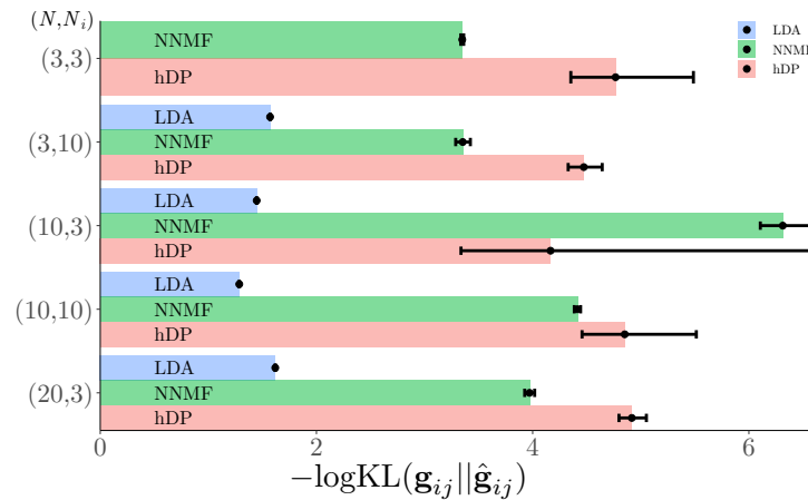
Fig 11: Comparisons among NNMF, LDA, and Model hDP. The KL divergence between the estimated sample-level posterior distribution over subpopulations and true distribution over subpopulations, KL(g_{ij} || \hat{g}_{ij}) , shows the model accuracy (higher -\log KL is better).
