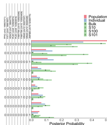
Fig 23: Posterior Distribution of Patient 5
