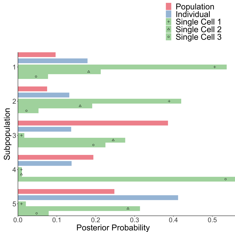
Fig 7: Posterior distribution plots for Patient 1 for Model hGP . Red bars show the population level distribution over subpopulations ( \hat{g}''|\mathcal{H}, \mathbf{x} ), blue bars show the individual level distribution ( \hat{g}'|\mathcal{H}, \mathbf{x} ), and green bars show the sample level distributions ( \hat{g}|\mathcal{H}, \mathbf{x} ).
