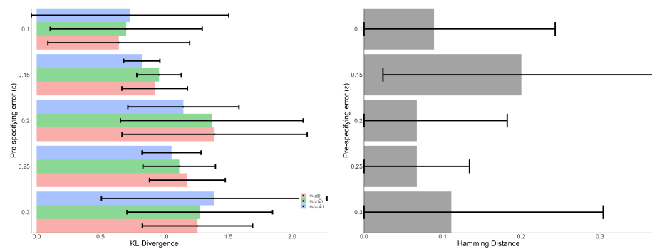
Fig 16: Sensitivity analysis varying \epsilon_{IA}^{(sc)} and \epsilon_{la}^{(sc)} . (left) Average KL divergence between true subpopulation distribution and estimated. (right) Average distance between true subpopulation genotype and estimated.
