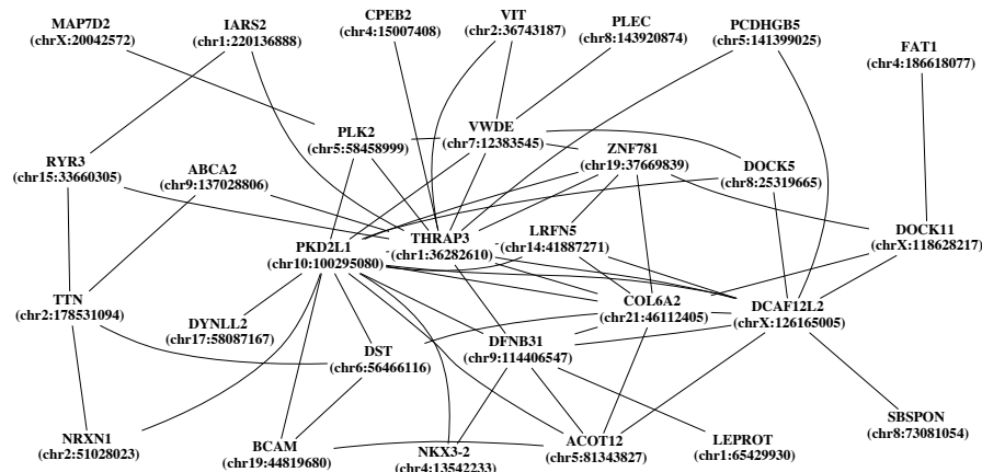
Fig 30: Inferred mutation co-occurrence network across Patient 5 from Model hGP .
