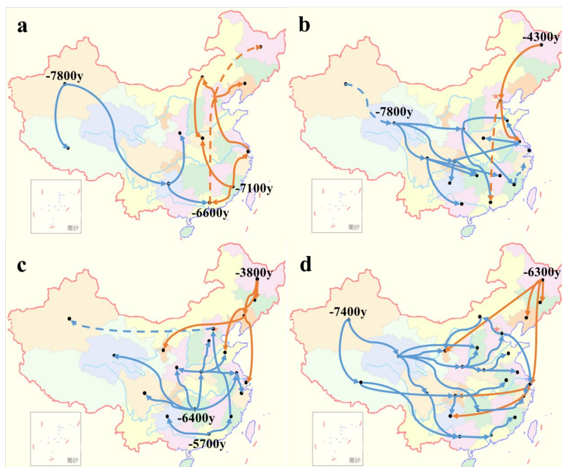
Figure 4. Potential propagation routes of four sub-lineages in China. Shown are routes for L2.2 (a), L4.2 (b), L4.4 (c) and L4.5 (d). The dotted line indicates that the distance is long and the evidence maybe weak (possibly due to a lack of strains). Blue lines indicate older transmission routes, while orange lines indicate more recent transmission routes.
