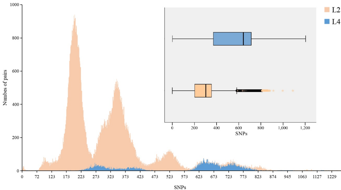
Figure 6. Number of pairwise differences between Mtb strains for lineage 2 and lineage 4. The alignment of 217 human-adapted Mtb clinical strains published previously (Comas et al., 2013) was used to calculate pairwise differences of global strains.
