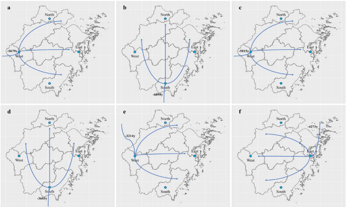
Figure 5. Potential propagation routes of six sub-lineages in Zhejiang Province. Shown are L2.1 (a), L2.2 (b), L2.3 (c), L4.2 (d), L4.4 (e) and L4.5 (f). The curves without starting points indicate the directions and years of the strains entering Zhejiang Province from other regions.
