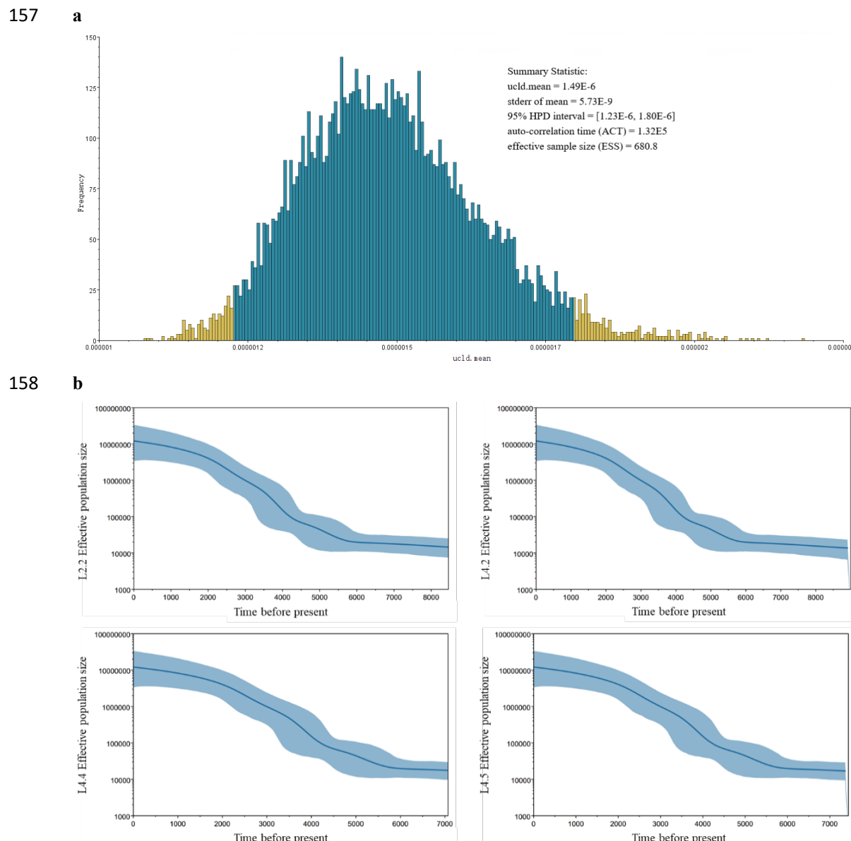
159 Figure 3. Mutation rates and changes in sub-lineage diversity over time. (a) The mutation rate was 160 estimated using BEAST. (b) Bayesian skyline plots indicating changes in the diversity of four 161 sub-lineages over time. Shaded areas show the 95% HPD (high posterior density) intervals for the 162 population-size estimations.
