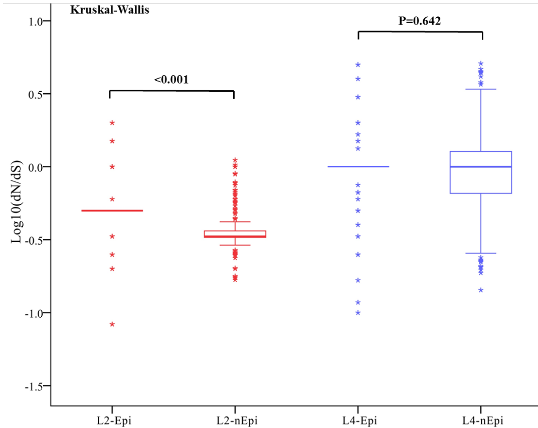
Figure 8. Pairwise ratios for the rates of nonsynonymous to synonymous substitutions (dN/dS) in lineage 2 and 4 isolates, assessing epitope and non-epitope regions of T cell antigens.
