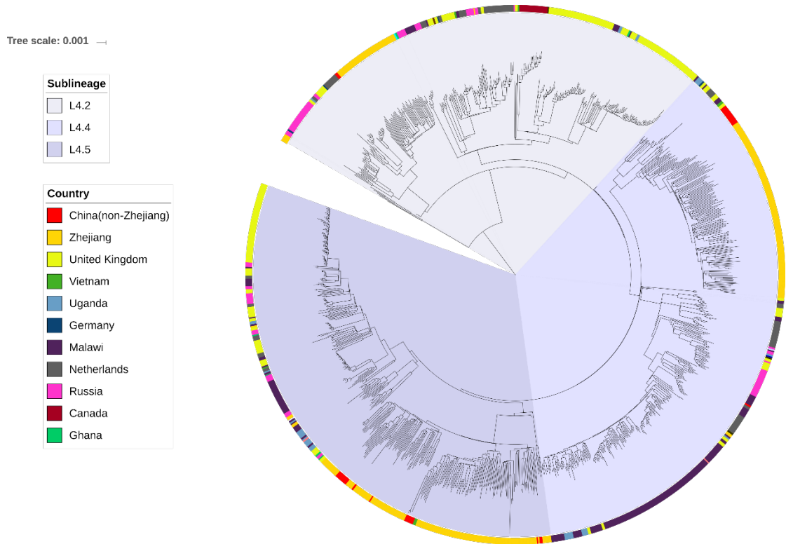
Figure 2. Bayesian phylogeny of the Zhejiang M. tuberculosis isolates and 1154 globally distributed publically available genomes for (a) lineage 2 and (b) lineage 4. Scale bar indicates the
