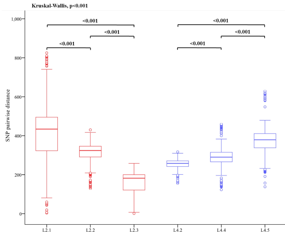
Figure 7. Box plots of pairwise genetic distances (number of polymorphisms) for each sub-lineage.
