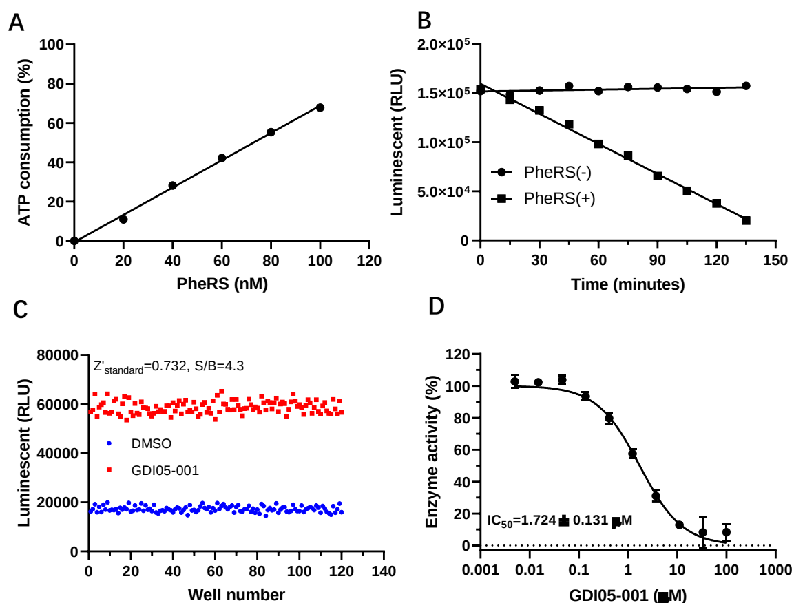
Figure S4. Development of HTS using ATP consumption assay (Kinase-Glo) and HTS optimization. A, Linearity of ATP consumption with respect to Mtb PheRS concentration. B, Linearity with respect to time with or without Mtb PheRS. C, Z' factor of HTS by using ATP consumption assay. D, IC 50 of tool compound GDI05-001 against Mtb PheRS.
