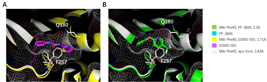
Figure S8. F257 and Q180 rotation creates a deeper amino acid pocket of Mtb PheRS. The side chain rotation of F257 and Q180 contributes to a much deeper amino acid pocket in the complexed structure than that in apo form structure. The amino acid pockets are indicated by mesh. A. Superposition of apo and GDI05-001 complexed structures. B. Apo and PF-3845 complexed structures.
