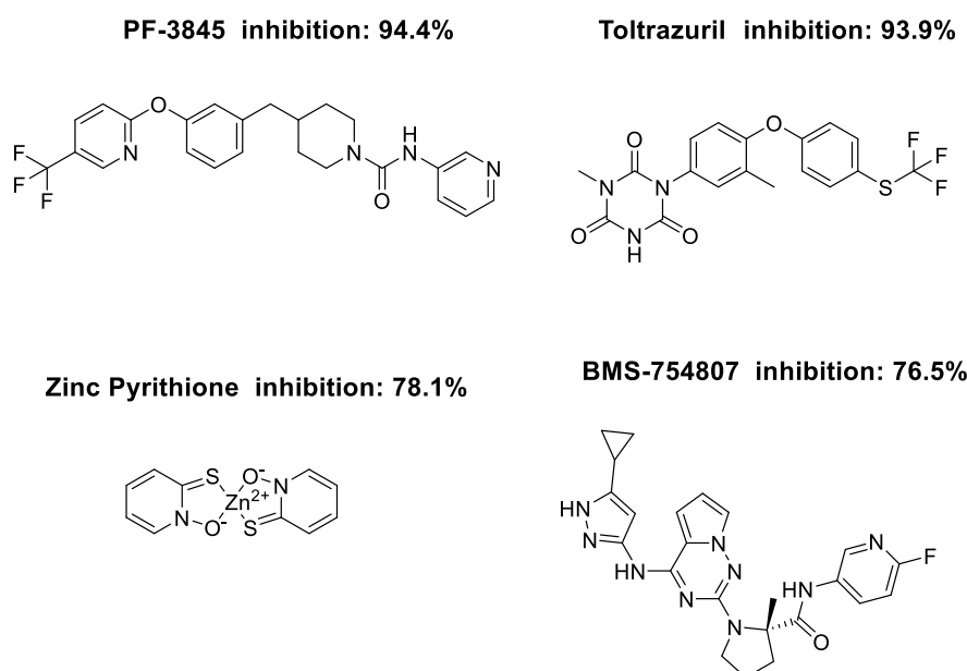
Figure S5. Primary hits of the Mtb PheRS HTS.
