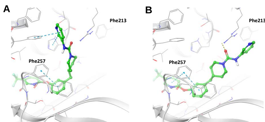
Figure S10. Two putative binding conformations of PF-3845 generated by Orbital docking platform (Accutar Biotech). A, PF-3845 is modelled into the substrate Phe and additional pockets. B, PF-3845 is modelled into both Phe and ATP binding pockets.
