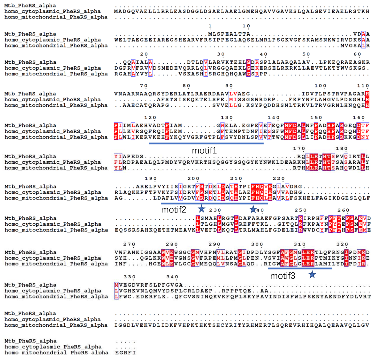
Figure S2. Alignment of PheRS α subunits and identification of motifs. Motif 1 forms part of the dimer interface and helps orient the motif 2 and 3 active site loops. Motif 2 participates in the binding of ATP, amino acid substrate, and the acceptor end of tRNA, while motif 3 interacts with ATP substrate. The highly conserved arginine and phenylalanine of motif 2, and the arginine of motif 3 marked by asterisks have catalytic roles.
