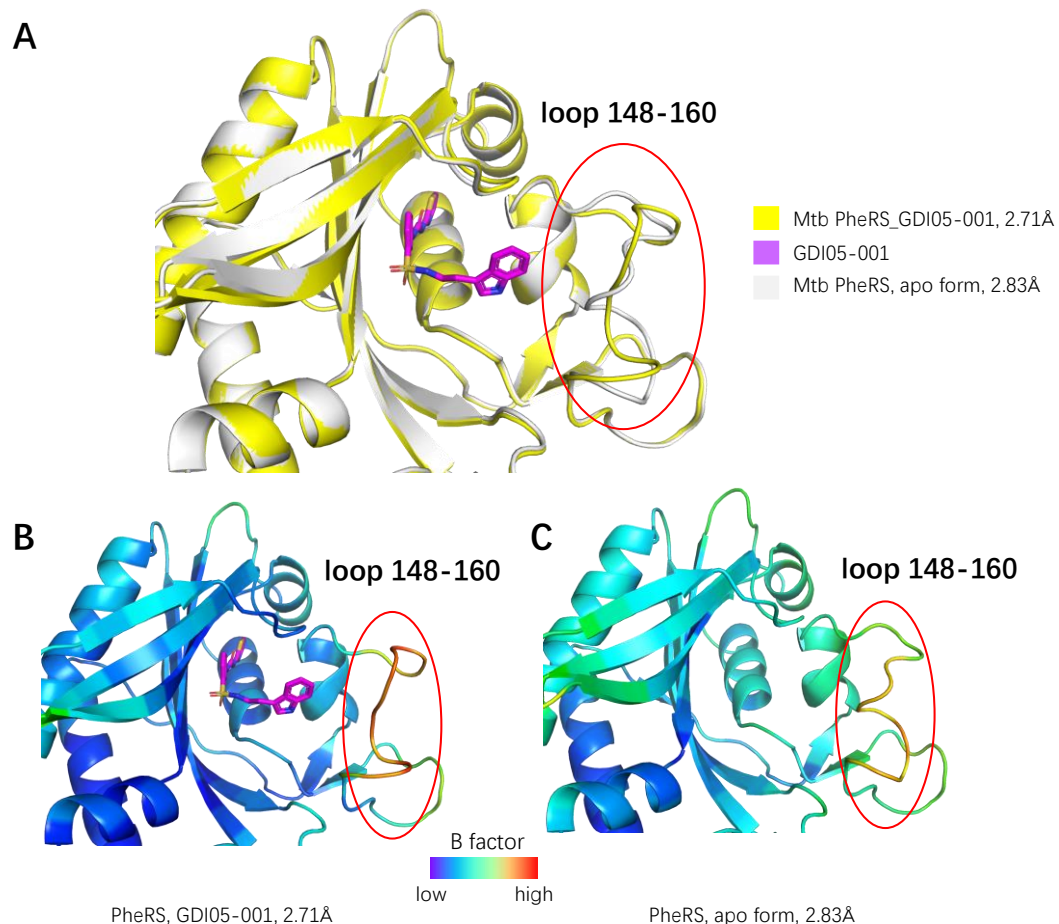
Figure S9. GDI05-001 binding leads to conformational change of the loop 148-160 of α subunit of Mtb PheRS. A, structure comparison of the α subunits of Mtb PheRS apo form and in complex with GDI05-001. B-C, structure colored by B factors. Compared to apo structure, the loop 148-160 of the GDI05-001 bound structure undergoes a conformational change, which has much higher B factors than the apo structure.
