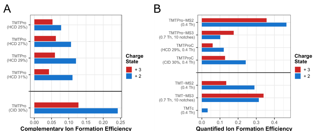
Figure 3. Optimization of TMTPProC ion formation and comparison with ion formation efficiencies in alternative multiplexed proteomics methods. A) Evaluation of various fragmentation methods for TMTPProC ion formation. HeLa peptides were labelled with TMTPPro and subjected to various fragmentation modalities. Shown are the median proportions of MS1 ion flux from the precursor that was converted into complementary ions. CID fragmentation produced about two-fold higher signal in the complementary ion cluster than HCD fragmentation. B) Comparison of TMTPProC ion efficiencies with alternative methods. HeLa peptides labeled with TMTPPro or TMT were subjected to various quantification methods. For each, we calculate the median fraction of precursor ion flux that is converted into the relevant ion used for quantification. TMTPPro improves complementary ion formation efficiency to the same level as both reporter ion-based quantification methods.
