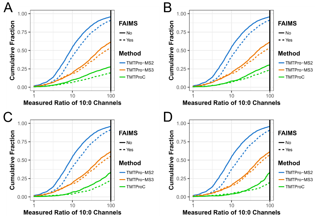
Figure S5. Evaluating ratio distortion for TMTProC and alternative multiplexed quantification strategies with various S:N cutoffs.
