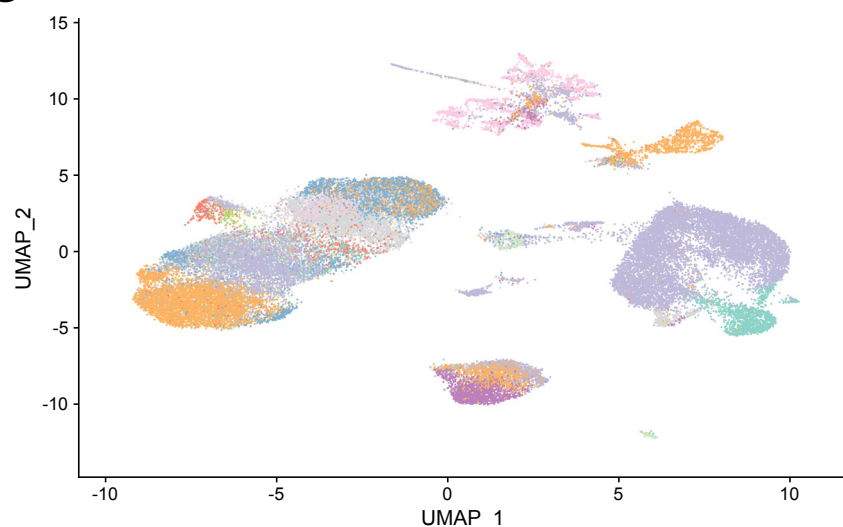
Figure 7: Supervised mapping of immune perturbations
