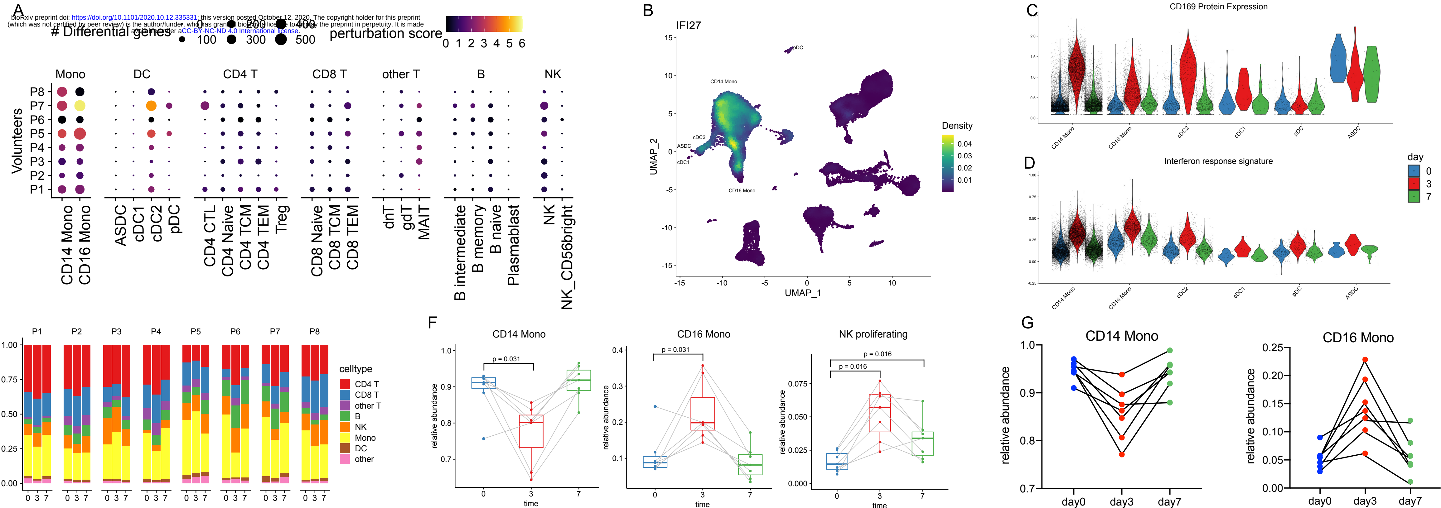
Figure 6: Identifying cell-type specific responses to vaccination
