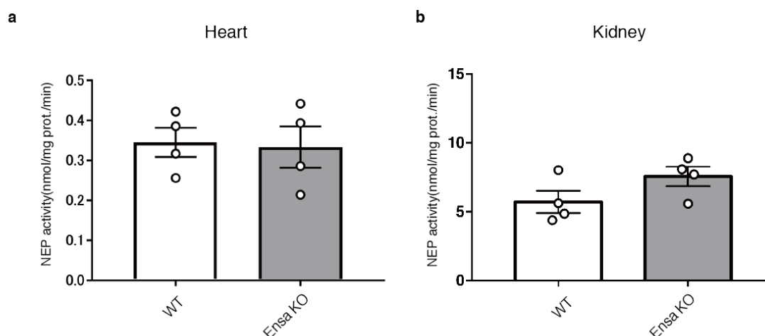
Extended data Fig.5 Cardiac and renal NEP activity in Ensa KO mice. a , NEP activity in membrane fractions from cardiac tissue of 3-month-old WT and Ensa KO mice (n = 4 for each group). b , NEP activity in the membrane fractions from kidney tissue of 3-month-old WT and Ensa KO mice (n = 4 for each group). Results are expressed as the mean \pm SEM.
