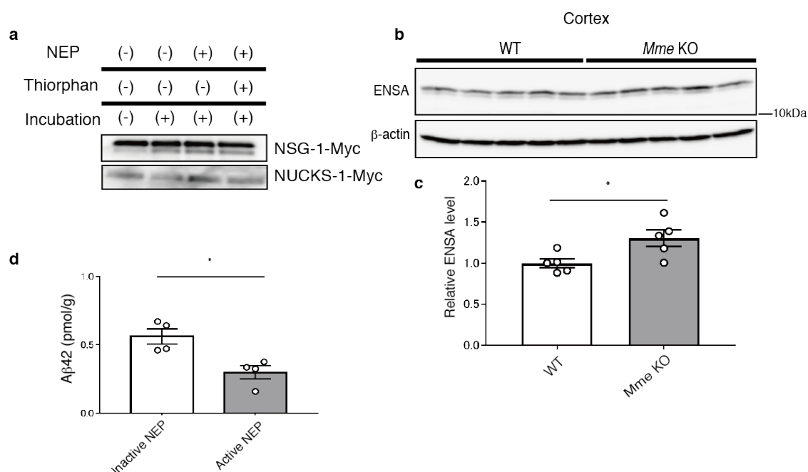
Extended data Fig.6 Identification of ENSA as a substrate for NEP. a , Immunoblotting of NSG-1 or NUCKS-1 incubated with or without NEP and thiorphan for 24 hours at 37°C. The specific band is detected by Myc-tag antibody. b , Immunoblotting of ENSA in cortices from 6-month-old WT and Mme KO mice. Values indicated in the graph show the intensity of ENSA bands normalized to that of β-actin (n = 5 for each group). c , Aβ 42 ELISA of Tris-HCl-buffered saline-soluble fractions containing 1% Triton-X from hippocampi of WT mice after overexpression of active or inactive mutant NEP by the SFV gene expression system (n = 4 for each group). Results are expressed as the mean ± SEM. * P < 0.05 (Student's t -test).
