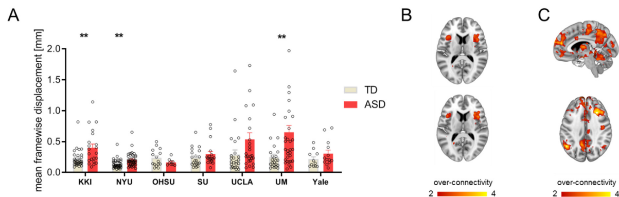
Supplementary Figure S2. Insular hyperconnectivity in children with ASD is identifiable after strict control of in scanner head motion. A) In scanner head motion during fMRI acquisition as measured with mean frame-wise displacement. Mean frame-wise displacement is higher in brain scans of children with ASD acquired at KKI ( t = 3.21 , p = 0.002 ), NYU ( t = 3.29 , p = 0.001 ) and UM ( t = 2.86 , p = 0.006 ). **p < 0.01 as compared to site-matched TDs. B) Upon removal of volumes showing frame-wise displacement higher than 0.2 mm, long-range connectivity mapping confirmed bilateral hyperconnectivity in anterior insular regions in children with ASD. C) Seed based mapping carried out on the same scrubbed data corroborated long-range hyperconnectivity between anterior insular areas and cortico-striatal targets.
