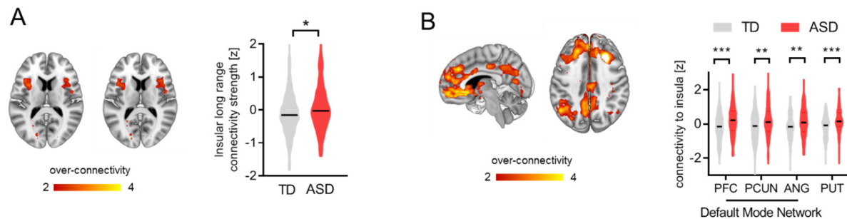
Supplementary Figure S1. Insular hyperconnectivity in children with ASD is not driven by a single collecting site. A) By excluding all scans acquired at Stanford University (i.e. the participating institution with the most prominent case-control hyperconnectivity [Cohen's d = 0.81 ]), long-range rsfMRI connectivity mapping confirmed the presence of bilateral functional connectivity of anterior insular cortices in children with ASD vs TDs ( t = 2.39 , p = 0.017 ). B) Similarly, seed based mapping on the same scans corroborated long-range hyperconnectivity between insular and cortico-striatal targets, suggesting that long range hyperconnectivity in ASD is not primarily attributable to time-series acquired at Stanford University. PFC, prefrontal cortex; PCUN, precuneus; ANG, angular gyrus; PUT, putamen. *p < 0.05 , **p < 0.01 , ***p < 0.001 .
