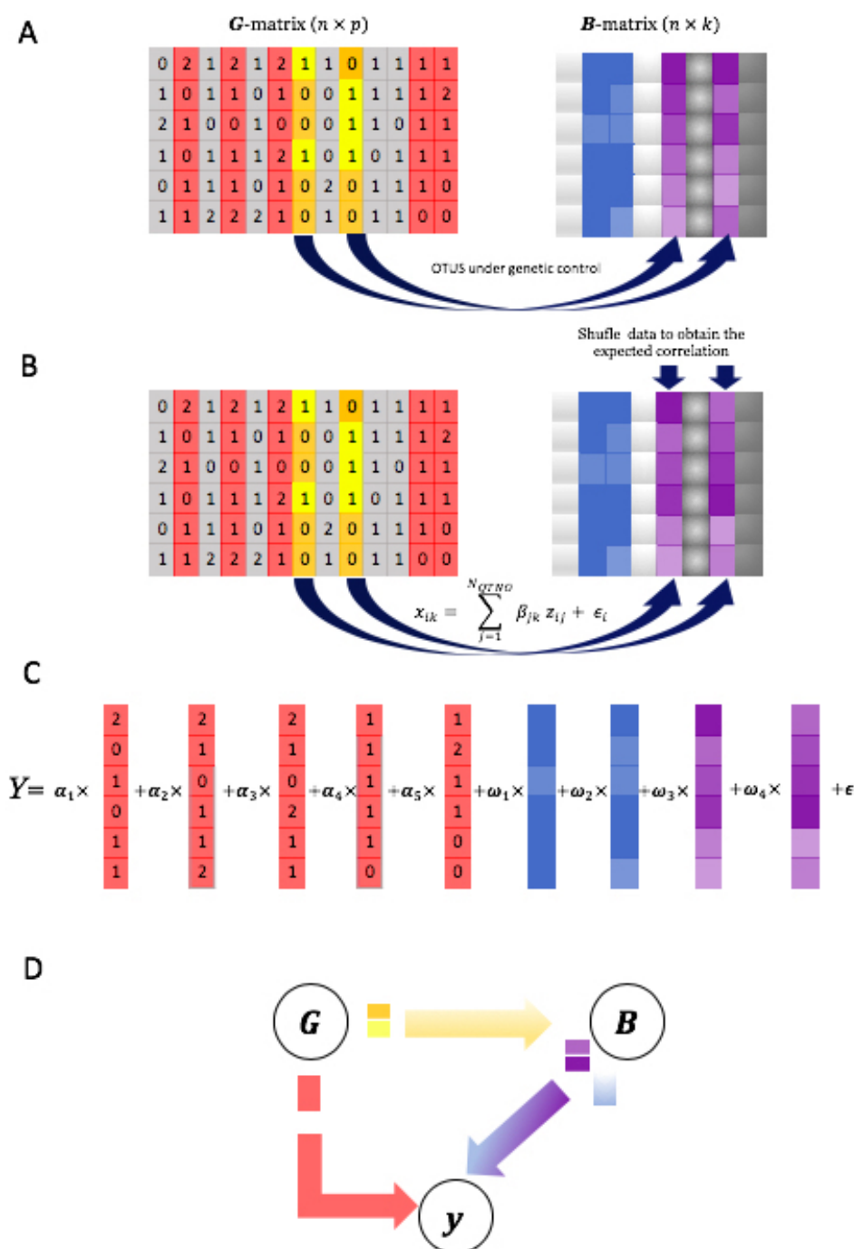
Fig 2: Simulation scheme for the Recursive scenario, i.e., the most complex scenario (Fig 1). A) Real input data comprises p genotypes ( G matrix) and k taxa abundances ( B matrix). SNPs in grey are neutral, those in red act directly on the phenotype y , and those in yellow/orange influence some OTU abundances (marked in magenta color in B matrix); abundances in blue are not genetically controlled. B) Given simulated effects, a genotypic value controlling the abundances is obtained via Eqn. 2. To fulfill the required heritability, abundances in magenta are reordered; high abundances (represented by a darker color) are associated with genotype '1' just to simplify visualization. A single SNP is shown as causative for each of the two OTUs but there is no limit in practice. C) The phenotype is simulated by adding the genome and the microbiome contributions plus a residual. D) The general causal diagram is shown.
