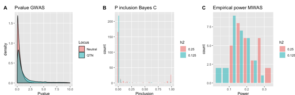
Fig 6: A) Distribution of -\log_{10} P-values of a GWAS of abundances on SNP data; B) Probability of inclusion in the Bayes Cgb model of causative OTUs for the two levels of microbiability considered. C) Power of identifying a causative OTU computed as the probability of exceeding the 95% threshold of the empirical distribution of P-values in an MWAS for the Recursive scenario.
