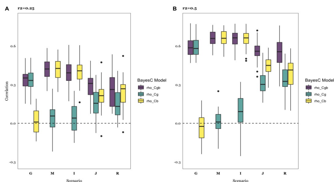
Fig 3. Predictive accuracy, computed as correlation between predicted and observed phenotypes across causal scenarios (Fig 1), for each of the Bayes C models: Cgb considers microbiome and genome; Cg includes genome data only, and Cb includes microbiome data only. A: r^2 = 0.25 ; B: r^2 = 0.50 . Details of scenarios are in Table 1: G, Genome; M, Microbiome; I, Indirect; J, Joint; R, Recursive. Results are average of 30 replicates per case.
