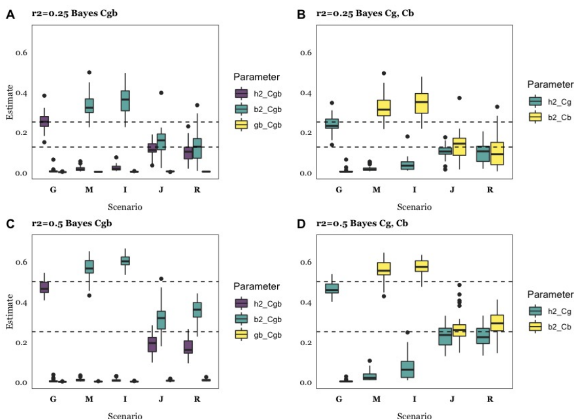
Fig 5: Estimates of heritability ( h^2 ), microbiability ( b^2 ), and correlation between genome and microbiome ( gb ) for each of the three Bayes C analysis models: Cgb includes microbiome and genome in the model (left panels); Cg includes genome only, and Cb includes microbiome data only (right panels). Upper rows correspond to r^2 = 0.25 and lower rows to r^2 = 0.50 . Details of simulation scenarios are in Table 1: G, Genome; M, Microbiome; I, Indirect; J, Joint; R, Recursive. Horizontal dashed lines indicate true h^2 or b^2 parameter values (0.125, 0.25, 0.5 depending on the scenario and on r^2 ). Results are average of 30 replicates. A: r^2=0.25 , Bayes Cgb estimates ( h^2 , b^2 and gb ); B: r^2 = 0.25 , Bayes Cg ( h^2 ) and Cb ( b^2 ) estimates; C: r^2 = 0.50 , Bayes Cgb estimates; D: r^2 = 0.50 , Bayes Cg and Cb estimates. Data are average of 30 replicates per case.
