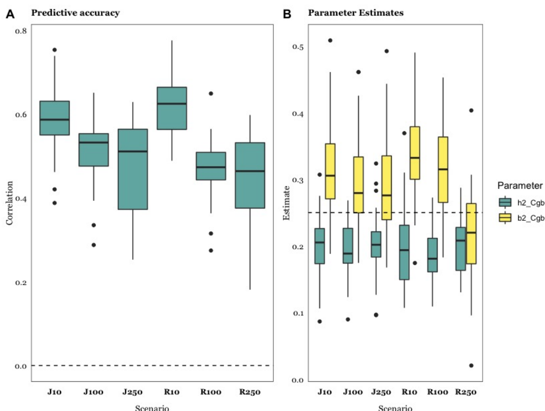
Fig 4. Effect of varying number of causative OTUs, r^2 = 0.5 . A: Predictive accuracy, computed as correlation between predicted and observed phenotypes, using Bayes Cgb. B: Heritability and microbiability estimates using Bayes Cgb. Details of scenarios are in Table 2 and diagrams in Fig 1: Jx, Joint scenario; Rx, Recursive scenario, with x being the number of causative OTUs ( x = 10, 100, 250 ), half of them under genetic control. Results shown are the average of 30 replicates.
