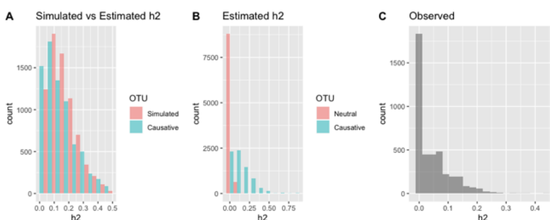
Fig 7: A: ‘True’ (simulated) and GBLUP estimated distribution of abundance heritabilities for causative OTUs in the Recursive scenario. B: GBLUP estimated distribution of abundance heritabilities for neutral and causative OTUs in the Recursive scenario. C: Actual distribution of OTU abundance heritabilities reported by Difford et al.[4].
