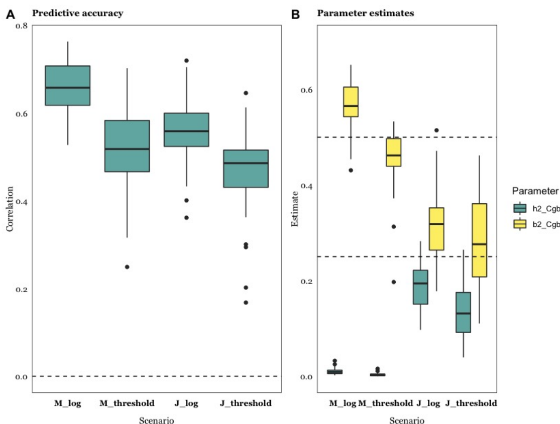
Fig 8. Comparison of multiplicative (log) and threshold Microbiome (M) and Joint (J) scenarios ( r^2 = 0.5 ). A: Predictive accuracy, computed as correlation between predicted and observed phenotypes, using Bayes Cgb. B: Heritability ( h^2 ) and microbiability ( b^2 ) estimates using Bayes Cgb. Results are average of 30 replicates. Scenarios M and J as specified in Table 1; the log transformation results are shown for completeness and are the same as in Figs 3 and 5. Data are average of 30 replicates.
