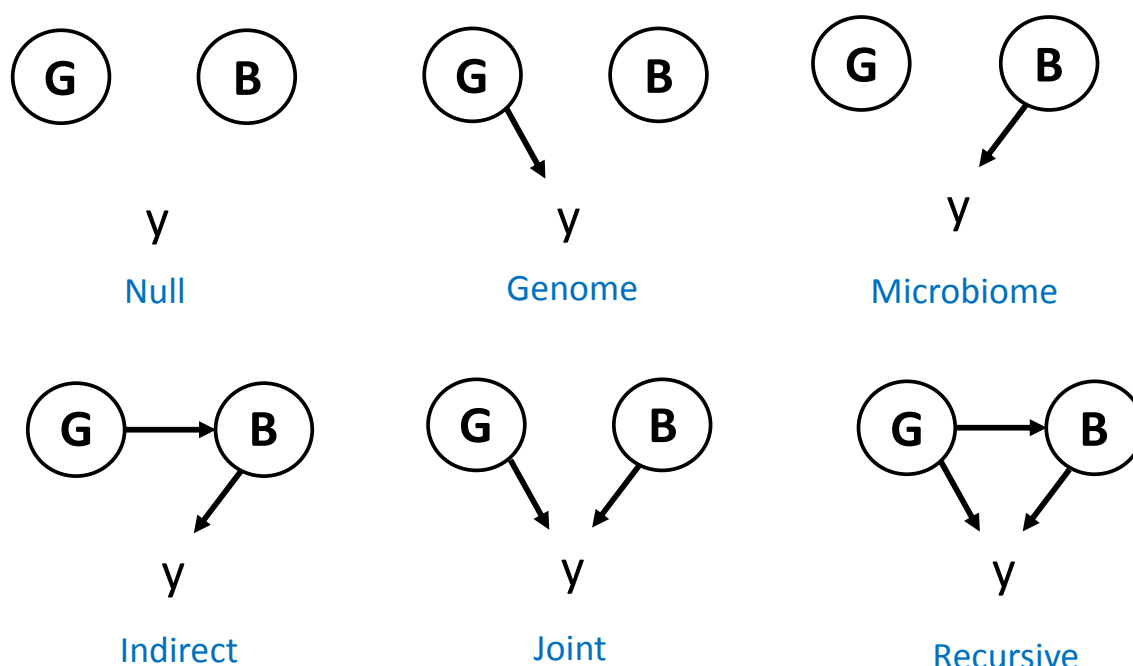
Fig 1. Representation of the scenarios evaluated: G , genome, typically comprises marker data; B , microbiome; y , phenotype of interest; arrows indicate causality. An arrow from G to y indicates that there is a subset of G elements (causative SNPs) that influence y ; an arrow from G to B indicates there exists a subset of G that influences a subset of abundances in B which, in turn, may also influence y . An arrow departing from B indicates there is a subset of microbial abundances (the causative abundances) that influence y . The SNPs affecting B need not necessarily be the same SNPs affecting y directly in the Recursive scenario. Note B can contain one or more sets of abundances such as archaea and bacteria communities, or different time or site sampling points. Without loss in generality, we assume B is a single community.
