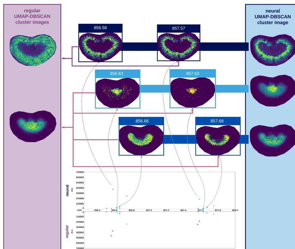
Figure 6. Ion image clustering results of the mouse kidney dataset. The Figure shows a zoom-in of the mean spectrum, highlighting an isotopic distribution, and marked associated ion images. Cluster assignments in the mean spectrum are shown for each m/z bin, for the neural (top) and regular (bottom) UMAP-DBSCAN pipelines. The purple (regular) and blue (neural) panels show the mean images for the clusters to which the marked ion images are assigned. Similar to the lymph node dataset, the neural pipeline shows better cluster assignments than the regular pipeline, with mean cluster images that show a closer match to the assigned cluster images.
