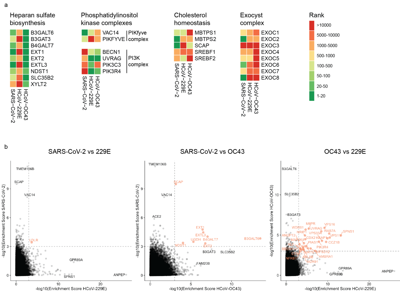
Extended Data Figure 2: Comparison of CRISPR screens reveals common and distinct host factors across SARS-CoV-2, 229E and OC43. (a) CRISPR screen ranking of genes, which are part of specific cellular pathway or complexes, across the three CRISPR screens. (b) Pairwise comparisons of gene enrichments between two CRISPR screens. Dotted lines indicate -\log_{10}(\text{Enrichment score}) > 3 . Genes that scored above the threshold in both screens, are highlighted in red.
