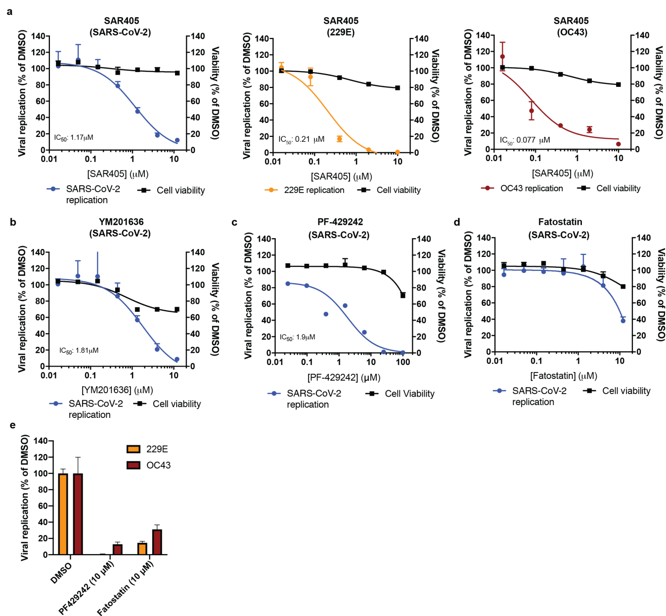
Figure 4: Pharmacological inhibition of phosphatidylinositol kinase complexes and cellular cholesterol homeostasis decreases infection with SARS-CoV-2 and common cold coronaviruses. (a) SAR405 dose-response curves for SARS-CoV-2, HCoV-229E and HCoV-OC43 replication in Huh7.5.1 cells and for cell viability of drug treated cells. (b-d) Dose-response curves of the effect of (b) YM201636, (c) PF-429242, (d) Fatostatin on SARS-CoV-2 replication and cell viability.
