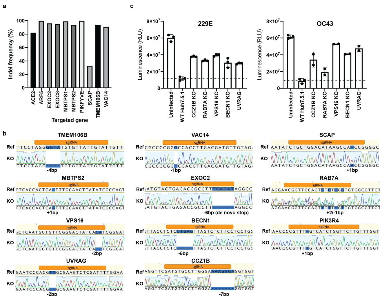
Extended Data Figure 4: Knockout of host factor genes reduces coronavirus infection and virus-induced cell death. (a) Indel frequency of RNP-edited polyclonal A549-ACE2 KO cells. Targeted loci were PCR-amplified, Sanger-sequenced and analyzed using Inference of CRISPR Edits (ICE) analysis 65 . (b) Genotyping of clonal Huh7.5.1. Targeted loci were PCR-amplified, Sanger-sequenced and aligned to WT reference sequence. Frameshifts are highlighted in blue. (c) Cell viability measurement of 229E or OC43 infected WT and KO Huh7.5.1 cells. Cells were infected with 229E (moi=0.05) or OC43 (moi=3) and viability was determined 8 dpi using Cell Titer Glo.
