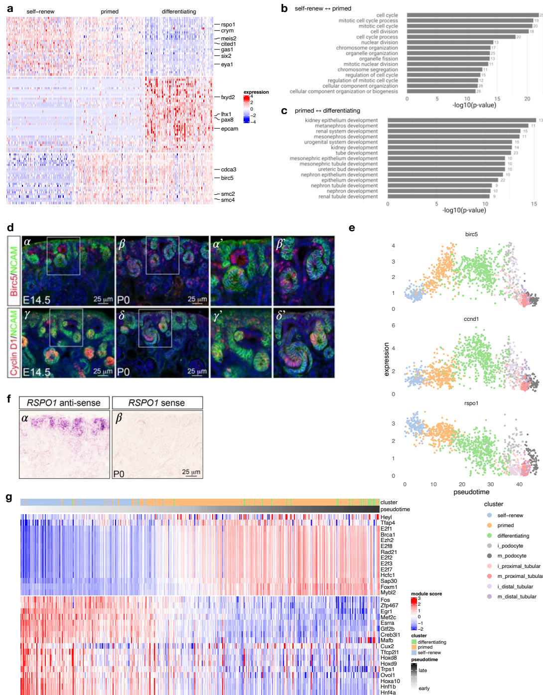
Figure 3: Transcriptional signatures of self-renewing, primed and differentiating nephron progenitor cells. Panel (a) shows differentially expressed genes on a heatmap of 100 random cells for each of the “self-renew”, “primed” and differentiating clusters, with key genes annotated on the right. Panels (b) and (c) show the 20 most-enriched Gene Ontology terms for genes differentially expressed between self-renewing and primed NP
