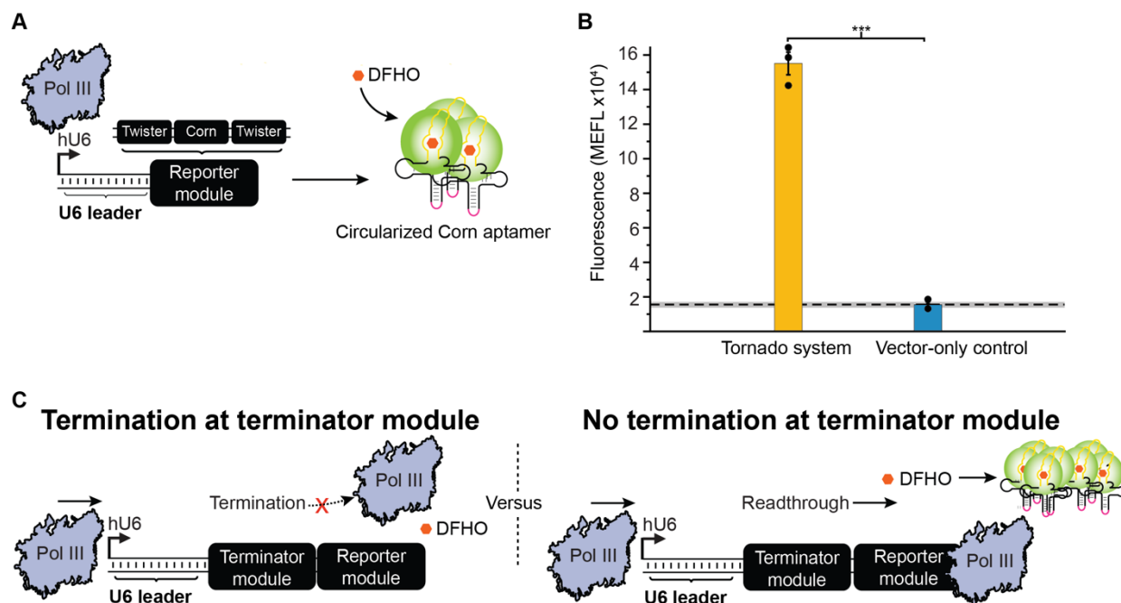
Figure 1: Development of an assay for measuring Pol III termination in human cells. A) Schematic overview of the construct design of the Tornado system [26]. A human U6 promoter drives Pol III transcription of a 'Reporter module', comprising a Corn aptamer (yellow line) which is embedded within a tRNA scaffold and flanked by two twister self-cleaving ribozymes. The ribozymes' self-cleavage results in a 5' hydroxyl and a 3' end consisting of a 2',3'-cyclic phosphate which is recognized and ligated (pink line) by the endogenous protein RtcB, increasing its stability. Ribozyme self-cleavage and ligation leaves a circularized Corn aptamer that is stabilized by the tRNA scaffold. When DFHO is bound to the Corn aptamer, this dye becomes fluorescent. B) Tornado enables quantification of Pol III transcription in cellulo . Colored bars represent the average of 3 biological replicates (circles). The dashed line indicates the average signal from the vector-only (negative) control cells, while the grey horizontal
