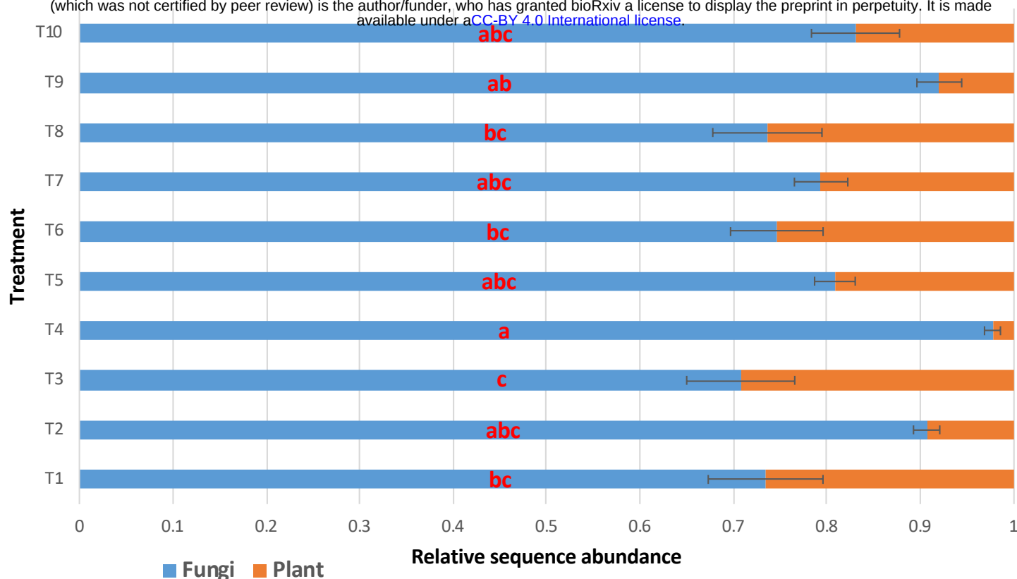
Fig. 3. Relative sequence abundance of Fungi to plants by treatment (Brignant soil). Letters on the bars indicate significant groupings as determined by Tukey's HSD post hoc test and error bars show standard error of the mean.
