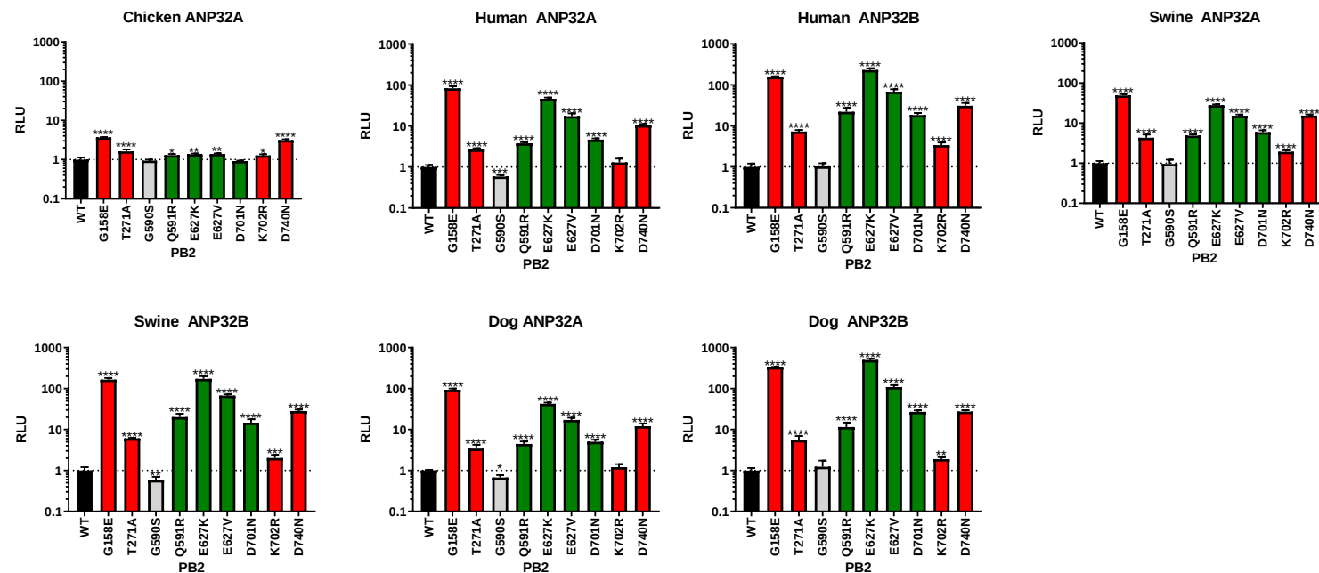
Figure S1. Extended version of Figure 2.
