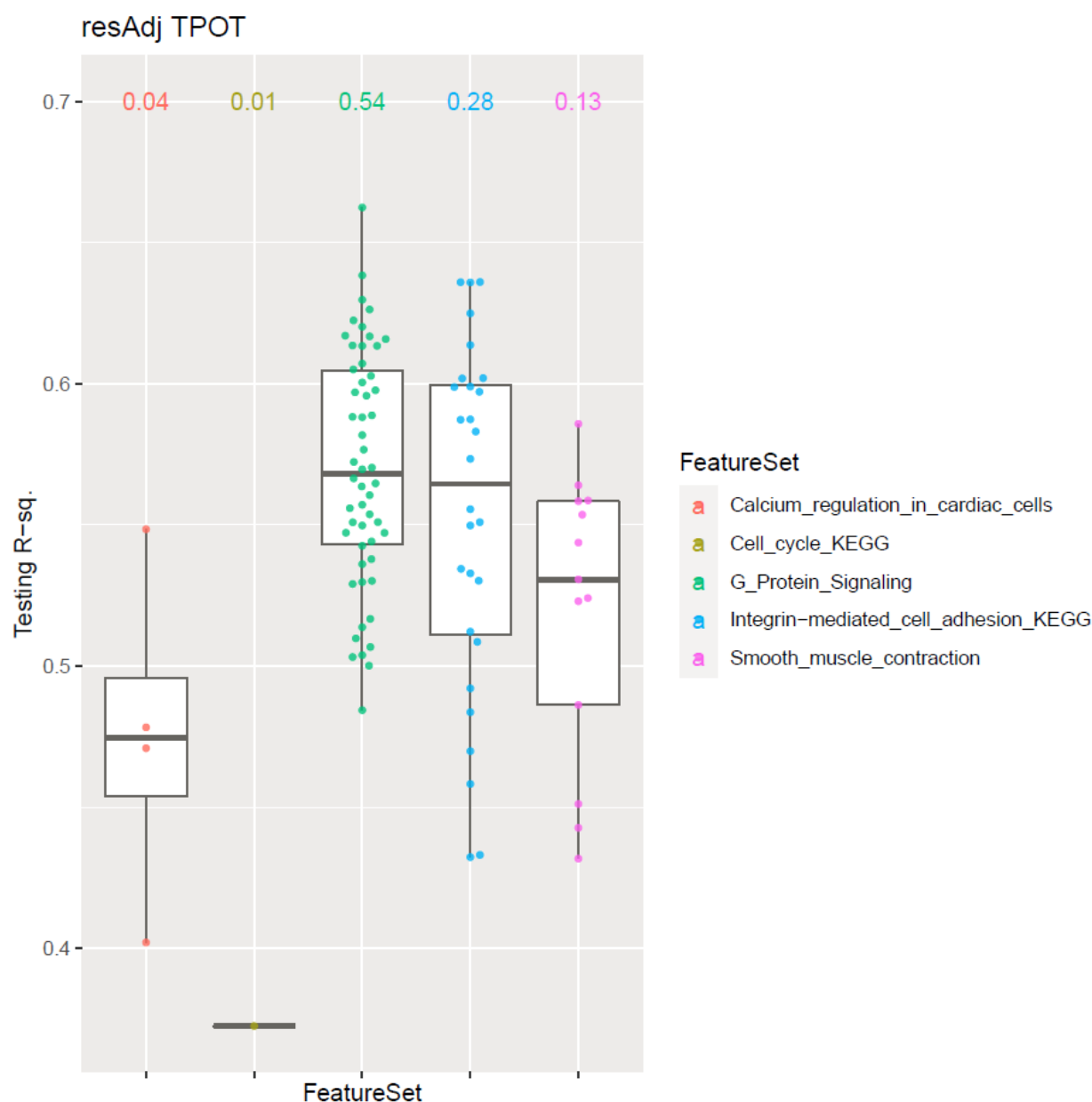
Figure 2. Boxplots for the results of 100 runs of resAdj TPOT on the TG-GATEs data set. Each point corresponds to one run, where the x-coordinate indicates the pathway (Feature Set) selected in the optimal pipeline for that run and the y-coordinate indicates the R^2 on the held-out Testing dataset.
