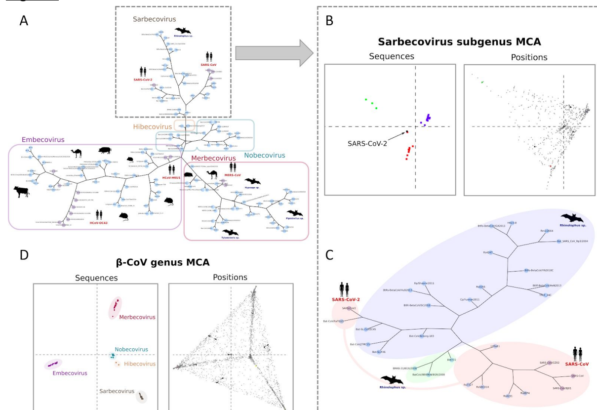
Figure 1. A) Phylogenetic tree obtained for the complete \beta -CoV spike protein family. S3Det subfamilies are highlighted by rectangles and reflect the phylogenetic classification of Betacoronavirus into five subgenera. B) Results of the S3Det MCA analysis showing the subfamily segregation and associated amino acid positions obtained for the Sarbecovirus subgroup. C) Phylogenetic tree obtained for the Sarbecovirus subgroup. S3Det clusters are highlighted by red, green and blue silhouettes. Both SARS-CoV-2 and RaTG13 are clustered together with SARS-CoV and other members of Sarbecovirus clade 1. D) Results of the S3Det MCA analysis showing the subfamily segregation and associated amino acid positions obtained for the full \beta -CoV family. Phylogenetic trees were built using PhyML (28). Nodes representing spike protein sequences from human pathogenic CoVs are colored in purple. Host species are shown for some of the nodes as dark silhouettes.
