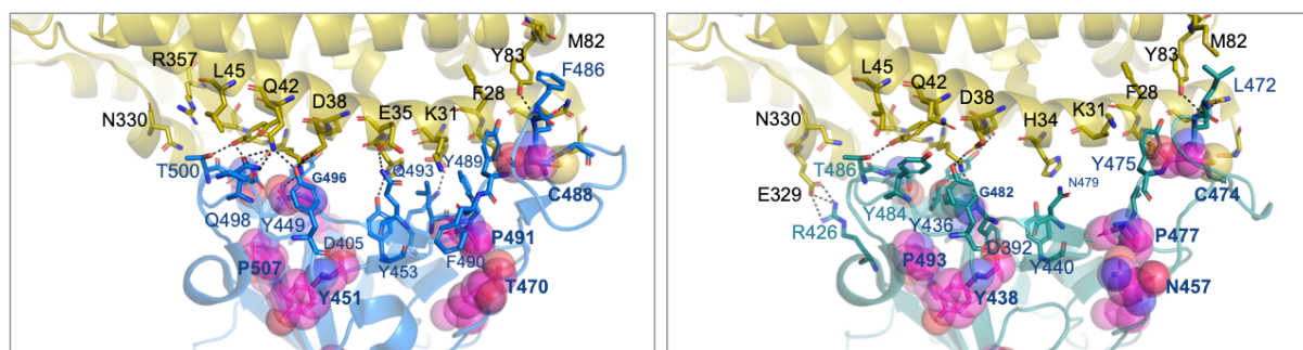
Figure 3. 3D structure of the spike protein from SARS-CoV-2 (blue; PDB ID: 6LZG) and SARS-CoV (green; PDB ID: 2AJF) in complex with the human ACE2 cell receptor (yellow). Amino acid residues at the interface are shown as sticks. Intermolecular contacts are shown as dashed black lines. SDPs are highlighted as spheres.
