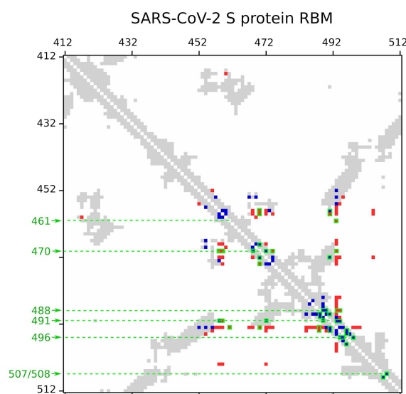
Figure 5. Contact map (8Å distance cutoff, any atom) over the RBM of the SARS-CoV-2 spike protein. MI-APC contact predictions (among top 500 scores) are shown in blue (true positives) and in red (false positives). SDPs are highlighted in green.
