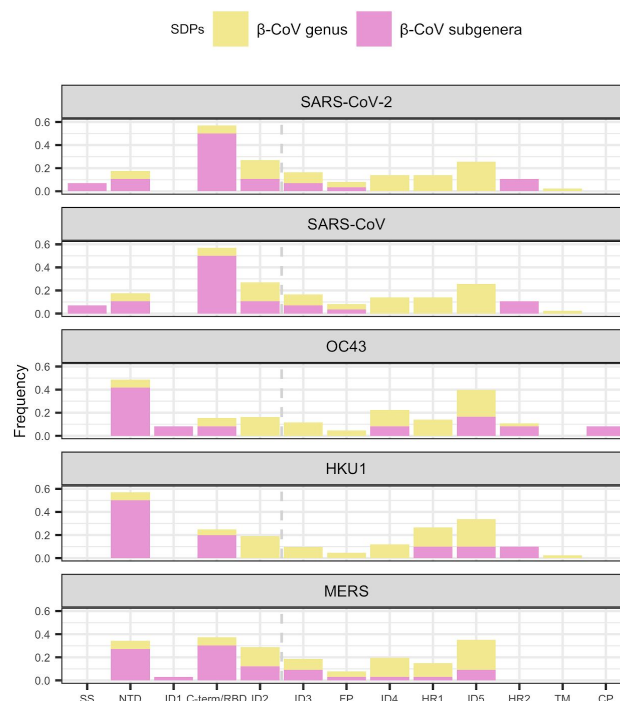
Figure 2. Frequency distribution of SDPs across different domains of the spike sequence from five human pathogenic \beta -CoVs. Protein domains are denoted as follows: SS, signal sequence; NTD, N-terminal domain; RBD, receptor binding domain; FP, fusion peptide; HR1, heptad repeat 1; HR2, heptad repeat 2. Interdomain regions are denoted by ID followed by an integer according to the order in which they appear in the sequence. Dashed vertical lines denote S1/S2 subunits boundaries.
