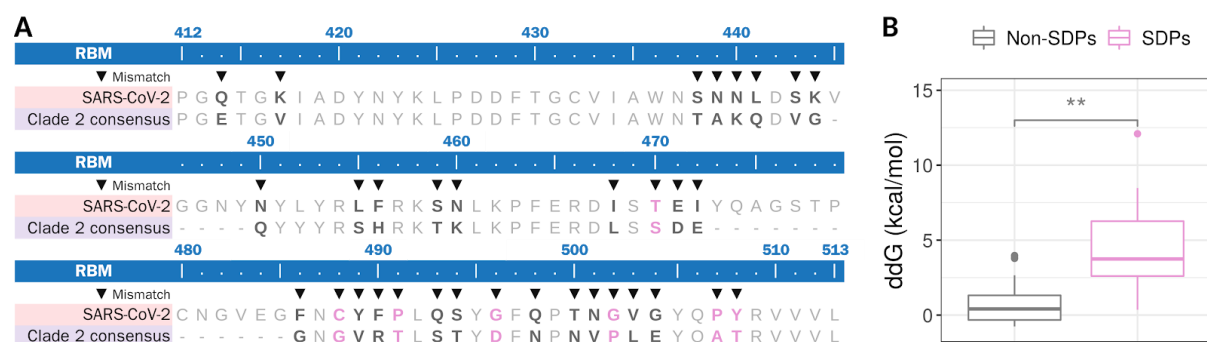
Figure 4. A) Pairwise sequence alignment of SARS-CoV-2 RBM and consensus sequence of Sarbecovirus clade 2. Black triangles indicate amino acid mismatches. SDP positions are depicted as pink letters. B) Boxplot distributions of \Delta\Delta G values resulting from mutating SDPs and non-SDPs using FoldX (PDB ID: 6LZG). Significant differences were computed using a Wilcoxon unpaired two-sample test ( p -value < 0.01).
